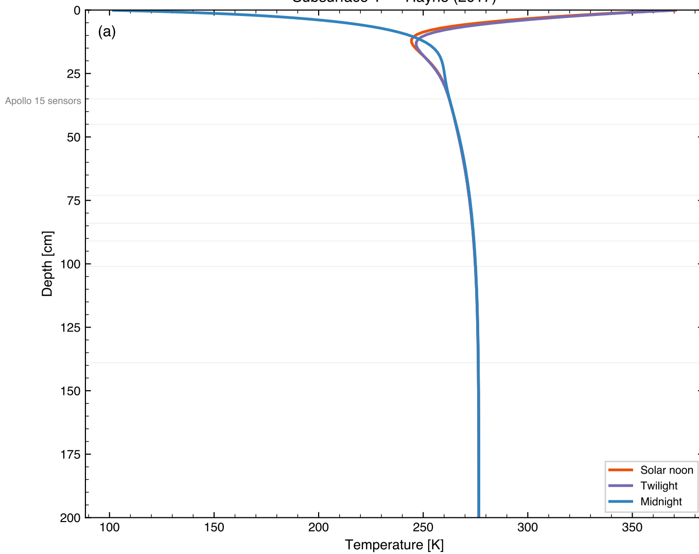
Subsurface T — Hayne (2017)
