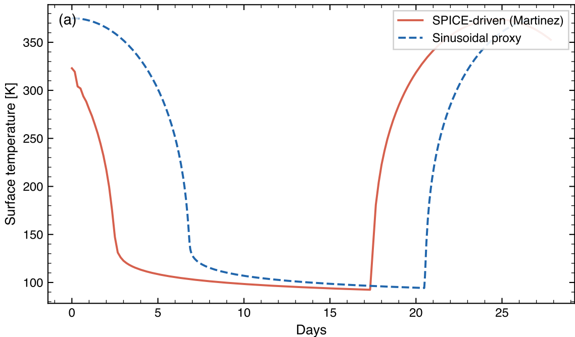
Surface T at 26.13°N — SPICE vs sinusoidal proxy
