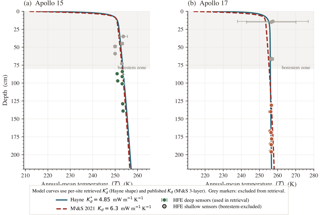
Figure 10. Annual-mean subsurface temperature profiles: Hayne retrieved K_d^* vs. Martínez & Siegler (2021) published K_d , at both sites. Solid teal: Hayne et al. (2017) model run with the per-site retrieved conductivity ( K_{d,A15}^* = 4.85 , K_{d,A17}^* = 11.23 \text{ mW m}^{-1} \text{ K}^{-1} ). Dashed red: M&S 2021 3-layer profile with its published K_d^{\text{disc}} = 6.3 \text{ mW m}^{-1} \text{ K}^{-1} (fixed at both sites). Coloured markers are HFE stability-window means for sensors below 80 cm (deep, used in retrieval); grey markers are the borestem-affected shallow sensors (excluded). The Hayne retrieval reproduces the deep gradient to near-zero bias at both sites (Table 2); the M&S profile sits between the two retrieved Hayne values and therefore over-predicts the warm A15 gradient and under-predicts the warm A17 gradient.
