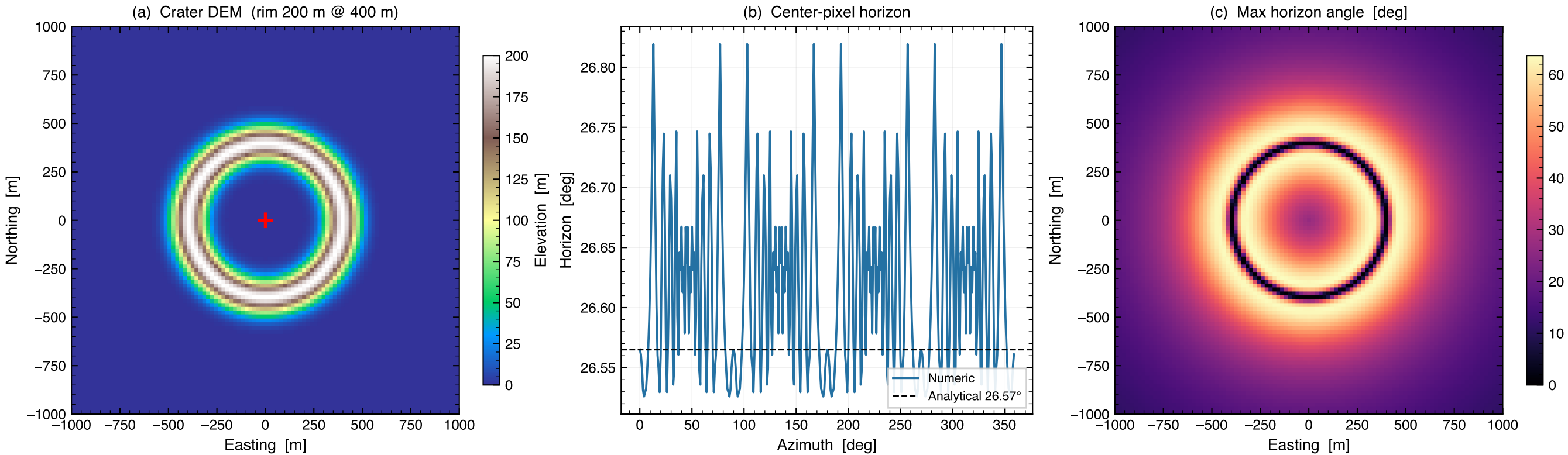
Fig 10 — Horizon tracer regression on a synthetic crater (PASS, RMS = 0.091^\circ )
