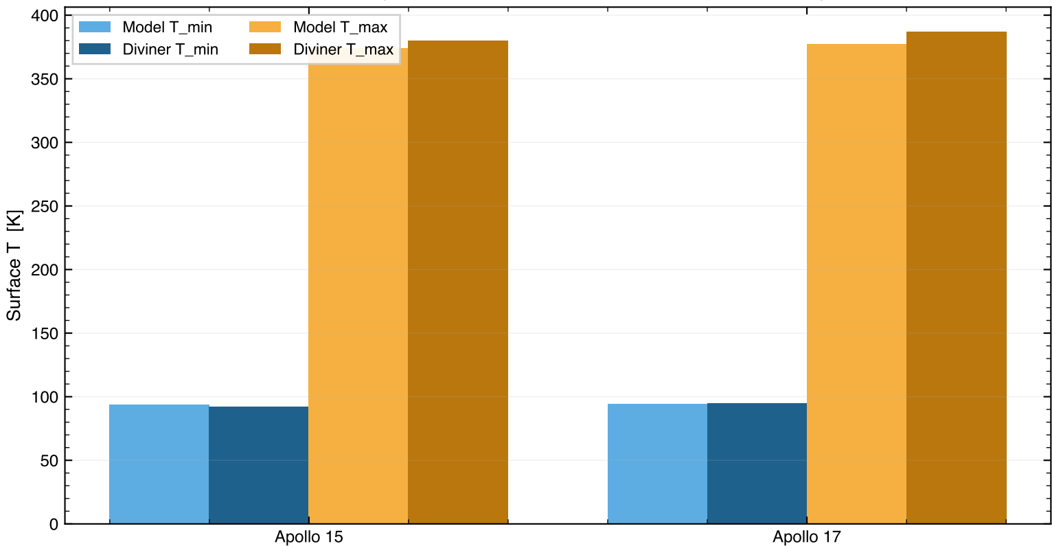
Fig 13 — Modelled vs Diviner-reported surface T extremes (Vasavada+2012 Fig 7, lat-band typical values; Diviner abs cal \pm 10 K, Paige+2010)
