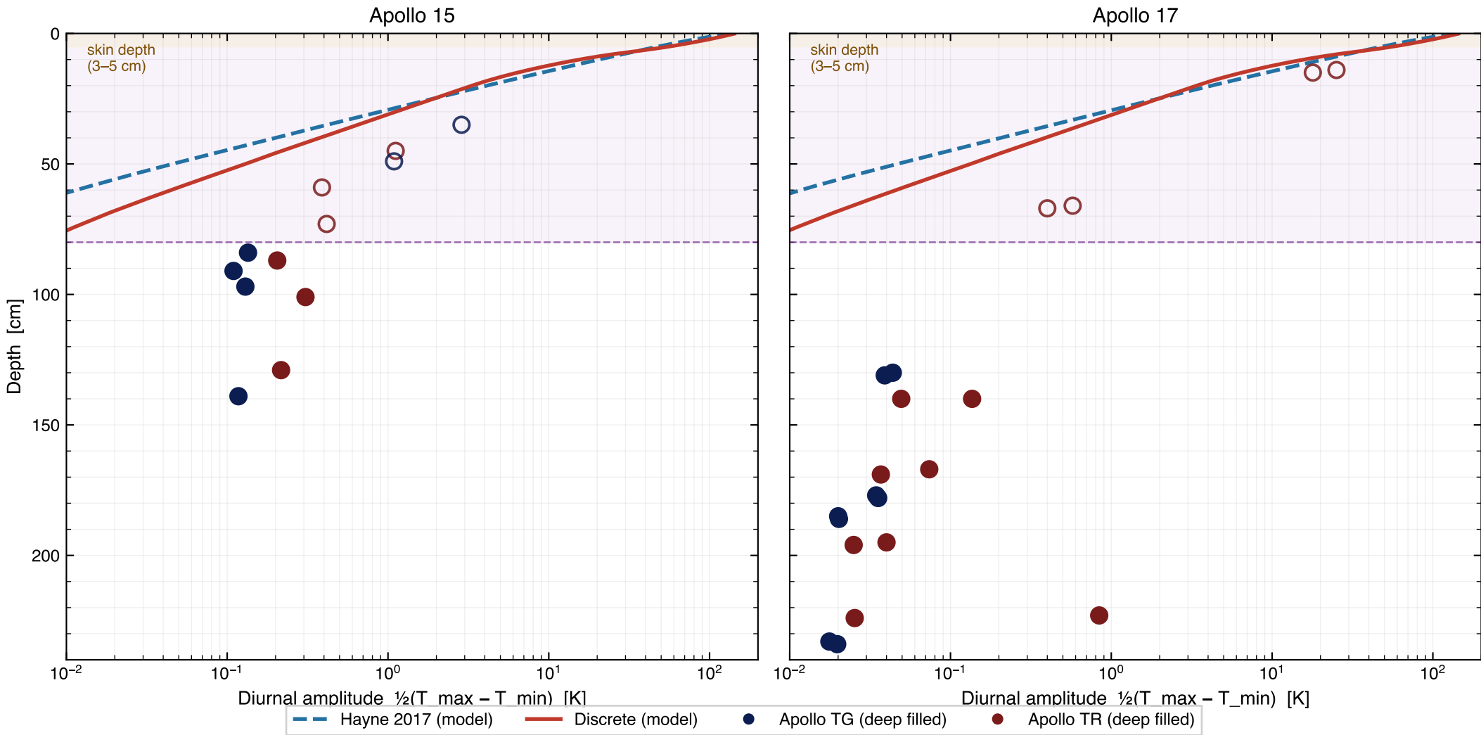
Fig 7 — Diurnal amplitude vs depth (skin-depth diagnostic; borestem heat-short produces the > 1 K tail at 30–60 cm)
