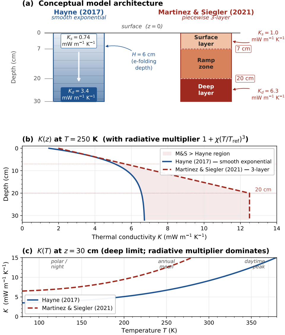
Figure 1. Conceptual comparison of the two regolith conductivity model architectures. (a) Physical layer structure: the Hayne et al. (2017) profile (blue) transitions continuously from a surface value K_s = 0.74 \text{ mW m}^{-1} \text{ K}^{-1} to a deep value K_d = 3.4 \text{ mW m}^{-1} \text{ K}^{-1} via an exponential with H = 6 \text{ cm} ; the Martínez and Siegler (2021) 3-layer profile (red) has a uniform surface layer ( K_s = 1.0 \text{ mW m}^{-1} \text{ K}^{-1} , 0–7 cm), a linear ramp zone (7–20 cm), and a uniform deep layer ( K_d = 6.3 \text{ mW m}^{-1} \text{ K}^{-1} , below 20 cm). (b) The corresponding K(z) profiles evaluated at T = 250 \text{ K} including the radiative multiplier 1 + \chi(T/T_{\text{ref}})^3 ; the shaded region is where the Martínez and Siegler (2021) conductivity exceeds the Hayne et al. (2017) value. The factor-of- \sim 2 difference in K_d is the dominant control on the deep-gradient discrepancy in Table 1.
