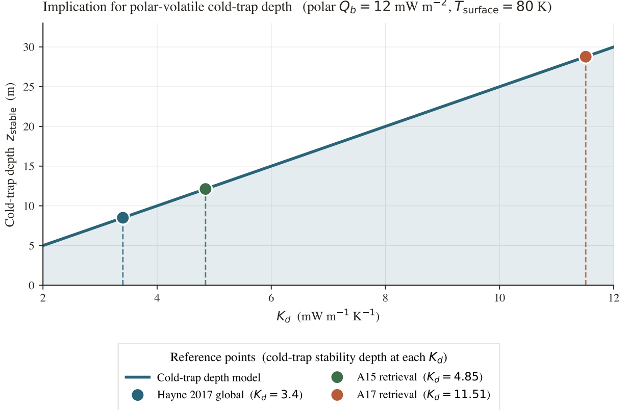
Figure 8. Implication for polar volatile cold-trap depth. Indicative cold-trap depth z_{\text{stable}} at which buried water ice is thermally stable on geological timescales (a Schorghofer and Aharonson 2005-style estimate at fixed polar surface temperature and basal heat flux), as a function of K_d . The factor-of- \sim 3 change in K_d between the global value of Hayne et al. (2017) and the A17 retrieval translates into a factor-of- \sim 3 change in z_{\text{stable}} .
