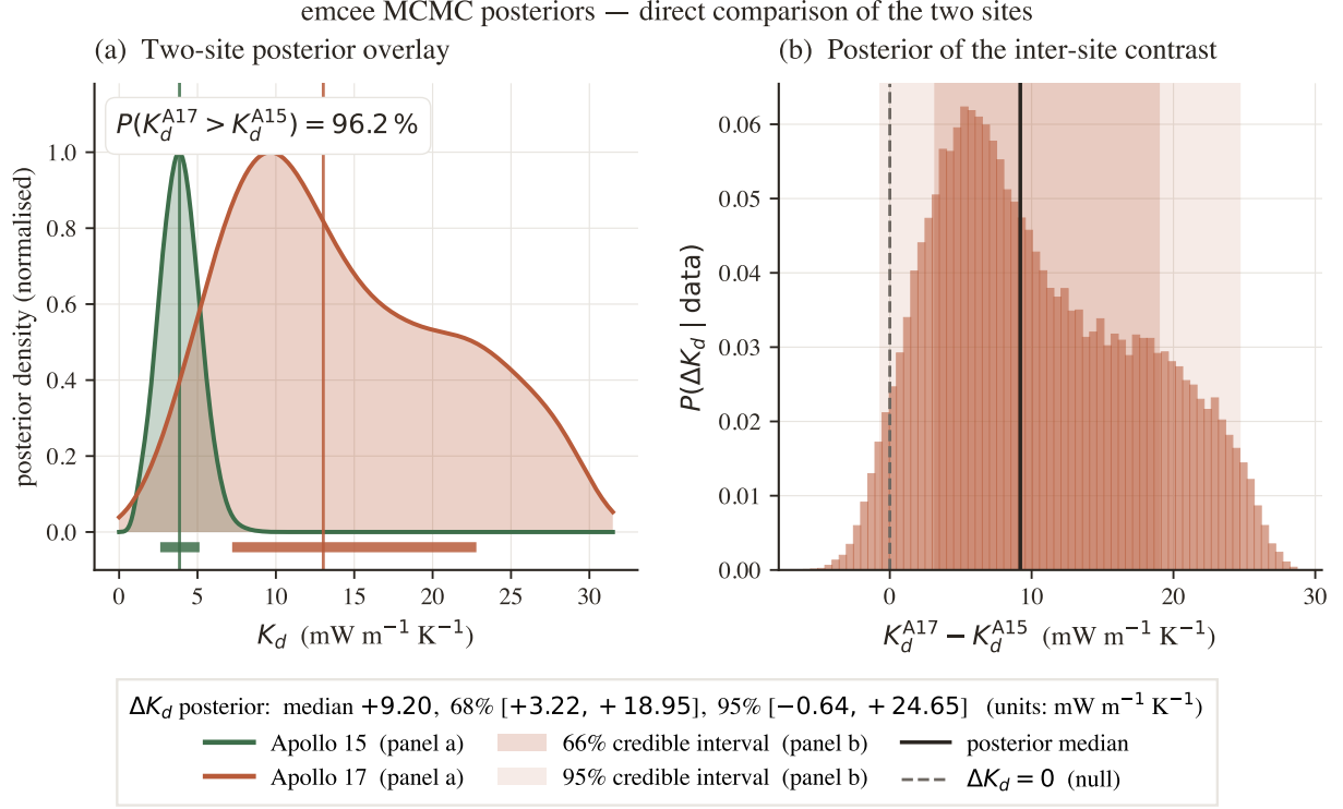
Figure 7. Direct two-site comparison of the MCMC posteriors. (a) The Apollo 15 (teal) and Apollo 17 (coral) marginal P(K_d | \text{data}) are overlaid on the same axes; filled curves are Gaussian-KDE estimates of the posterior, vertical lines mark medians, and the short bars at the foot of each curve span the 16–84 percentile range. The annotated probability is computed by drawing paired samples from the two marginals (the two sites’ data are independent), and quantifies how strongly the data discriminate K_d^{A17} from K_d^{A15} . (b) Posterior distribution of the inter-site contrast \Delta K_d \equiv K_d^{A17} - K_d^{A15} , formed from the same paired draws. The 66% (darker) and 95% (lighter) credible intervals are shaded; the dashed line at \Delta K_d = 0 shows the null hypothesis of a uniform deep conductivity. The bulk of the posterior mass lies above zero (with the 95% credible interval just touching zero at the lower bound, reflecting the widening that follows when the K_d/Q_b degeneracy is treated explicitly), providing a distribution-level statement of the inter-site contrast that complements the bootstrap-based contrast in Fig. 5.
