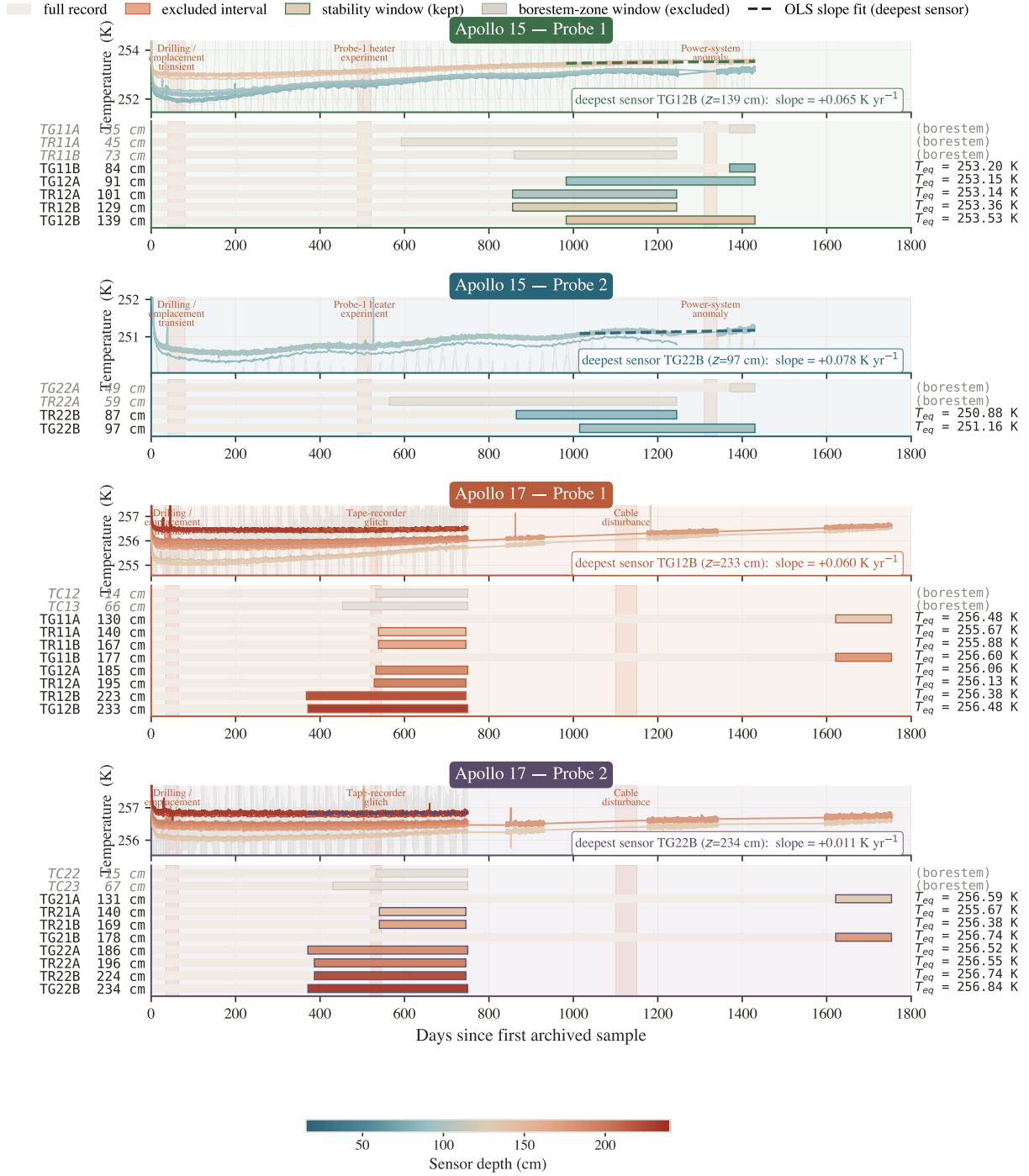
Figure 1. Per-probe stability-window timeline at Apollo 15 and 17. Raw HFE temperature traces (top sub-panel per probe) with documented disturbance intervals shown as translucent coral bands annotated by the physical event they correspond to: drilling / emplacement transient (residual heat released into the regolith over the first \sim 60 days as the borestem and probe came into thermal equilibrium with the surrounding regolith; Langseth et al. 1976; Nagihara et al. 2018); probe-1 heater experiment at A15 (an axial calibration heater pulsed in the gradient-bridge ring); power-system anomaly at A15 (TG-bridge data drop-out coincident with a reference-resistor switch); tape-recorder glitch at A17 (digitizer drop-outs in the restored Nagihara et al. 2018 record); and a brief A17 cable disturbance (Probe-2 cable fault). The bands are kept deliberately faint so the underlying traces remain readable; the selected stability windows are outlined and labelled with their OLS-fit long-term drift in mK 1/d. Lower sub-panel per probe: per-sensor stability-window Gantt strip colour-coded by sensor depth (sequential teal-coral scale on the shared colour bar). Sensor rows are ordered by depth (shallowest at top). The window-mean equilibrium temperatures listed at right-edge of each row are the T_{eq} values used in the deep-sensor RMSE (eq. 8).
