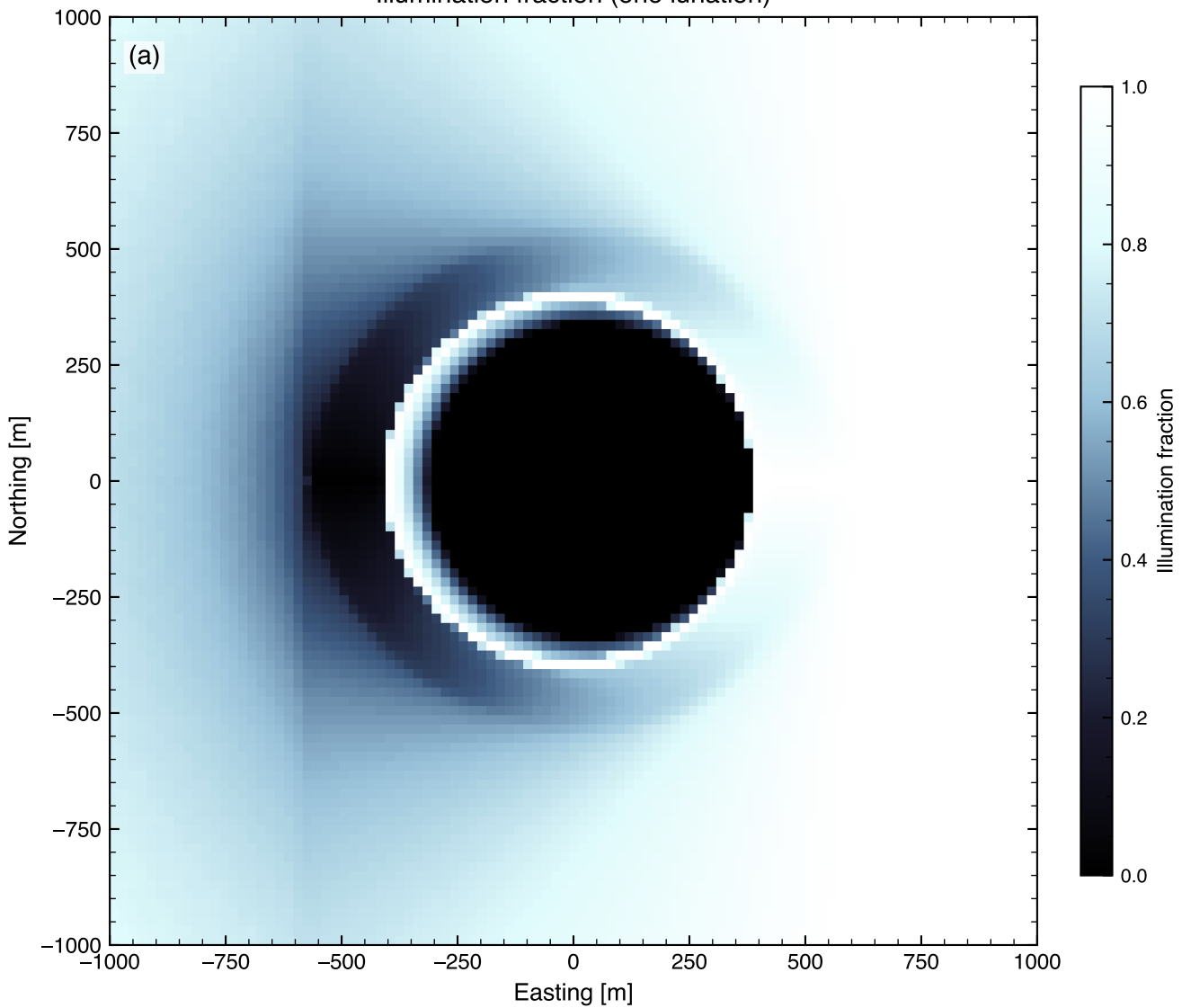
Illumination fraction (one lunation)
