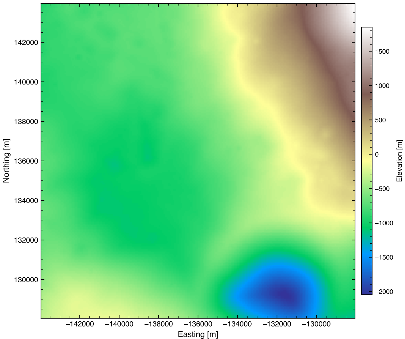
LOLA DEM subset — LDEM_80S_80MPP_ADJ.TIF
