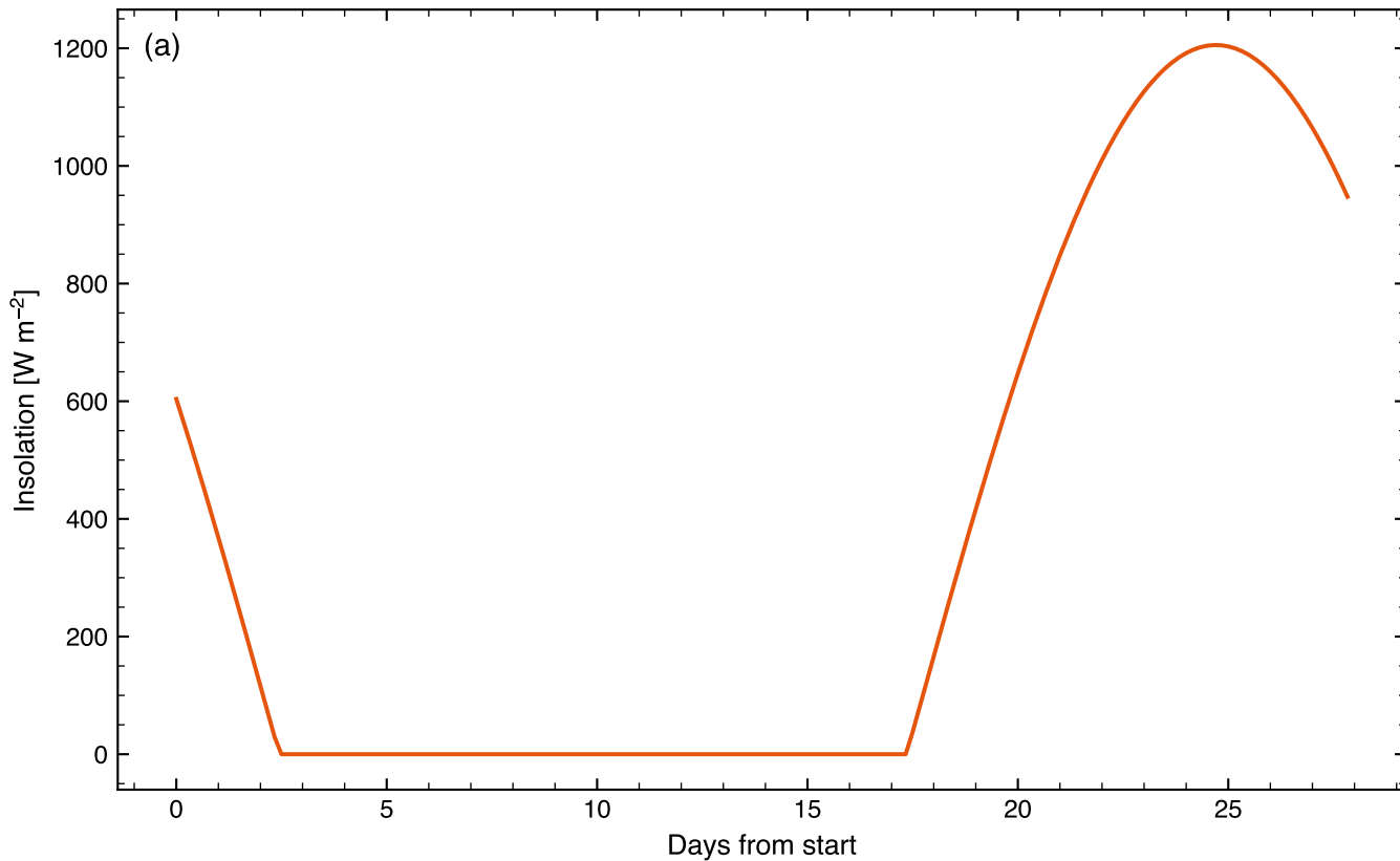
Insolation at 26.13°N, 3.63°E
