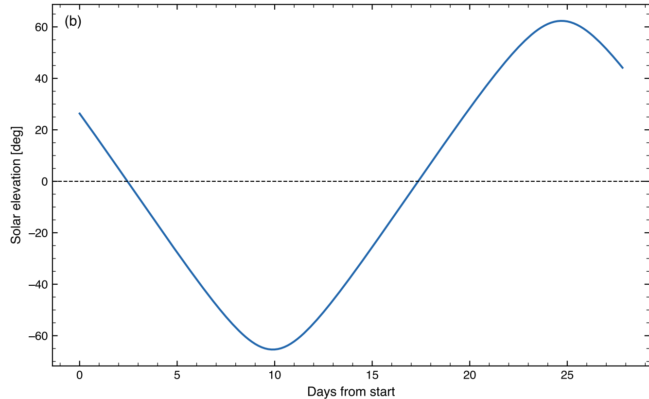
Solar elevation (SPICE/DE440)
