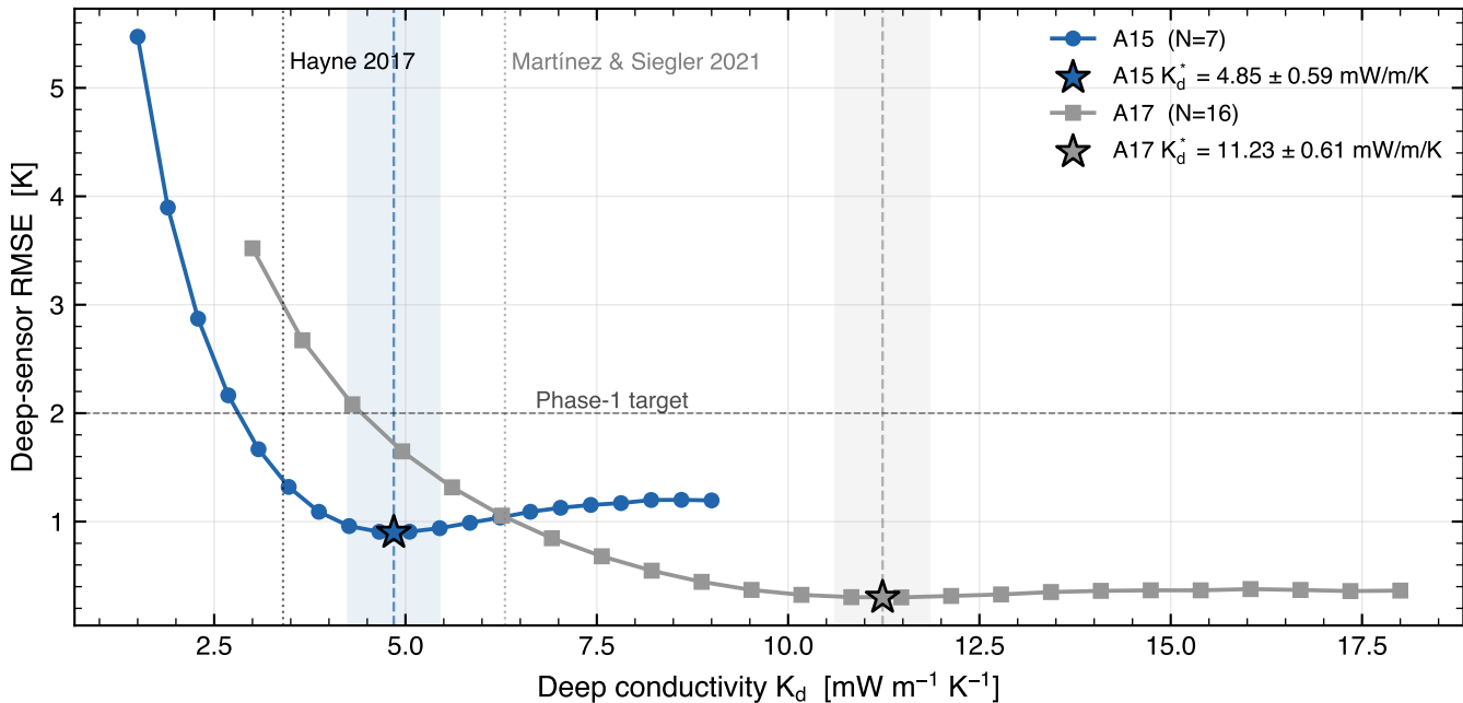
Per-site K_d retrieval with Hayne (2017) shape held fixed
