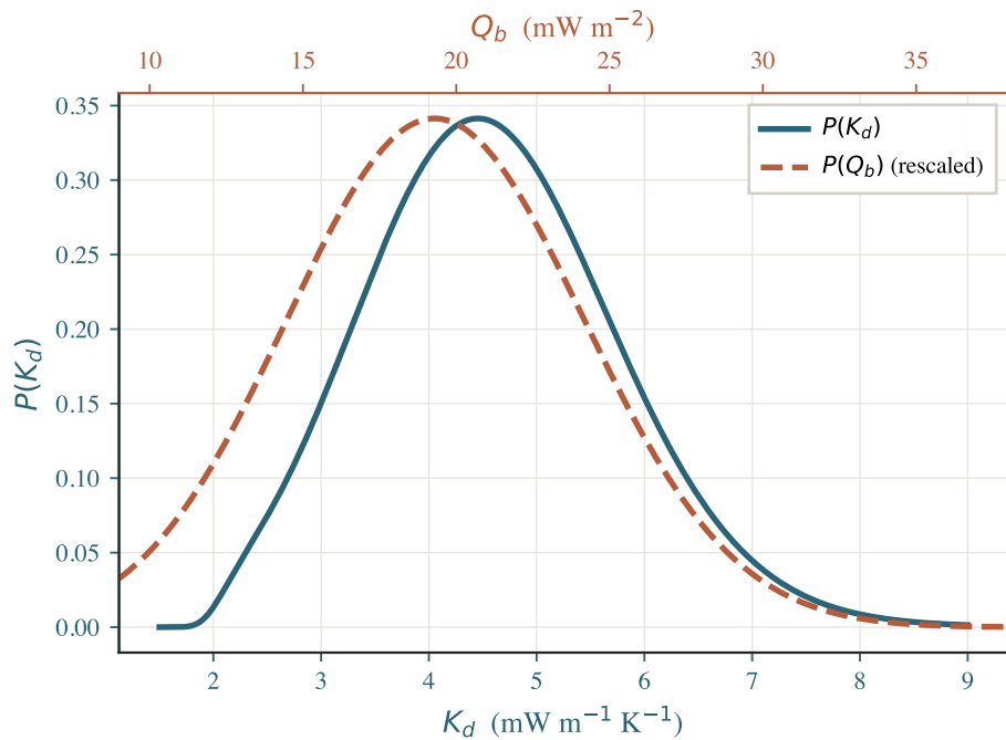
(c) A15 marginal posteriors
