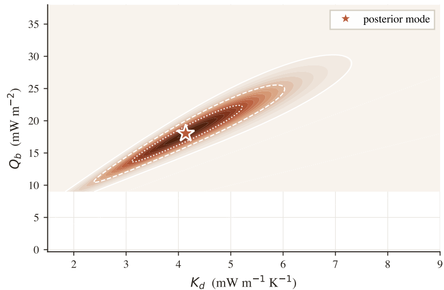
(c) A15 marginal posteriors
