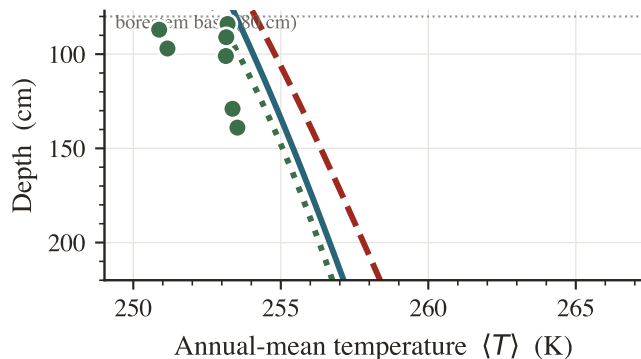
(c) Apollo 15 — deep-sensor zoom
