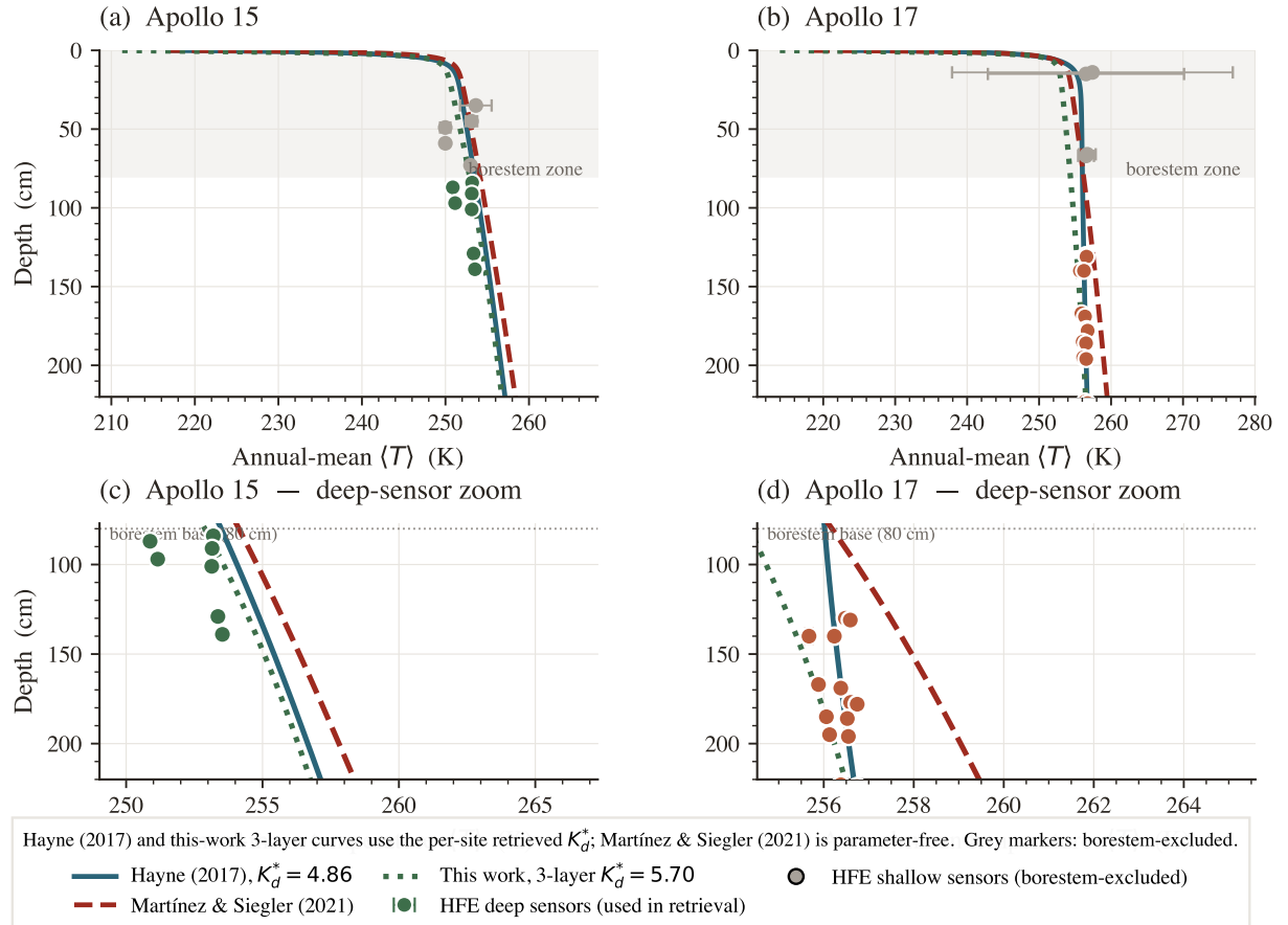
Figure 10. Annual-mean T(z) : three conductivity models against the Apollo HFE deep sensors. Solid teal: Hayne et al. (2017) at the per-site retrieved K_d^* ; dashed red: parameter-free Martínez and Siegler (2021); dotted green: this-work 3-layer at its per-site retrieved K_d^* . Top panels: full profile; bottom panels: deep-sensor zoom. Coloured markers: HFE deep sensors (used in retrieval); grey markers: borestem-affected shallow sensors (excluded).
