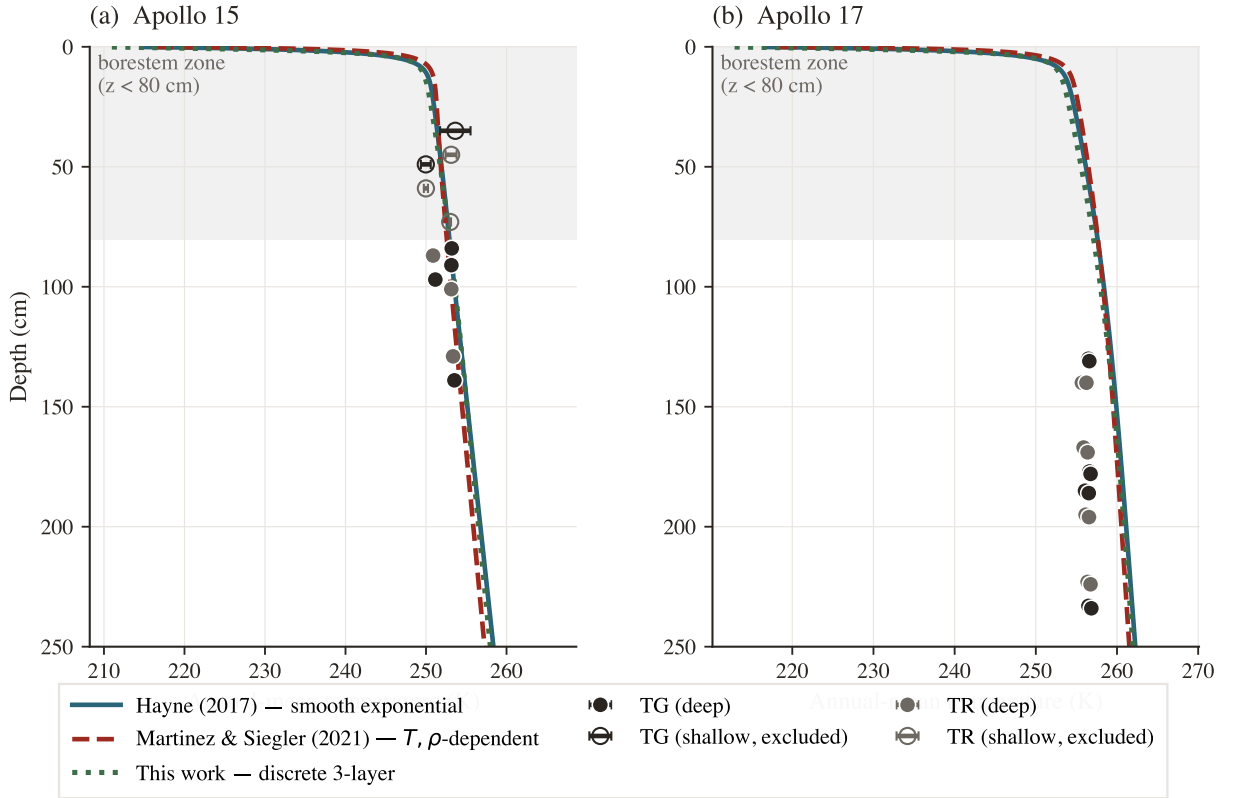
Figure 2. Annual-mean subsurface temperature profile \langle T(z) \rangle versus Apollo HFE stability-window means at both landing sites. Three conductivity models at their nominal (un-retrieved) parameters: Hayne et al. (2017) smooth-exponential (solid teal, global K_d = 3.4 ), Martínez and Siegler (2021) T, \rho -dependent (dashed red), and the this-work discrete 3-layer model (dotted green). Markers are coloured by sensor type (warm-charcoal = TG, grey = TR), with horizontal bars equal to the within-window standard deviation of the observed equilibrium temperature. The shaded band marks the borestem-contaminated zone ( z < 80 \text{ cm} ); sensors there are plotted but excluded from the quantitative RMSE in Table 2. Same parameters at both sites; only A , \varepsilon , latitude, Q_b vary (measured quantities).
