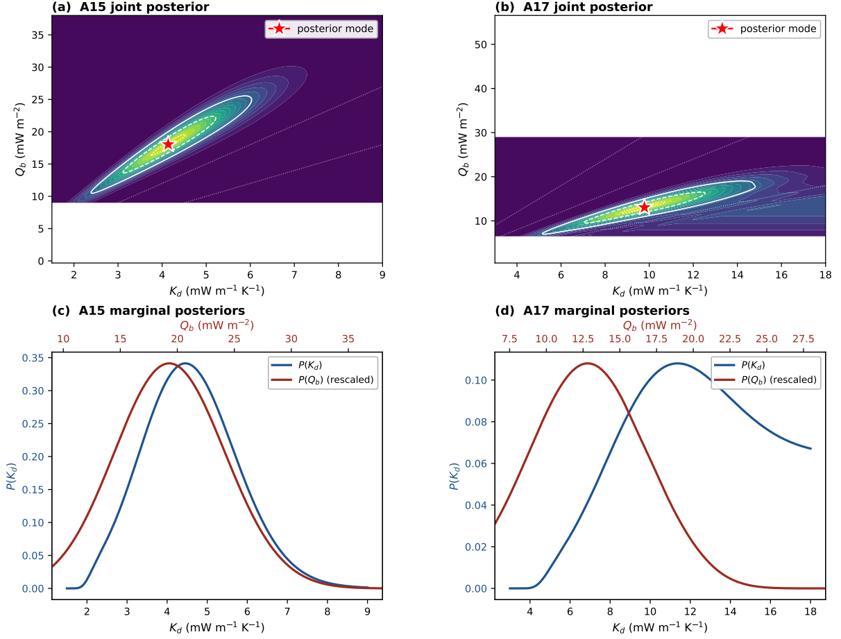
Figure 4.2. Joint Bayesian posterior in (K_d, Q_b) at the two Apollo sites. Panels (a)–(b): 2-D posterior densities with the maximum a posteriori marker (red star) and dotted iso-ratio lines Q_b/K_d = \text{const.} . Panels (c)–(d): the marginal posteriors on K_d (blue, left axis) and on Q_b (red, right axis). The posterior contracts onto the iso-ratio ridge along which the equilibrium temperature profile is invariant; the prior on Q_b breaks the degeneracy in only the orthogonal direction.
