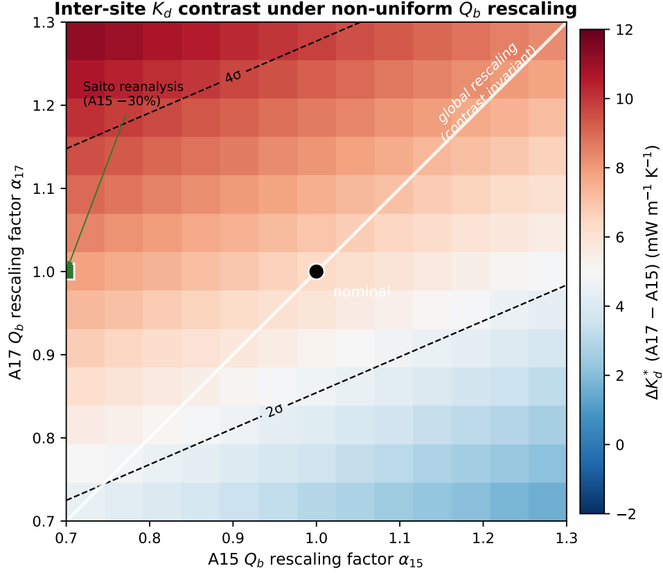
Figure 8. Inter-site K_d^* contrast under non-uniform Q_b rescaling. Heatmap of \Delta K_d^* as a function of independent rescaling factors \alpha_{15} and \alpha_{17} on the published basal heat fluxes at each site. The white diagonal marks "global" rescaling ( \alpha_{15} = \alpha_{17} ), under which the contrast is exactly invariant. Dashed black contours give the contrast significance ( \sigma ) computed against the bootstrap standard error. The black circle shows the nominal published Q_b at both sites and the red square shows the Saito et al. (2007); Nagihara et al. (2018) reanalysis configuration in which Q_{b,A15} is reduced by 30% with Q_{b,A17} held fixed. The contrast remains significant at \geq 4\sigma across the entire reanalysis envelope.
