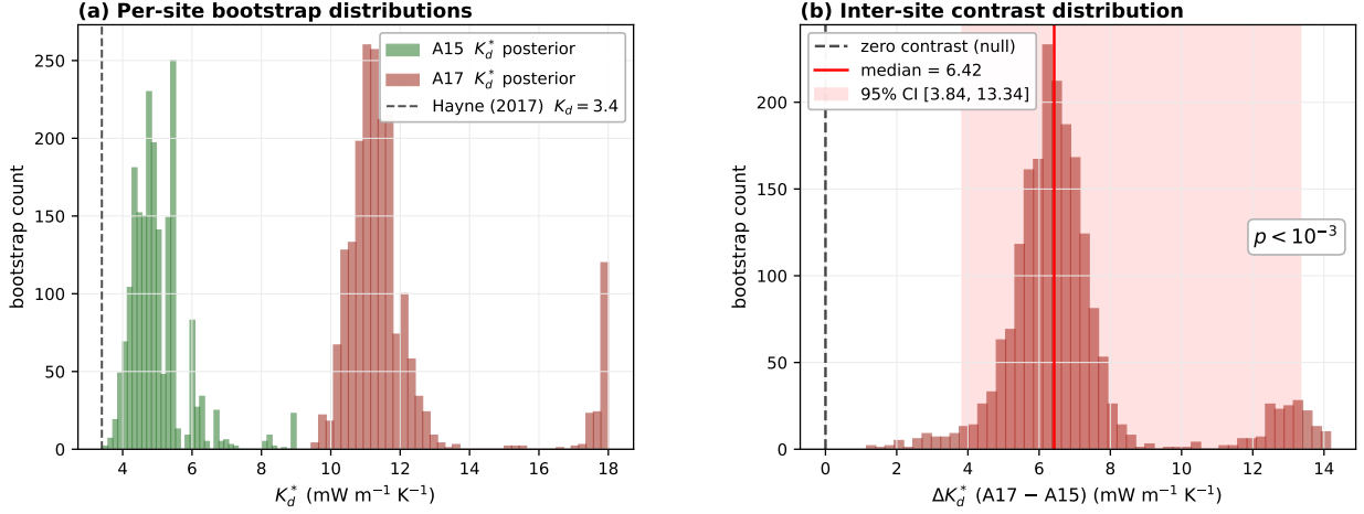
Figure 7. Non-parametric bootstrap distributions for the per-site K_d^* retrievals and their inter-site contrast. (a) Histograms of K_d^* from N_{\text{boot}} = 2000 resamples of the deep-sensor set at each site (with replacement); markers below each histogram show the median (downward triangles) and 95% bootstrap confidence intervals (horizontal bars). The vertical dashed line marks the published global value K_d = 3.4 \text{ mW}/(\text{m K}) . (b) Distribution of the inter-site contrast \Delta K_d^* = K_{d,A17}^* - K_{d,A15}^* , with the 95% bootstrap CI shaded; the distribution does not overlap zero, giving p < 10^{-3} for the null of inter-site equality.
