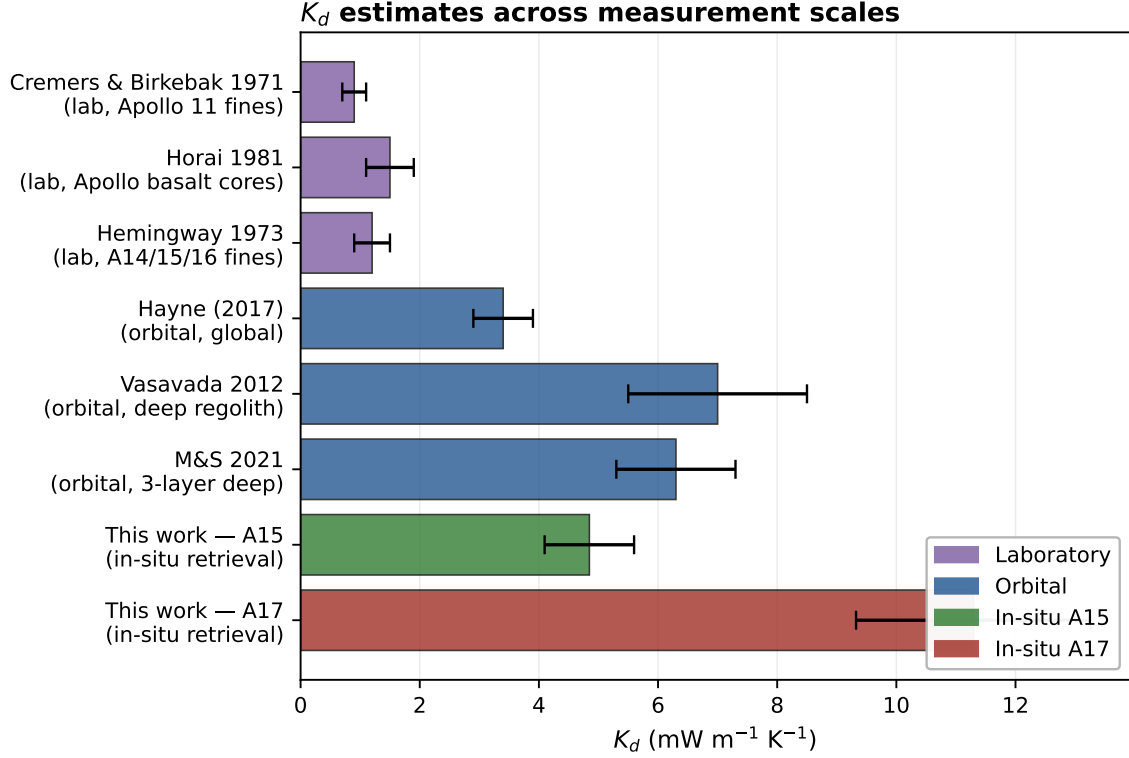
Figure 10. K_d estimates across measurement scales. Laboratory measurements on returned Apollo regolith samples (Cremers and Birkebak, 1971; Horai, 1981; Hemingway et al., 1973) cluster at \sim 1 mW/(m K); orbital fits (Hayne et al., 2017; Vasavada et al., 2012; Martínez and Siegler, 2021) span \sim 3 – 7 \times 10^{-3} W/(m K); and the present in-situ retrievals lie at \sim 5 (A15) and \sim 11 (A17) mW m -1 K -1 . Error bars are the published 1-sigma laboratory uncertainties, an indicative \sim 20\% on the orbital fits, and the bootstrap standard error on the in-situ retrievals.
