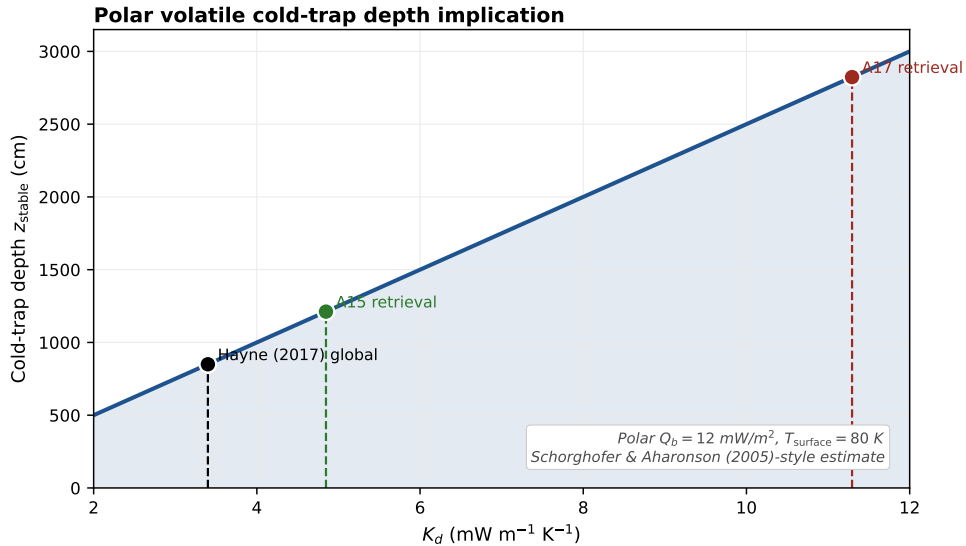
Figure 11. Implication for polar volatile cold-trap depth. Indicative cold-trap depth z_{\text{stable}} at which buried water ice is thermally stable on geological timescales (a Schorghofer and Aharonson 2005-style estimate at fixed polar surface temperature and basal heat flux), as a function of K_d . The factor-of- \sim 3 change in K_d between the global value of Hayne et al. (2017) and the A17 retrieval translates into a factor-of- \sim 3 change in z_{\text{stable}} , illustrating that the regional heterogeneity in K_d reported here is large enough to matter for downstream volatile-stability budgets.
