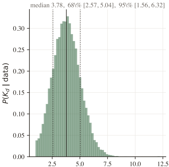
(c) Apollo 15 — marginal P(K_d)
