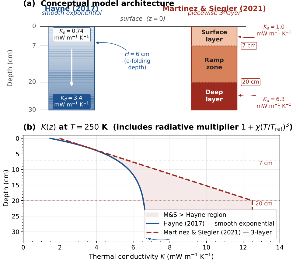
Figure 1. Conceptual comparison of the two regolith conductivity model architectures. (a) Physical layer structure: the Hayne et al. (2017) profile (blue) transitions continuously from a surface value K_s = 0.74 \text{ mW m}^{-1} \text{ K}^{-1} to a deep value K_d = 3.4 \text{ mW m}^{-1} \text{ K}^{-1} via an exponential with H = 6 \text{ cm} ; the Martínez and Siegler (2021) 3-layer profile (red) has a uniform surface layer ( K_s = 1.0 \text{ mW m}^{-1} \text{ K}^{-1} , 0–7 cm), a linear ramp zone (7–20 cm), and a uniform deep layer ( K_d = 6.3 \text{ mW m}^{-1} \text{ K}^{-1} , below 20 cm). (b) The corresponding K(z) profiles evaluated at T = 250 \text{ K} including the radiative multiplier 1 + \chi(T/T_{\text{ref}})^3 ; the shaded region is where the Martínez and Siegler (2021) conductivity exceeds the Hayne et al. (2017) value. The factor-of- \sim 2 difference in K_d is the dominant control on the deep-gradient discrepancy in Table 1.
