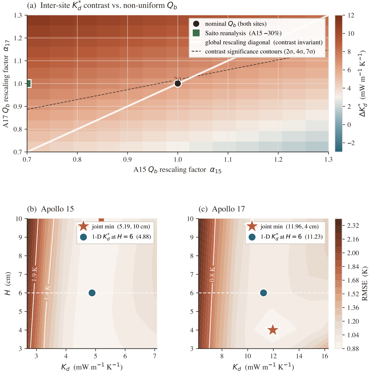
Figure 6. Robustness of the per-site K_d^* contrast. (a) Inter-site contrast \Delta K_d^* as a function of independent per-site rescaling factors \alpha_{15}, \alpha_{17} on the published basal heat fluxes; the white diagonal marks global rescaling, under which the contrast is exactly invariant. Dashed contours give the bootstrap-normalised significance ( \sigma ). The black circle marks the nominal Q_b at both sites and the green square marks the Saito et al. (2007) ; Nagihara et al. (2018) reanalysis at A15. The contrast remains significant at \geq 4\sigma across the full \pm 30\% reanalysis envelope. (b)–(c) Two-parameter joint fit of K_d and the e-folding depth H at each site; white contours are at the labelled RMSE values above the joint minimum. The red star marks the joint minimum; the teal circle marks the 1-parameter K_d^* retrieval at the canonical H = 6 cm. The two minima coincide to within the 0.5 K RMSE contour, indicating that K_d is the dominant identified lever and that the retrieval is not a degenerate trade-off with H .
