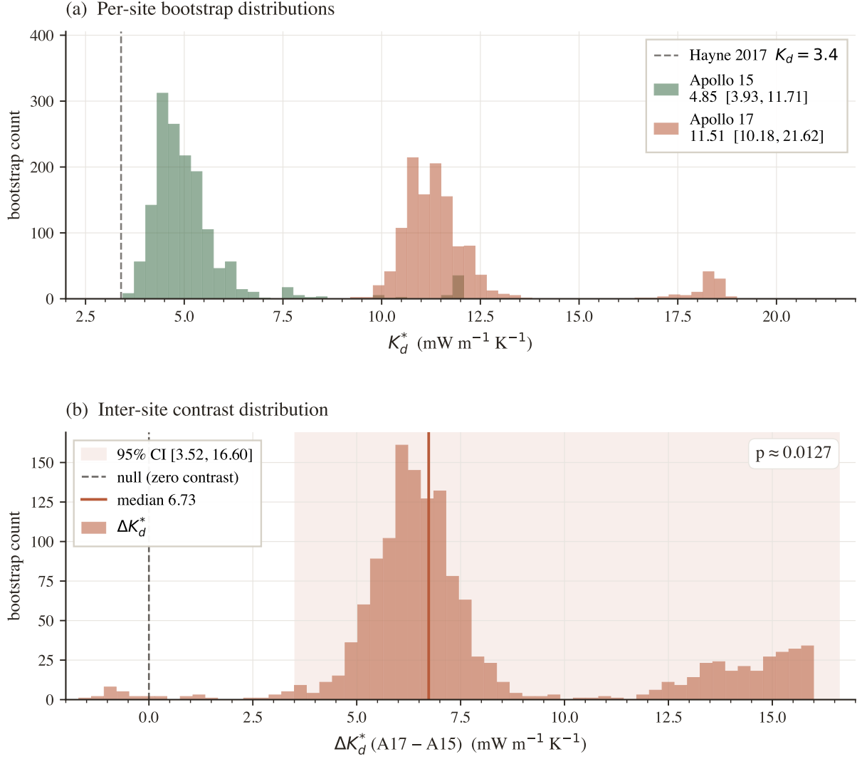
Figure 5. Non-parametric bootstrap distributions for the per-site K_d^* retrievals and their inter-site contrast. (a) Bootstrap histograms of K_d^* from N_{\text{boot}} = 2000 resamples of the deep-sensor set at each site (with replacement and with the published \pm 2.5 cm sensor-placement uncertainty propagated). The 95% confidence intervals are listed in the legend. The vertical dashed line marks the published global value K_d = 3.4 \text{ mW}/(\text{m K}) . (b) Distribution of the inter-site contrast \Delta K_d^* = K_{d,A17}^* - K_{d,A15}^* , with the 95% bootstrap CI shaded. The distribution does not overlap zero, giving p \approx 0.013 for the null of inter-site equality.
