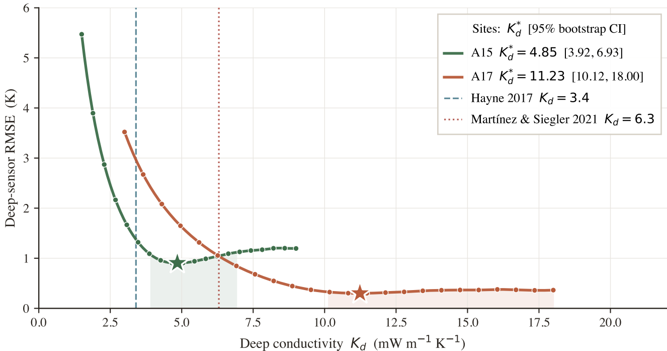
Per-site K_d retrieval under the Hayne 2017 functional form
