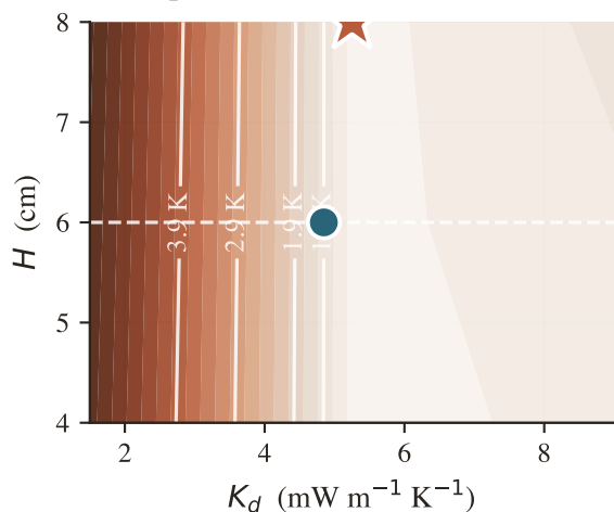
(b) Apollo 15
