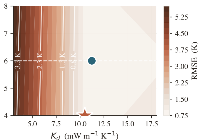
(c) Apollo 17
