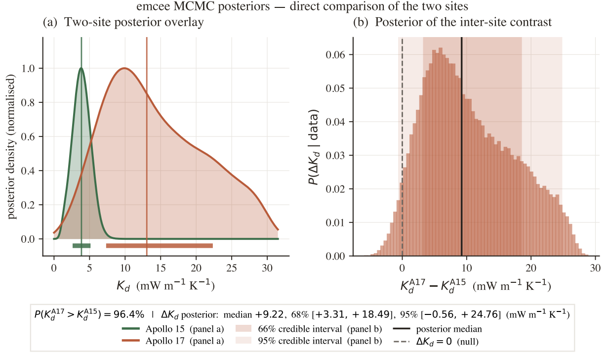
Figure 7. Direct two-site comparison of the MCMC posteriors. (a) The Apollo 15 (teal) and Apollo 17 (coral) marginal P(K_d | \text{data}) are overlaid on the same axes; filled curves are Gaussian-KDE estimates of the posterior, vertical lines mark medians, and the short bars at the foot of each curve span the 16–84 percentile range. The annotated probability is computed by drawing paired samples from the two marginals (the two sites’ data are independent), and quantifies how strongly the data discriminate K_d^{A17} from K_d^{A15} . (b) Posterior distribution of the inter-site contrast \Delta K_d \equiv K_d^{A17} - K_d^{A15} , formed from the same paired draws. The 66% (darker) and 95% (lighter) credible intervals are shaded; the dashed line at \Delta K_d = 0 shows the null hypothesis of a uniform deep conductivity. The bulk of the posterior mass lies above zero (with the 95% credible interval just touching zero at the lower bound, reflecting the widening that follows when the K_d/Q_b degeneracy is treated explicitly), providing a distribution-level statement of the inter-site contrast that complements the bootstrap-based contrast in Fig. 5.
