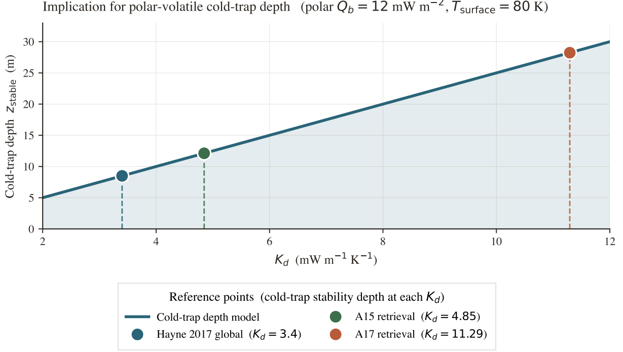
Figure 8. Implication for polar volatile cold-trap depth. Indicative cold-trap depth z_{\text{stable}} at which buried water ice is thermally stable on geological timescales (a Schorghofer and Aharonson 2005-style estimate at fixed polar surface temperature and basal heat flux), as a function of K_d . The factor-of- \sim 3 change in K_d between the global value of Hayne et al. (2017) and the A17 retrieval translates into a factor-of- \sim 3 change in z_{\text{stable}} .
