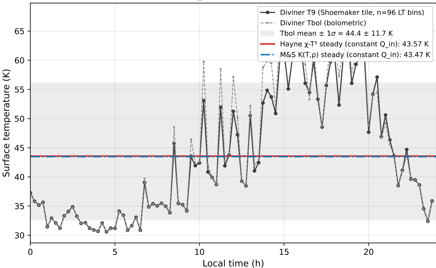
Phase 2 Fig. 3 (preliminary) — Shoemaker PSR surface T Constant-scattered-flux approx: Q_{\text{scatter}} = 191.1 \text{ mW/m}^2 (calibrated to T_{\text{bol}} mean)
