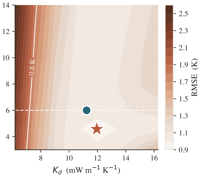
(c) Apollo 17
