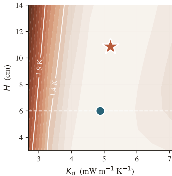
(b) Apollo 15
