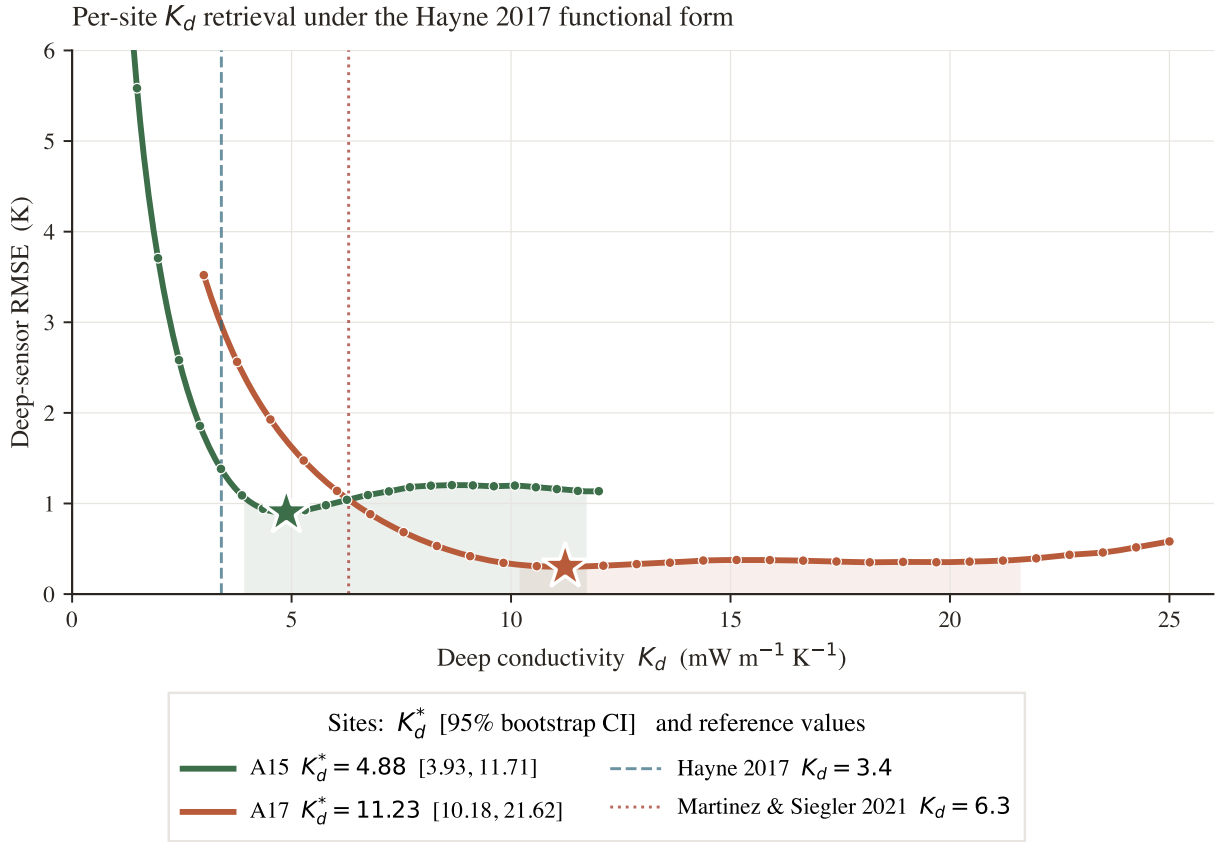
Figure 4. Per-site K_d retrieval under the Hayne et al. (2017) functional form. Deep-sensor RMSE (eq. 8) as a function of K_d , with K_s , H , \chi , T_{\text{ref}} , \rho(z) and c_p(T) all held at their published values. Filled markers are the swept grid; the solid curve is the parabolic refinement through the three values bracketing the minimum; and the shaded band is the bootstrap 95% confidence envelope. Vertical dashed lines mark the published Hayne et al. (2017) value (3.4 mW/(m K)) and the Martínez and Siegler (2021) 3-layer deep value (6.3 mW/(m K)). The two landing-site optima differ by approximately 6.7 mW/(m K), with a 95% bootstrap CI that excludes zero (Fig. 5).
