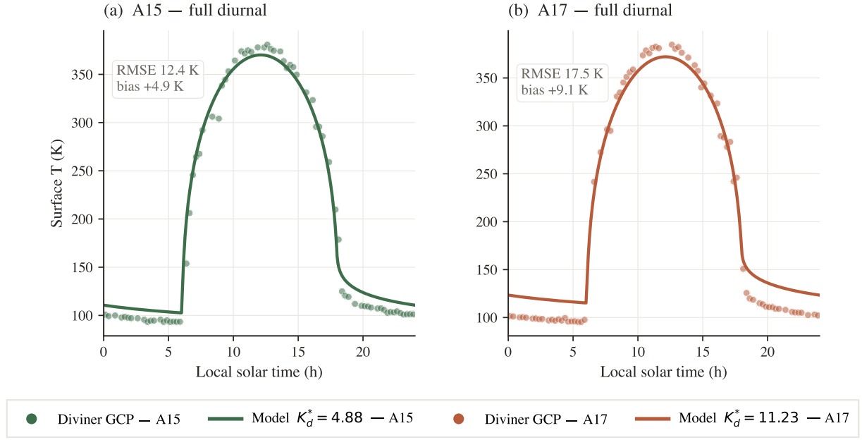
Figure 7. Surface-temperature closure against the Diviner Lunar Radiometer Global Cumulative Product. Modelled surface temperature (solid lines) at Apollo 15 (teal) and Apollo 17 (coral), run with the per-site retrieved K_d^* , overlaid on the Diviner Williams et al. (2017) diurnal brightness-temperature composite (markers). Terminator timing, daytime plateau width, and night-time floor are faithfully reproduced at both sites (full-cycle RMSE 12.4 K and 17.5 K at A15 and A17 respectively); the model runs slightly warmer than the Diviner composite across the full cycle, with the largest discrepancy on the night side, consistent with the well-documented anisothermal-footprint and sub-pixel rock-population effects (Bandfield et al., 2015; Hayne et al., 2017) and does not affect the deep-gradient retrieval. Per-site night-only residuals are tabulated in the Supporting Information.
