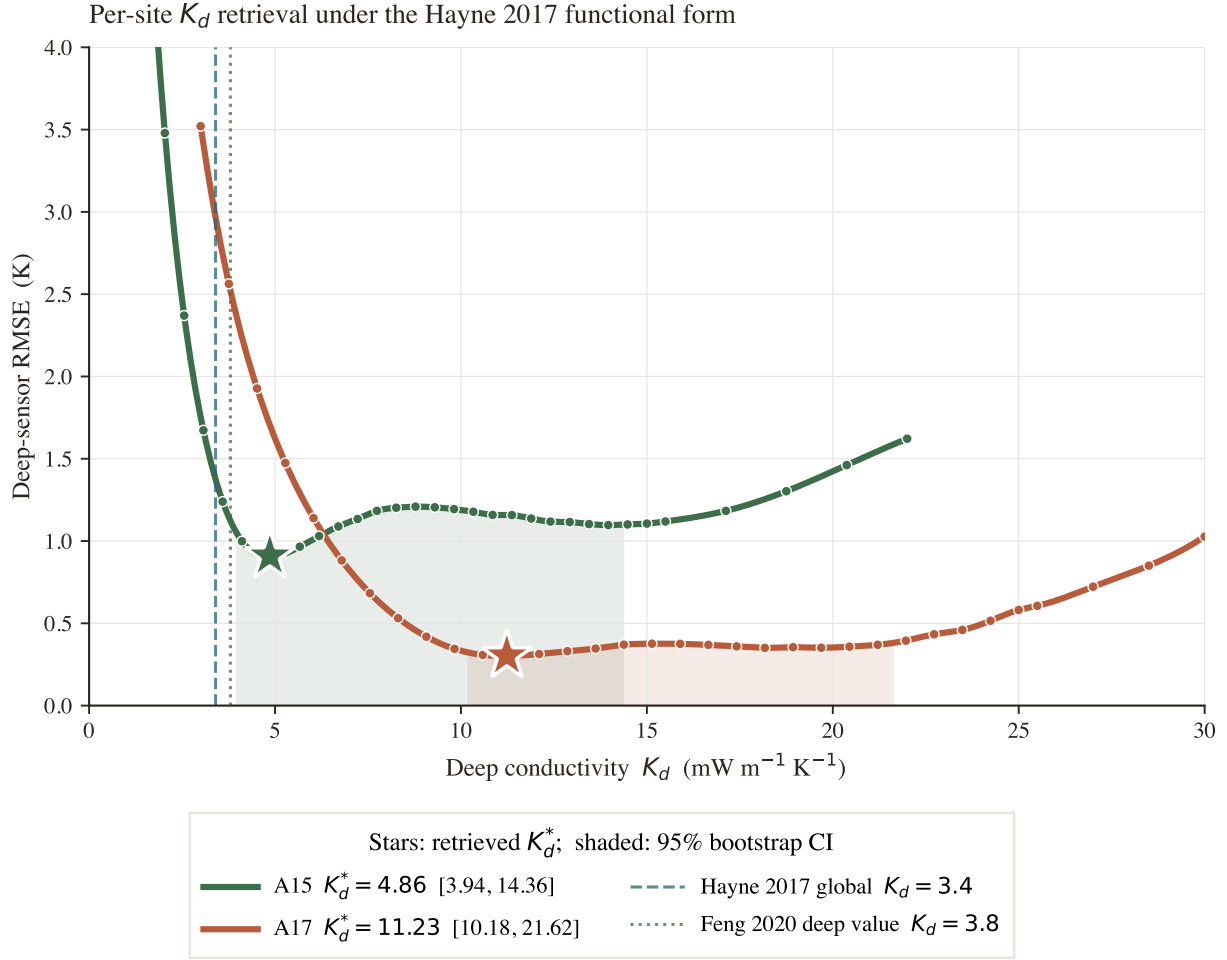
Figure 6. Per-site K_d retrieval under the Hayne et al. (2017) functional form, with all other Hayne et al. (2017) parameters held at their published values. Deep-sensor \text{RMSE}(K_d) at each site, extended past the fitting grid so each curve is shown rising again on the high- K_d side: the minima are genuine bracketed bowls, not descending shoulders. Markers: forward-model evaluations; stars: retrieved K_d^* ; shaded band: 95% bootstrap CI. Dashed vertical: Hayne et al. (2017) global K_d = 3.4 ; dotted: the Feng et al. (2020) deep value K_d = 3.8 .
