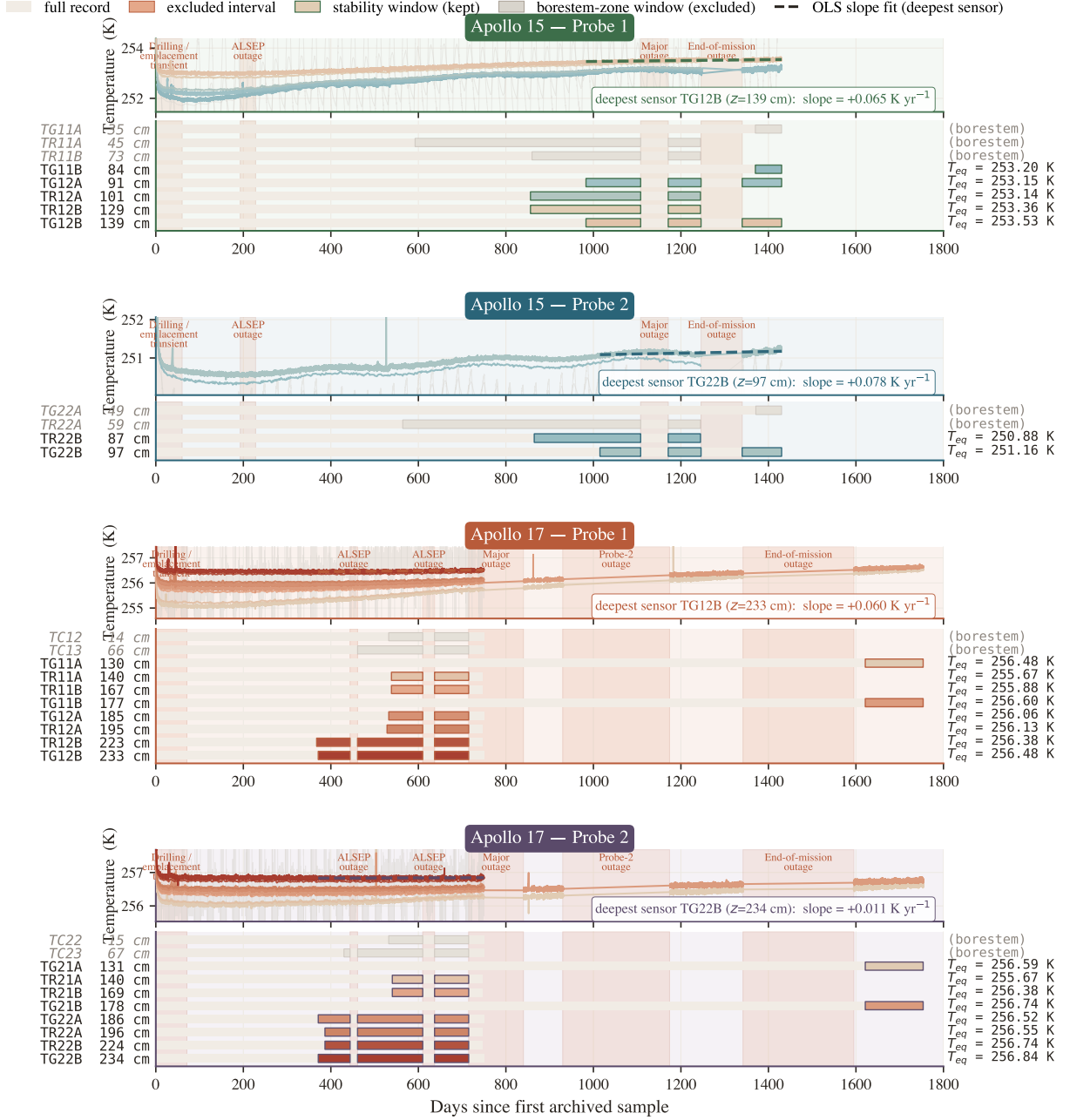
Figure 3. Per-probe stability-window timeline at Apollo 15 and 17 (4 probes). Each probe panel shows, above, the raw HFE traces with coral bands marking documented data-quality events and the selected stability windows outlined; and, below, a depth-coded per-sensor Gantt strip broken at outages. Selection criteria and the role of the window-mean T_{eq} are described in §2.
