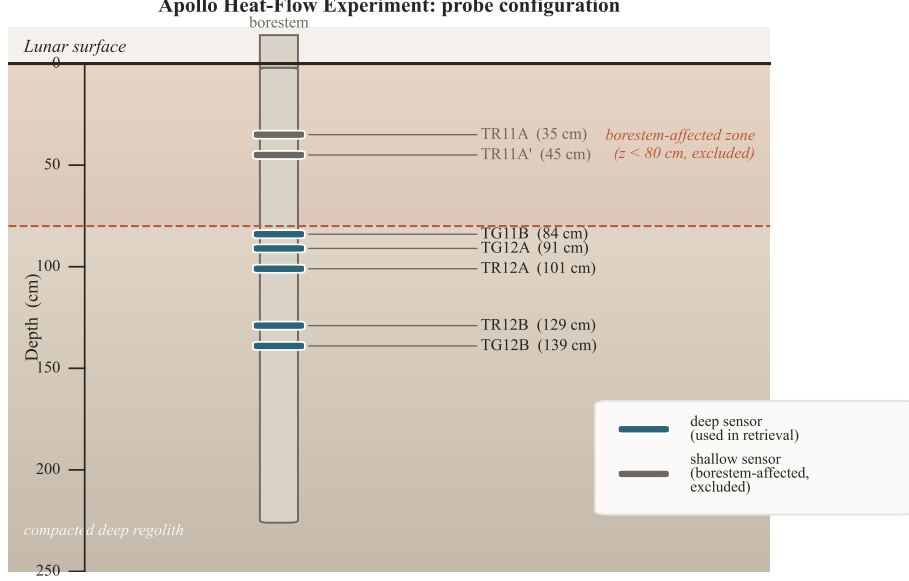
Figure 1. Configuration of an Apollo Heat-Flow Experiment probe. A fibreglass borestem, emplaced by the astronauts, carries gradient-bridge and ring-bridge thermometers at fixed depths along the regolith column (representative Apollo 15 Probe-1 placements shown). Heat conducted down the borestem from the surface contaminates the uppermost \sim 80 cm (coral band); only the sensors below that depth (teal) are used in the conductivity retrieval.
