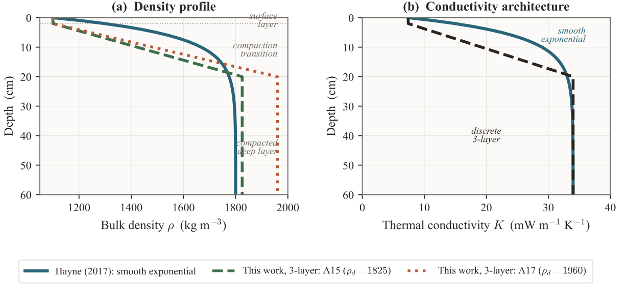
Figure 2. The two conductivity-model architectures considered here. (a) Bulk-density profile \rho(z) : the Hayne et al. (2017) smooth-exponential form against the this-work discrete three-layer model, the latter shown at both the Apollo 15 and 17 deep bulk densities. (b) The corresponding thermal-conductivity architecture K(z) — a smooth exponential rise versus a surface layer, a compaction transition, and a compacted deep layer. Only the top 60 cm is shown, below which all profiles are flat.
