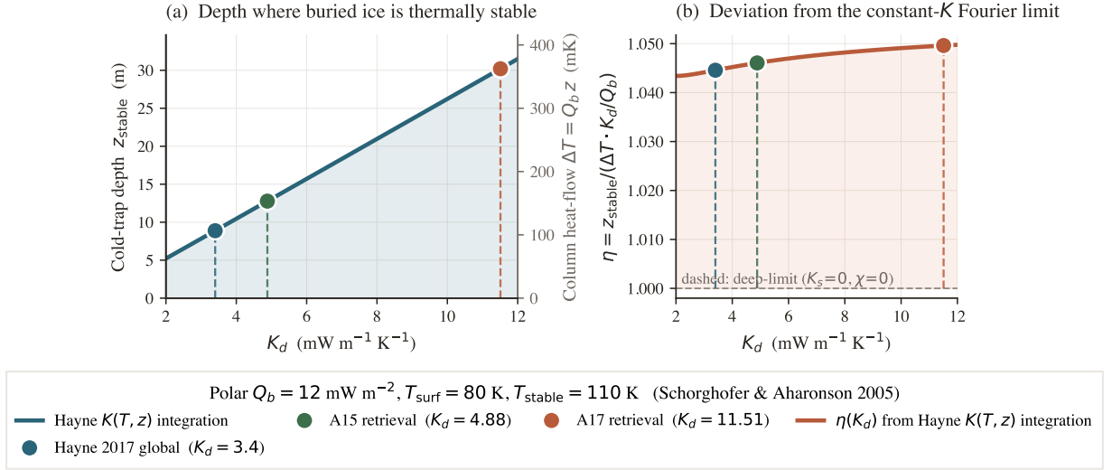
Figure 11. Polar cold-trap depth vs. K_d (Schorghofer-2005-style estimate at T_{\text{surf}} = 80 \text{ K} , Q_b = 12 \text{ mW/m}^2 ). (a) z_{\text{stable}} from RK4 forward-integration of dT/dz = Q_b/K(T, z) through the Hayne K(T, z) profile until T = T_{\text{stable}} = 110 \text{ K} ; the right axis recasts the same depth as the column heat-flow drop \Delta T = Q_b z . The curve is close to linear because the Q_b/K_d term dominates. (b) Ratio \eta = z_{\text{stable}}/[(\Delta T) K_d/Q_b] relative to the constant- K Fourier limit; \eta \approx 1.04\text{--}1.05 resolves the mild ( \sim 5\% ) departure from linearity from the shallow- K_s layer and the radiative term.
