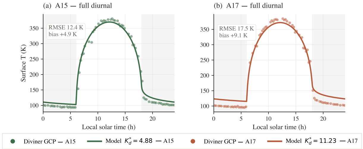
Figure 9. Surface-T closure against the Diviner Lunar Radiometer GCP. Modelled surface T (solid) at A15 (teal) and A17 (coral) with per-site K_d^* , vs. Diviner (Williams et al., 2017) diurnal composite (markers); shaded bands = night (LST < 6 or \geq 18 h). Full-cycle RMSE 12.4 and 17.5 K. The model is slightly warmer than Diviner across the cycle, with the largest discrepancy on the night side, consistent with anisothermal-footprint and sub-pixel rock-population effects (Bandfield et al., 2015; Hayne et al., 2017).
