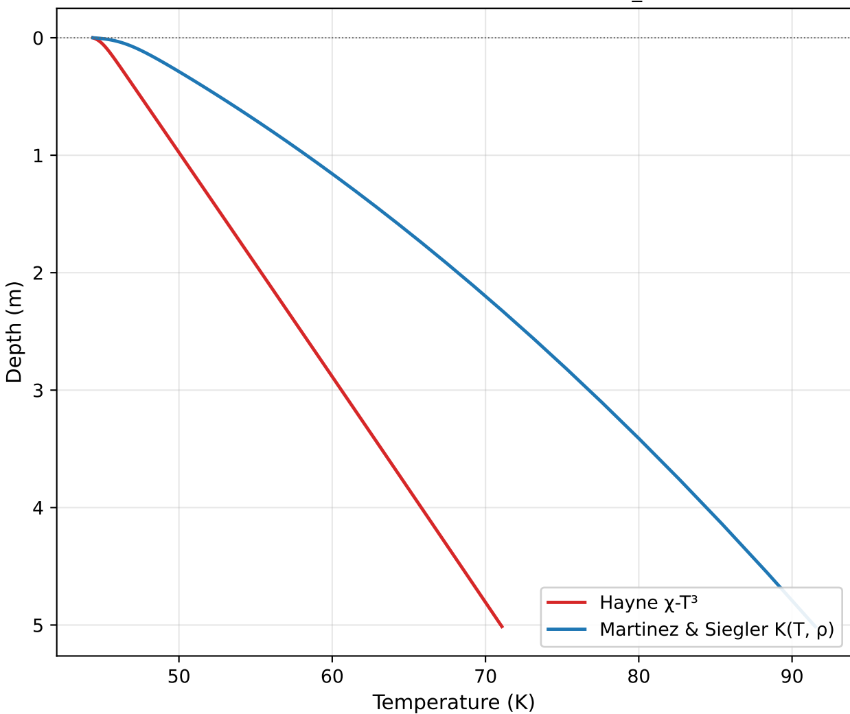
Phase 2 Fig. 4 — Shoemaker PSR T(z) profile Dirichlet T(0)=44.4 K (Diviner Tbol time-mean), Q b =18 mW/m 2
