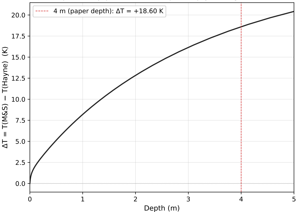
Phase 2 Fig. 5 (1D proxy) — K-model T-disagreement vs depth at Shoemaker (Replaces the paper's 2D 4-m \Delta T map; same physics, single column)
