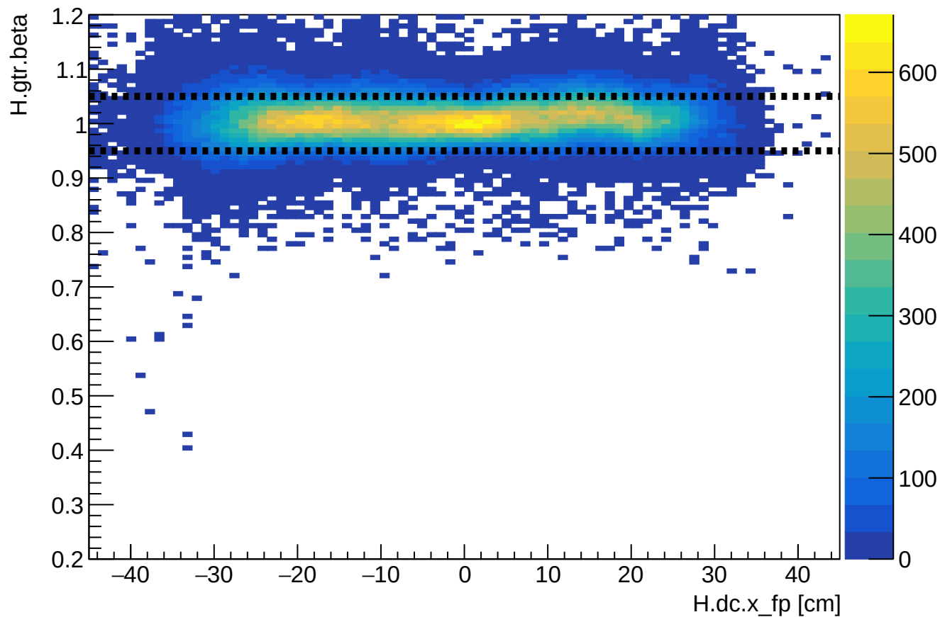
Phase 2 run 28229: HMS beta vs HMS xfp
