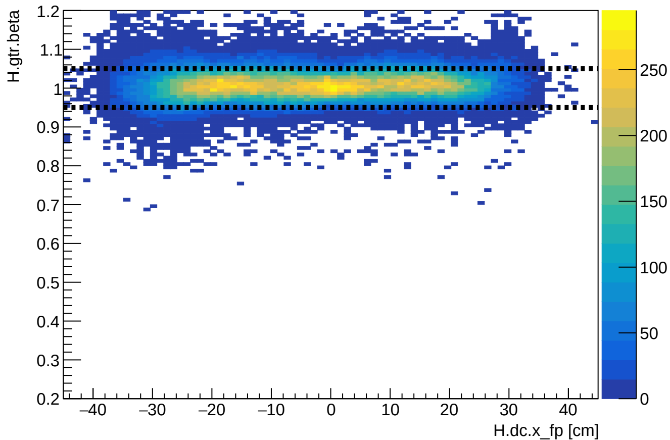
Phase 2 run 27192: HMS beta vs HMS xfp
