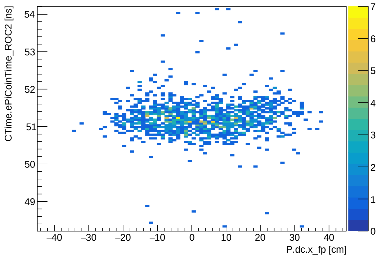
Phase 1 run 24117: CTime (ROC2) vs SHMS xfp
