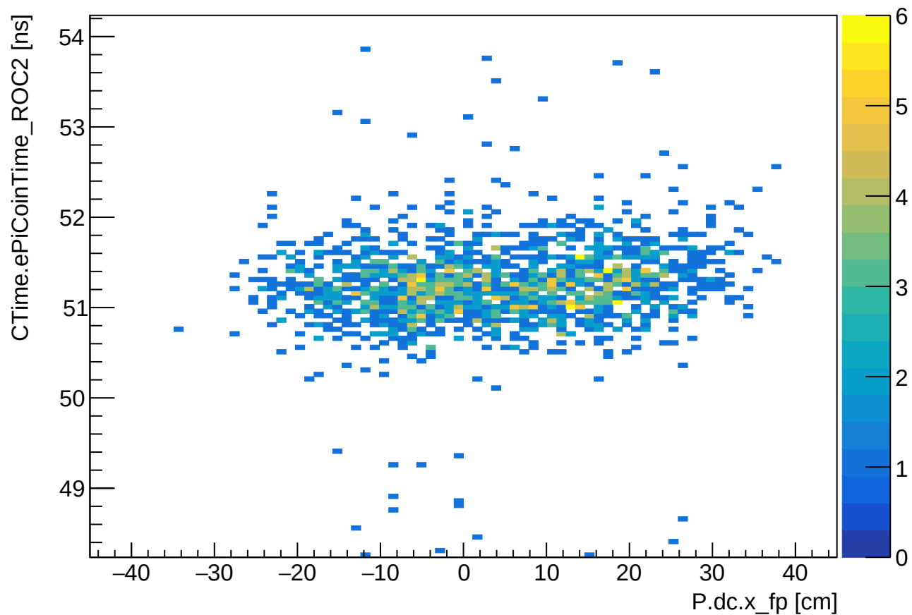
Phase 1 run 24112: CTime (ROC2) vs SHMS xfp
