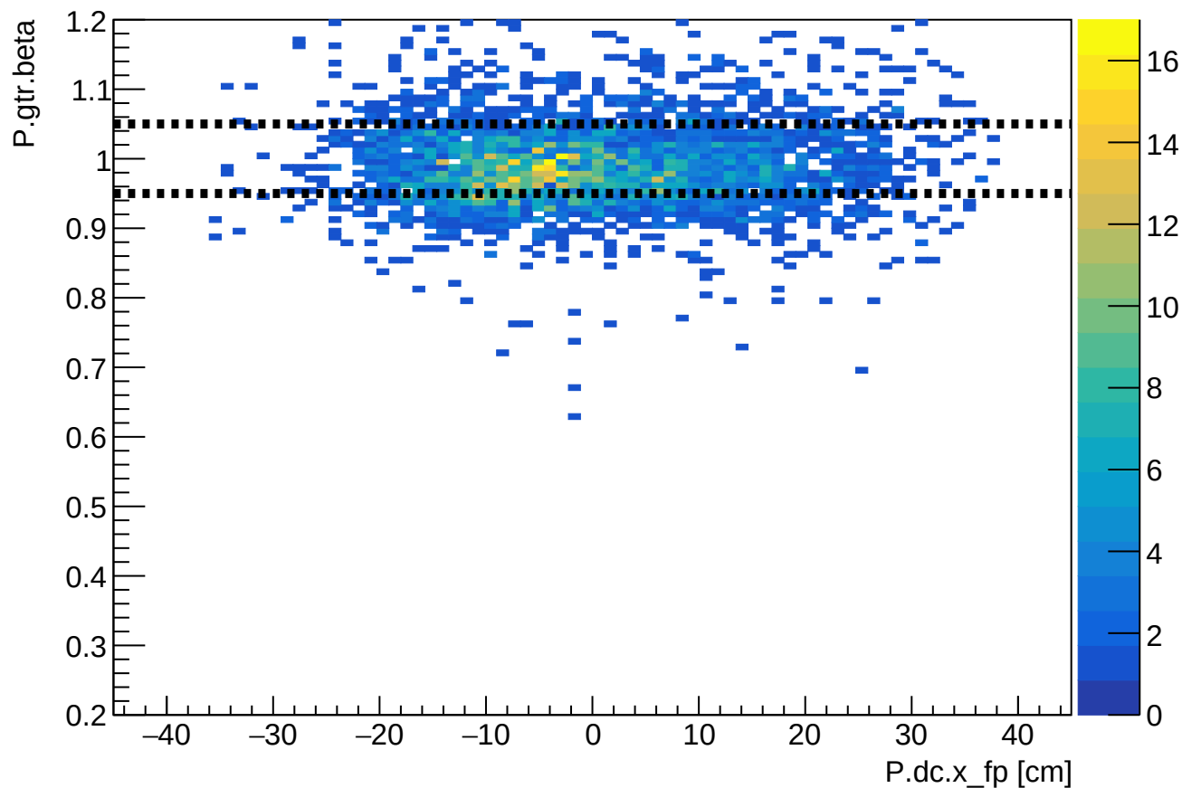
Phase 1 run 24040: SHMS beta vs SHMS xfp
