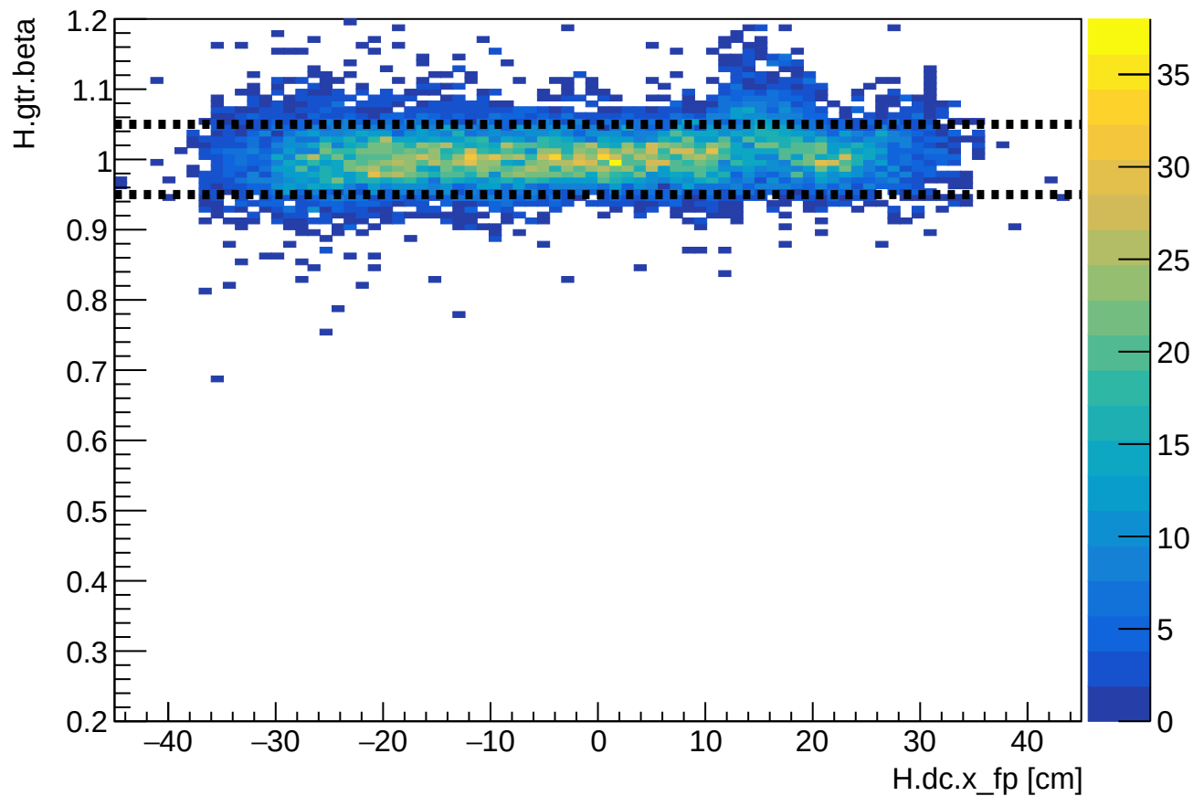
Phase 1 run 24112: HMS beta vs HMS xfp
