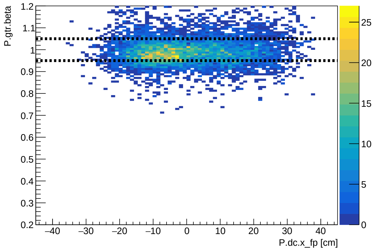
Phase 1 run 24117: SHMS beta vs SHMS xfp
