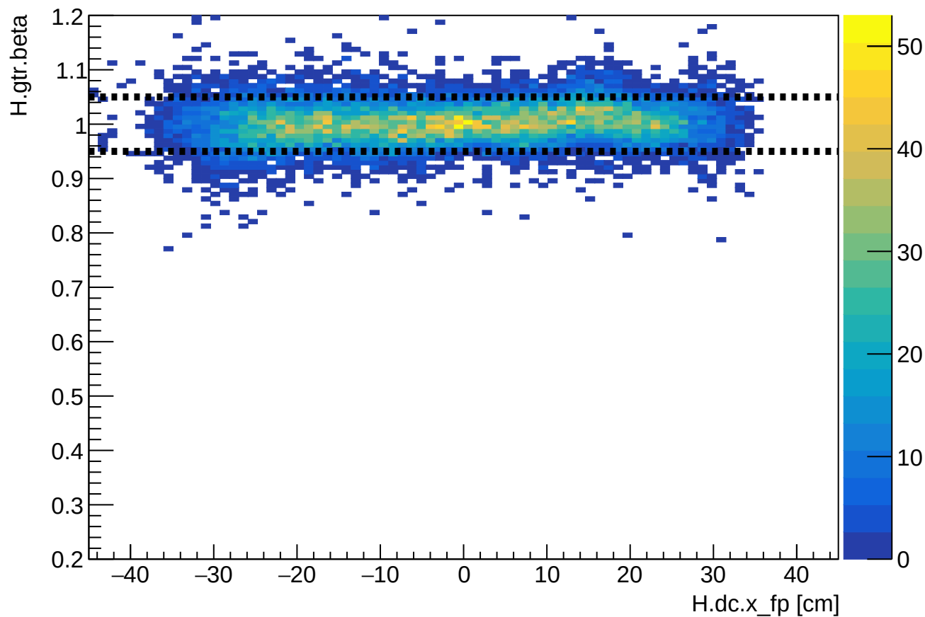
Phase 1 run 24647: HMS beta vs HMS xfp
