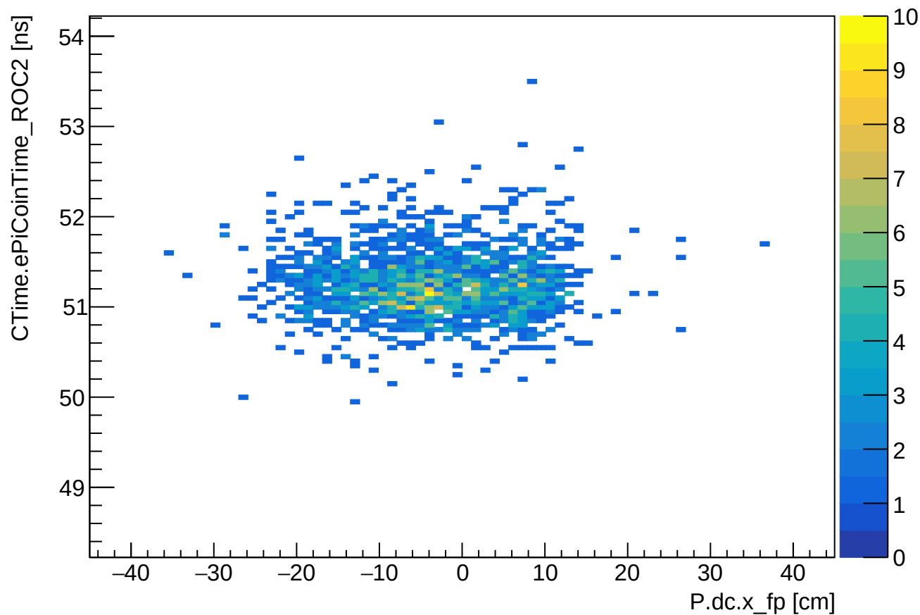
Phase 1 run 24208: CTime (ROC2) vs SHMS xfp
