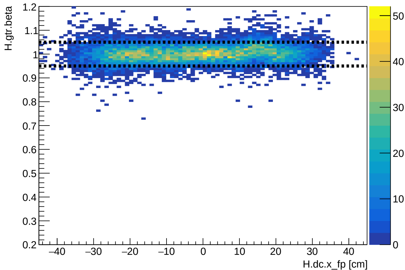
Phase 1 run 24621: HMS beta vs HMS xfp
