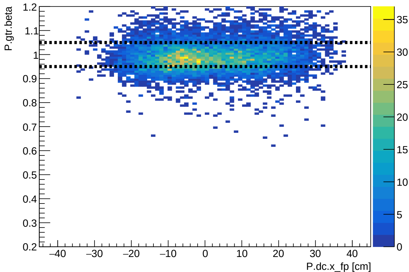
Phase 1 run 24112: SHMS beta vs SHMS xfp
