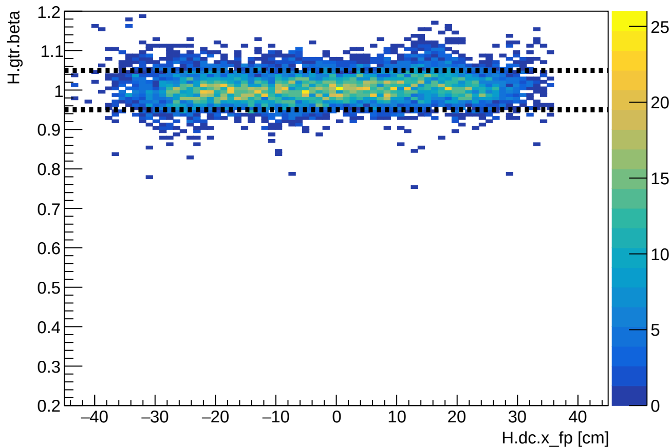
Phase 1 run 24117: HMS beta vs HMS xfp
