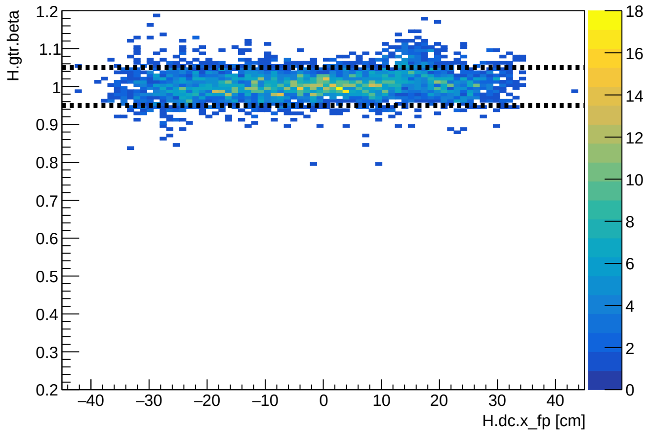
Phase 1 run 24208: HMS beta vs HMS xfp
