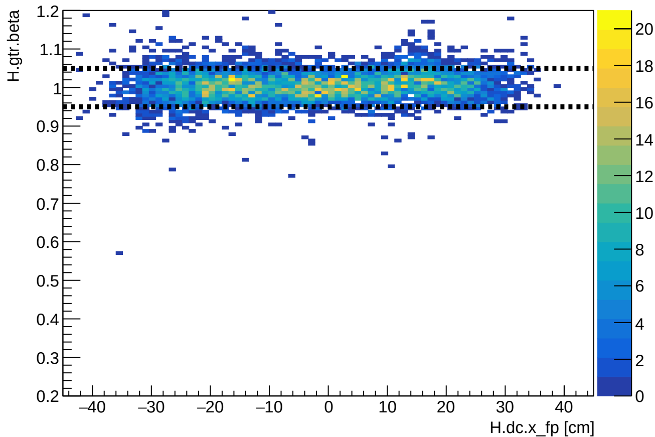
Phase 1 run 24041: HMS beta vs HMS xfp
