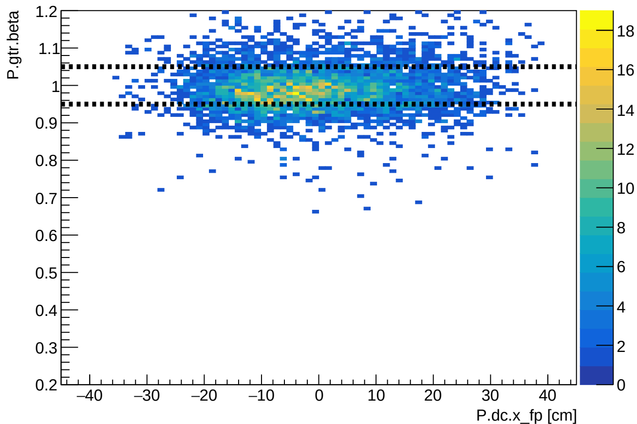
Phase 1 run 24041: SHMS beta vs SHMS xfp
