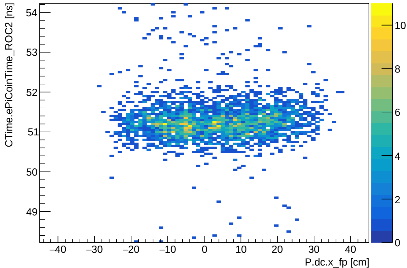
Phase 1 run 24621: CTime (ROC2) vs SHMS xfp
