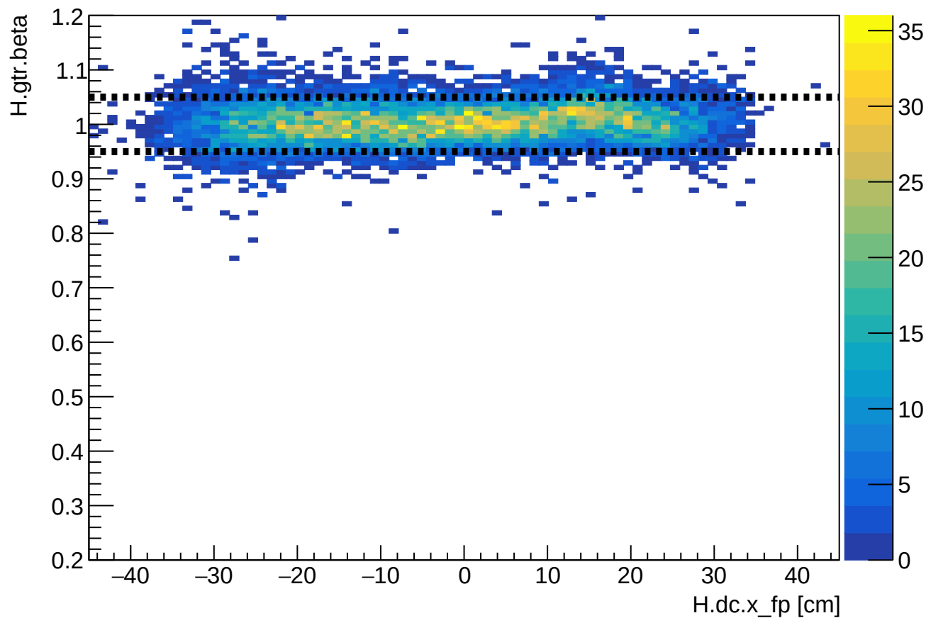
Phase 1 run 24123: HMS beta vs HMS xfp
