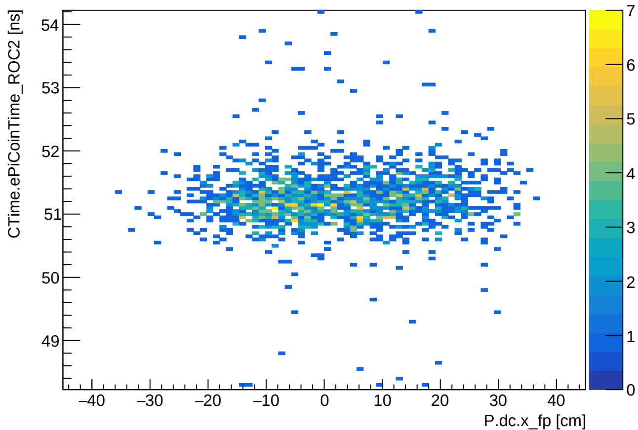
Phase 1 run 24123: CTime (ROC2) vs SHMS xfp
