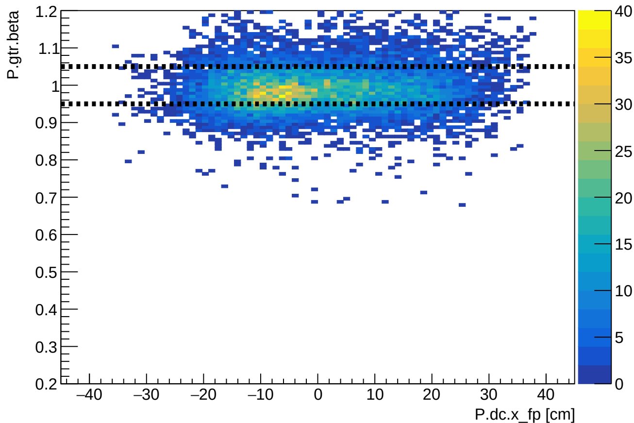
Phase 1 run 24123: SHMS beta vs SHMS xfp
