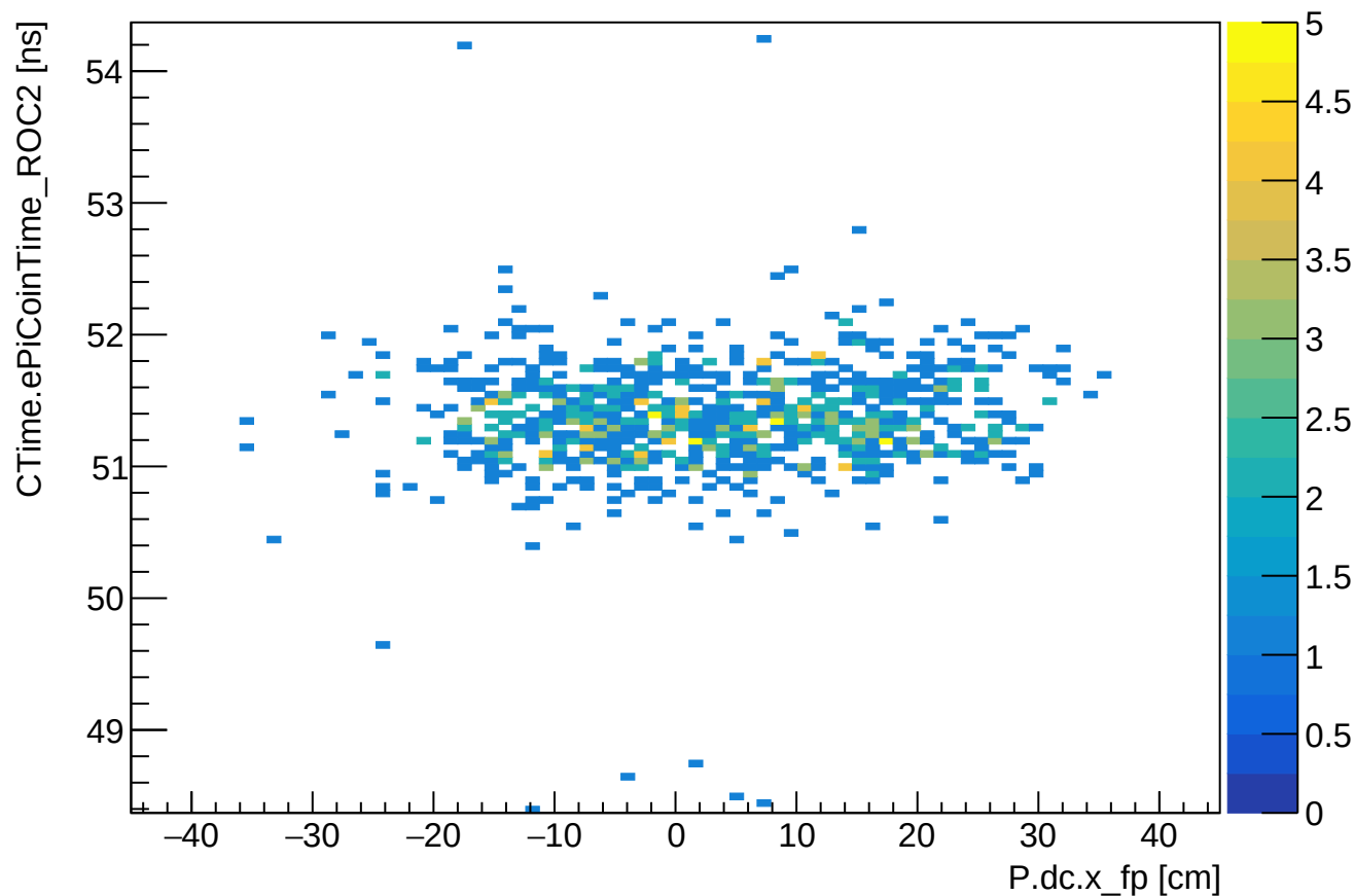
Phase 1 run 24040: CTime (ROC2) vs SHMS xfp
