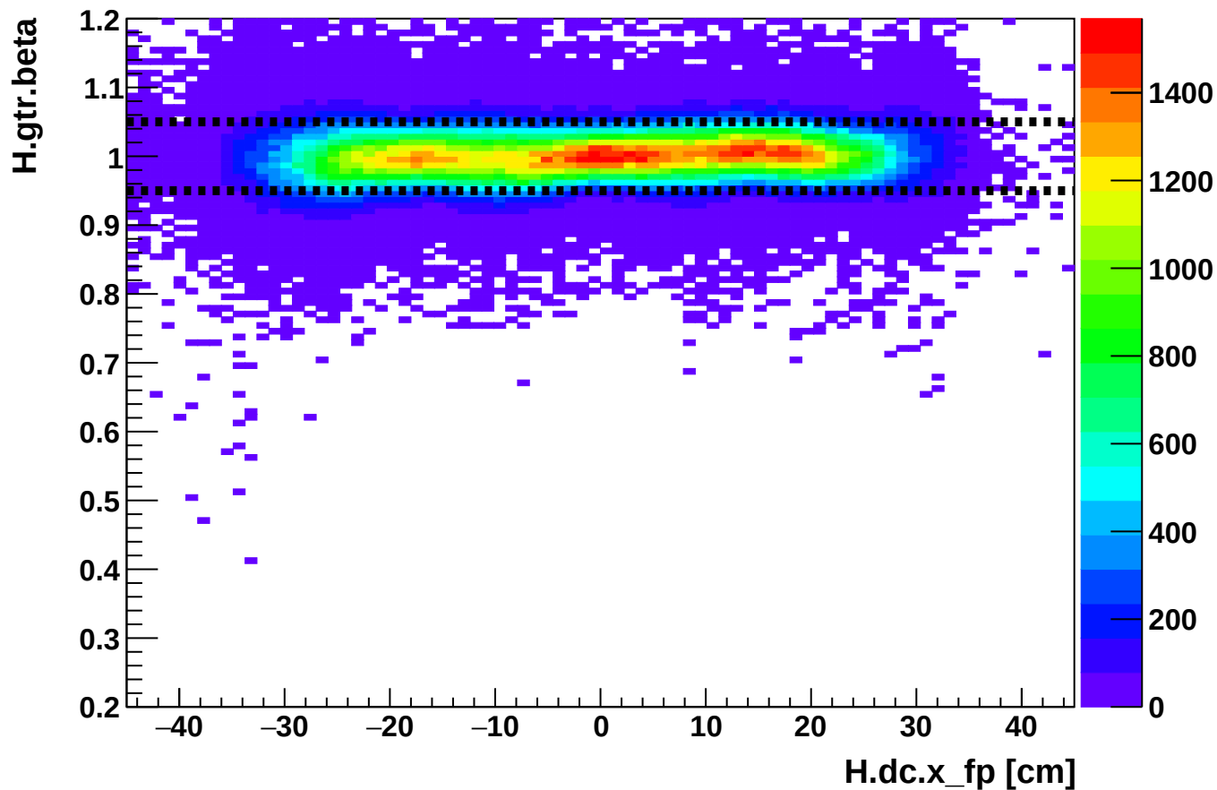
Phase 1 run 24900: HMS beta vs HMS xfp
