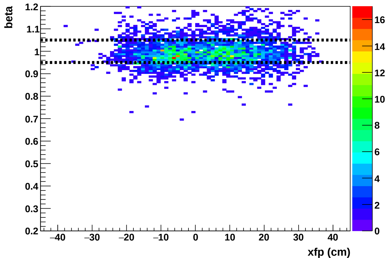
Phase 2 run 27237: beta vs xfp (SHMS)
