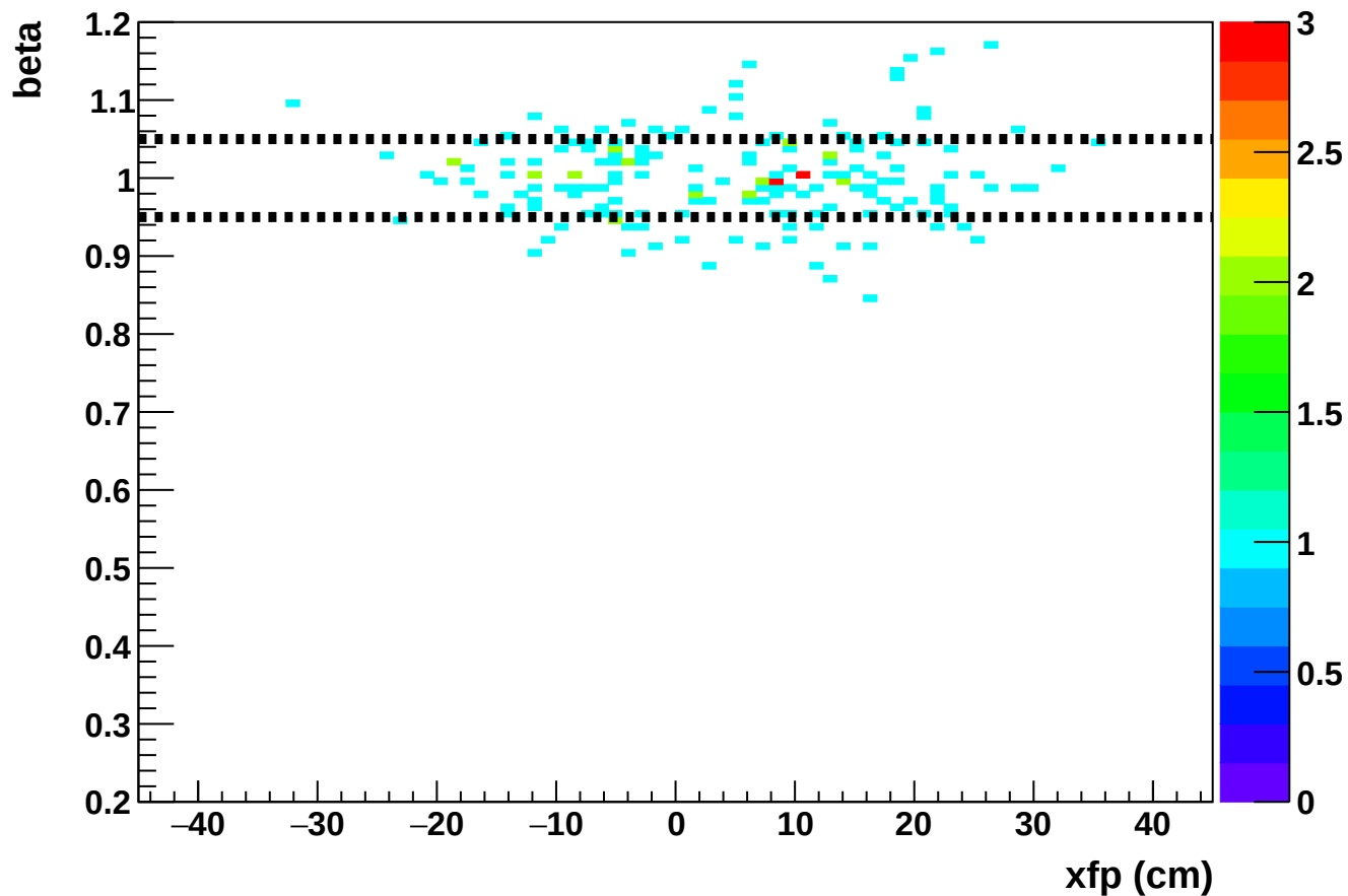
Phase 2 run 27267: beta vs xfp (SHMS)
