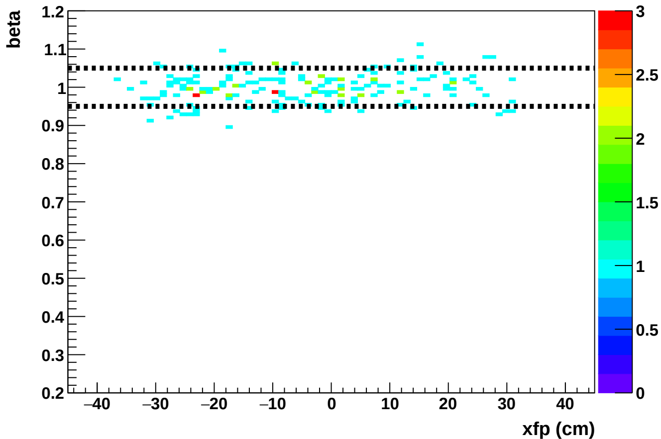
Phase 2 run 27266: beta vs xfp (HMS)
