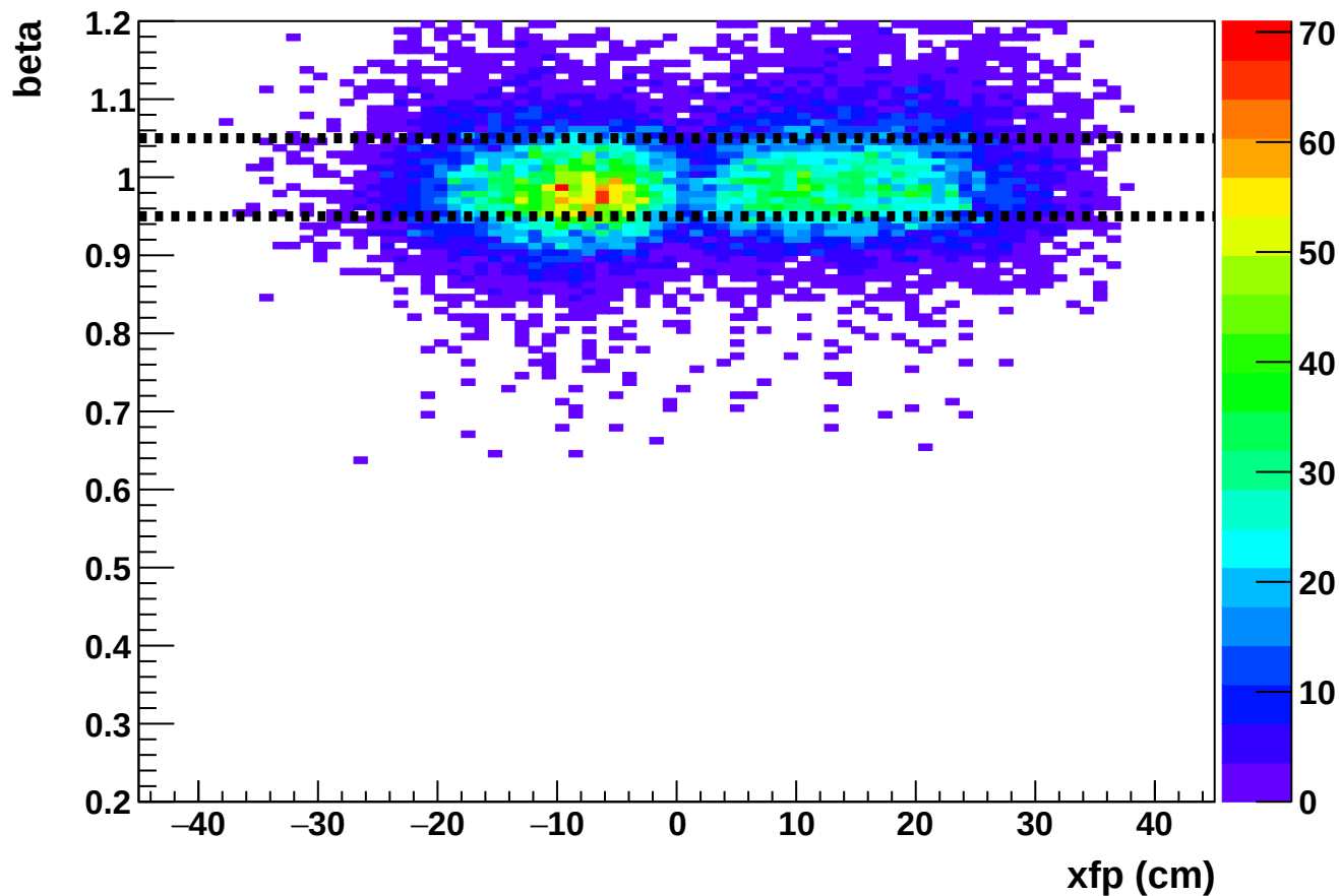
Phase 2 run 27184: beta vs xfp (SHMS)
