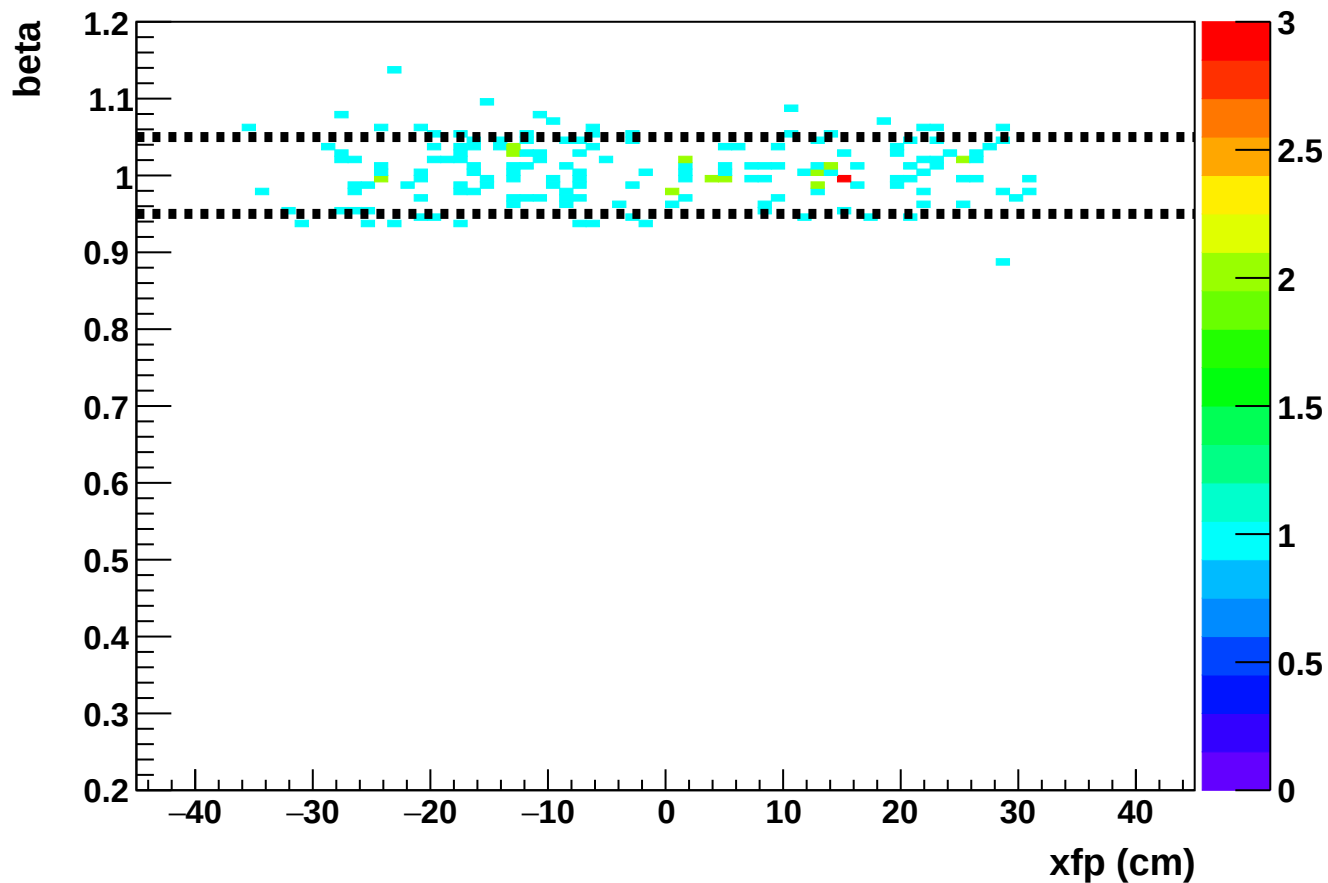
Phase 2 run 27267: beta vs xfp (HMS)
