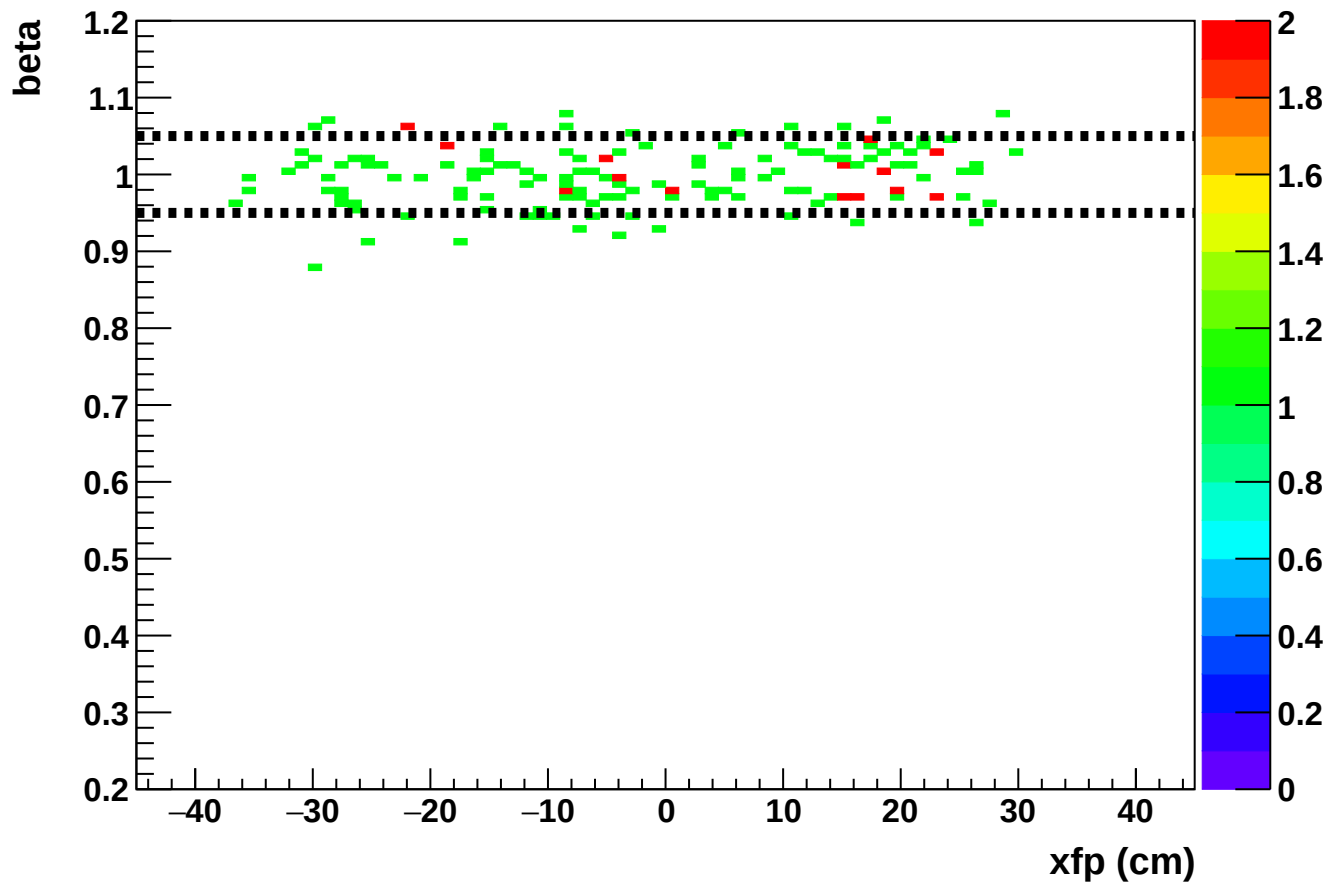
Phase 2 run 27321: beta vs xfp (HMS)
