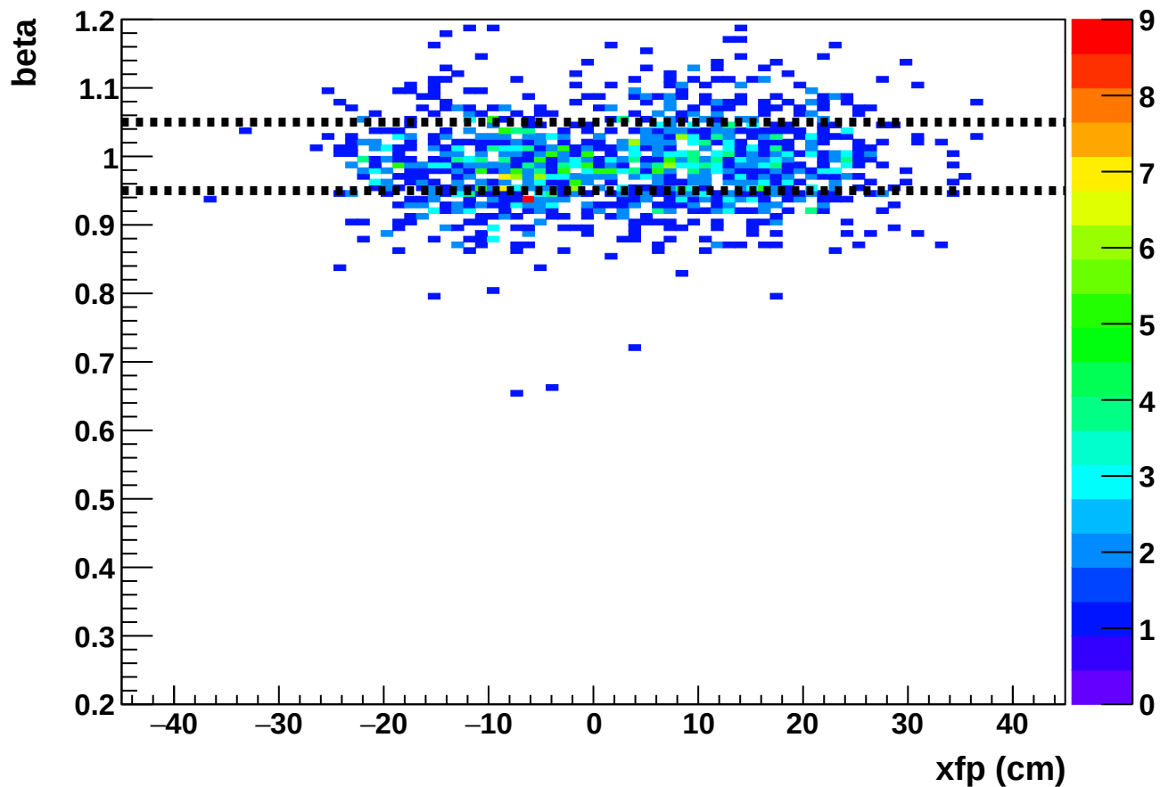
Phase 2 run 27280: beta vs xfp (SHMS)
