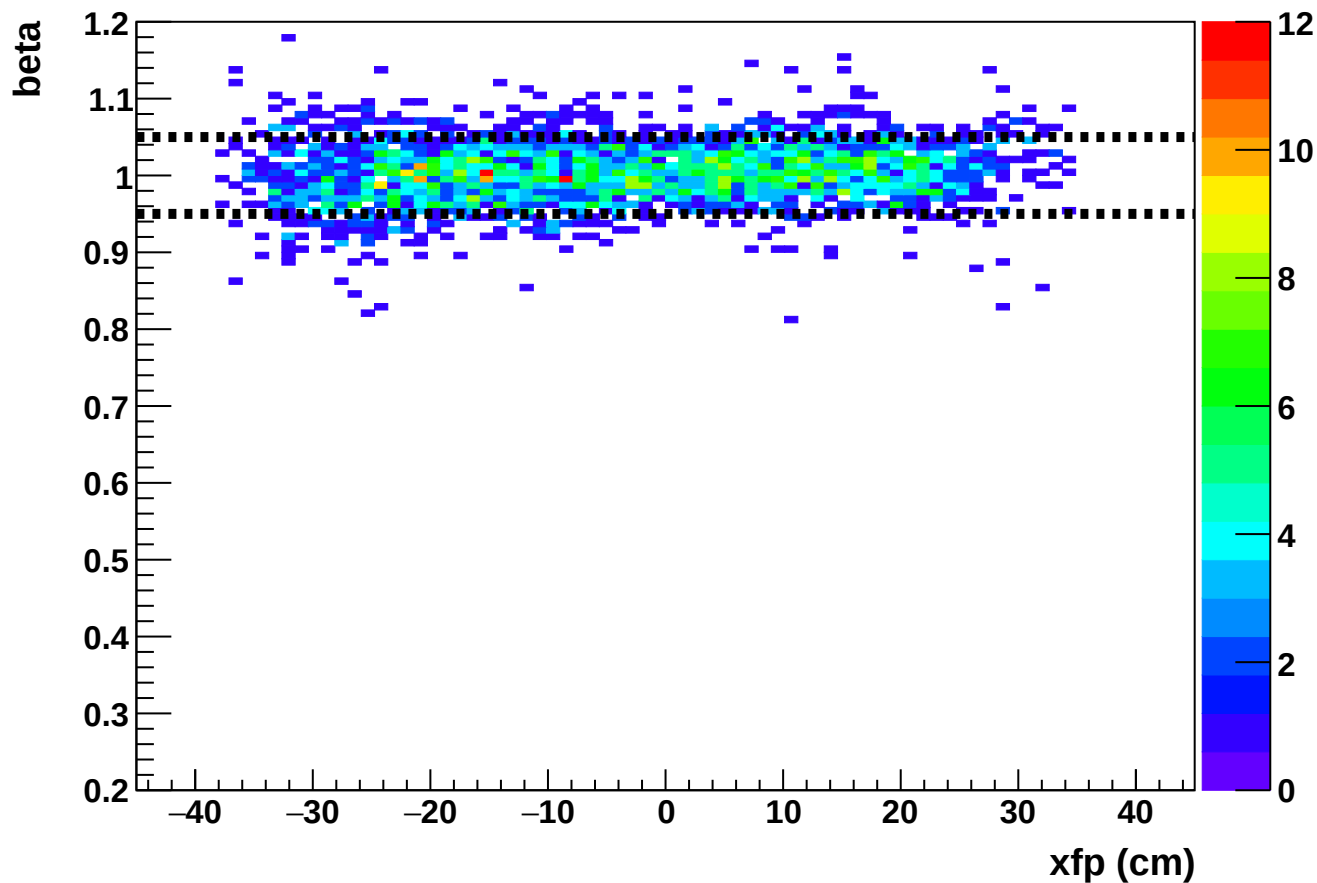
Phase 2 run 27213: beta vs xfp (HMS)
