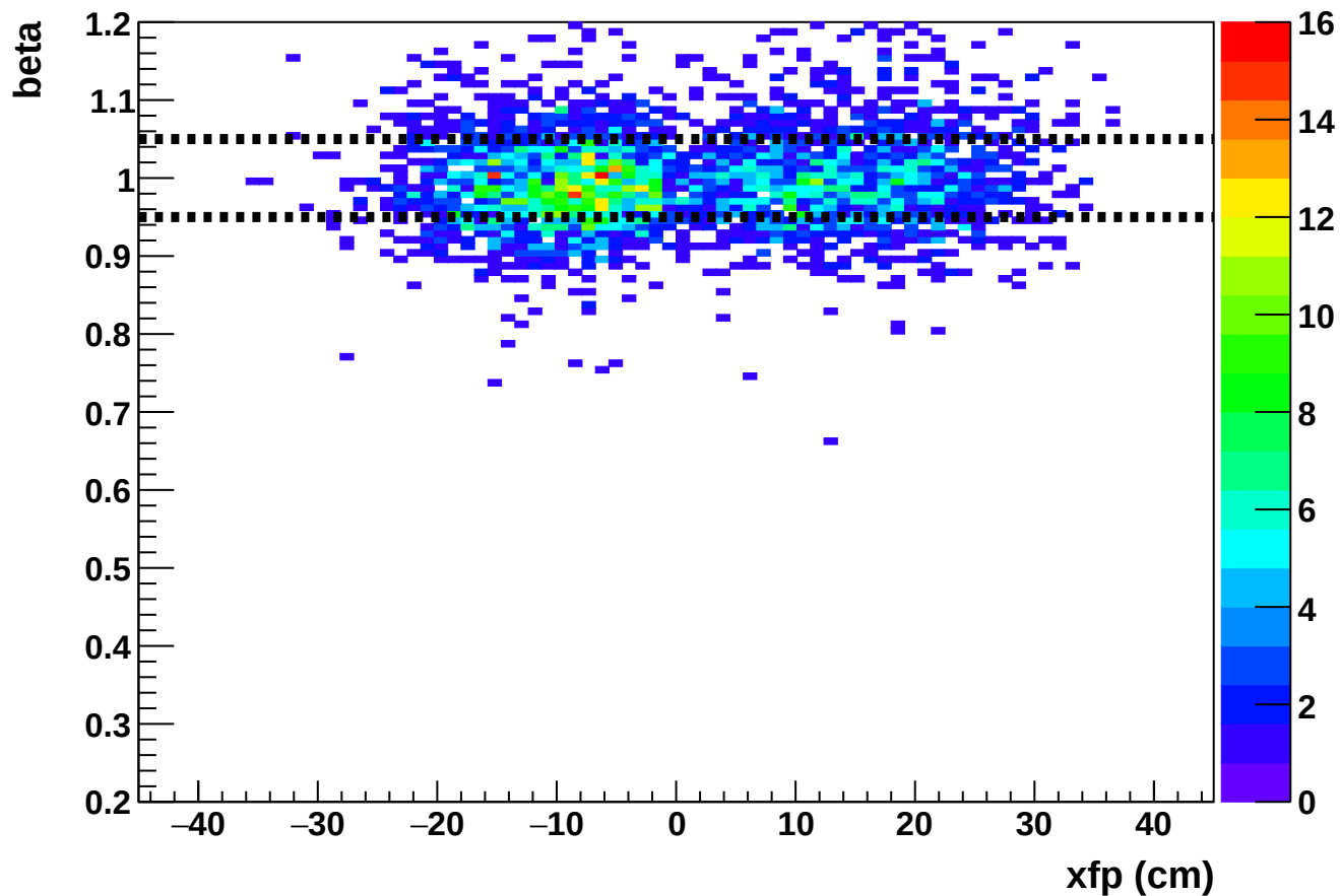
Phase 2 run 27187: beta vs xfp (SHMS)
