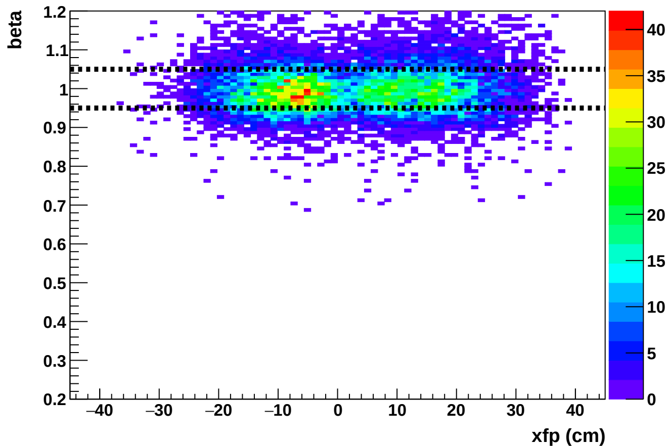
Phase 2 run 27124: beta vs xfp (SHMS)
