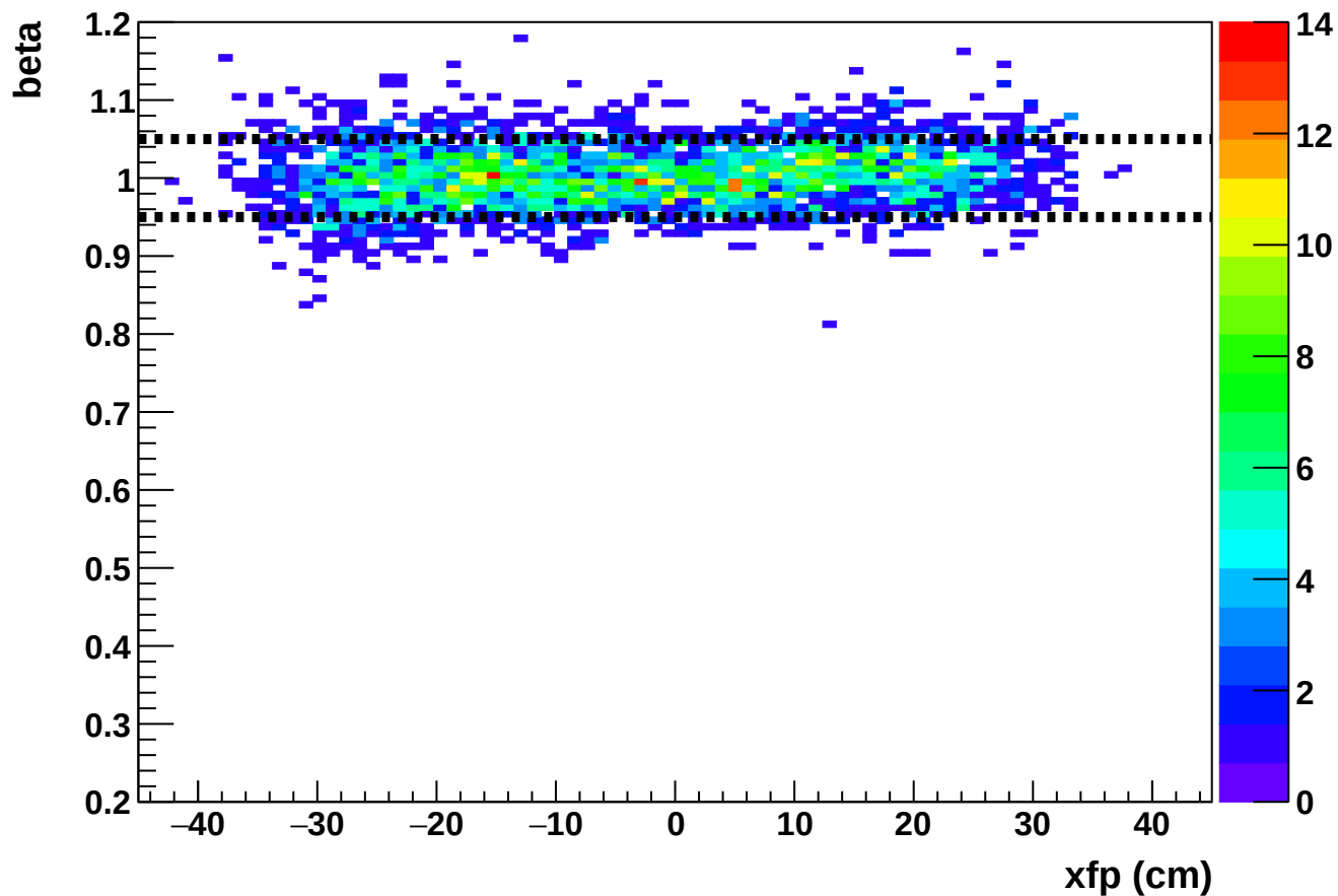
Phase 2 run 27314: beta vs xfp (HMS)
