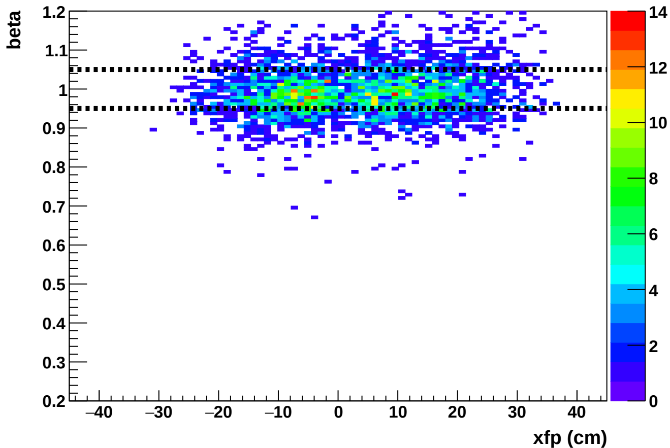
Phase 2 run 27242: beta vs xfp (SHMS)
