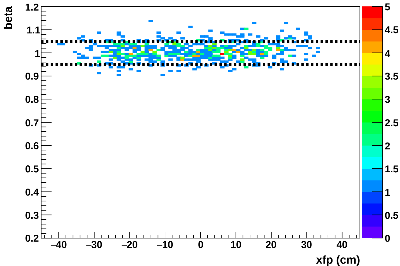
Phase 2 run 27160: beta vs xfp (HMS)
