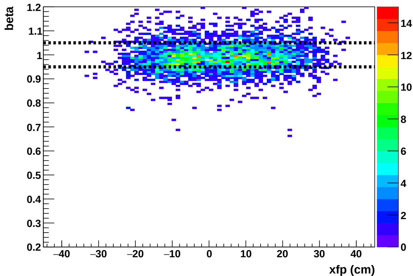
Phase 2 run 27311: beta vs xfp (SHMS)
