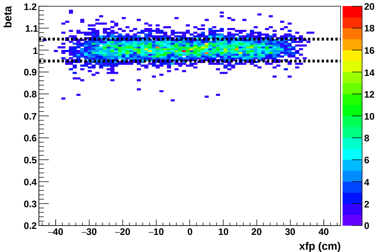
Phase 2 run 27133: beta vs xfp (HMS)
