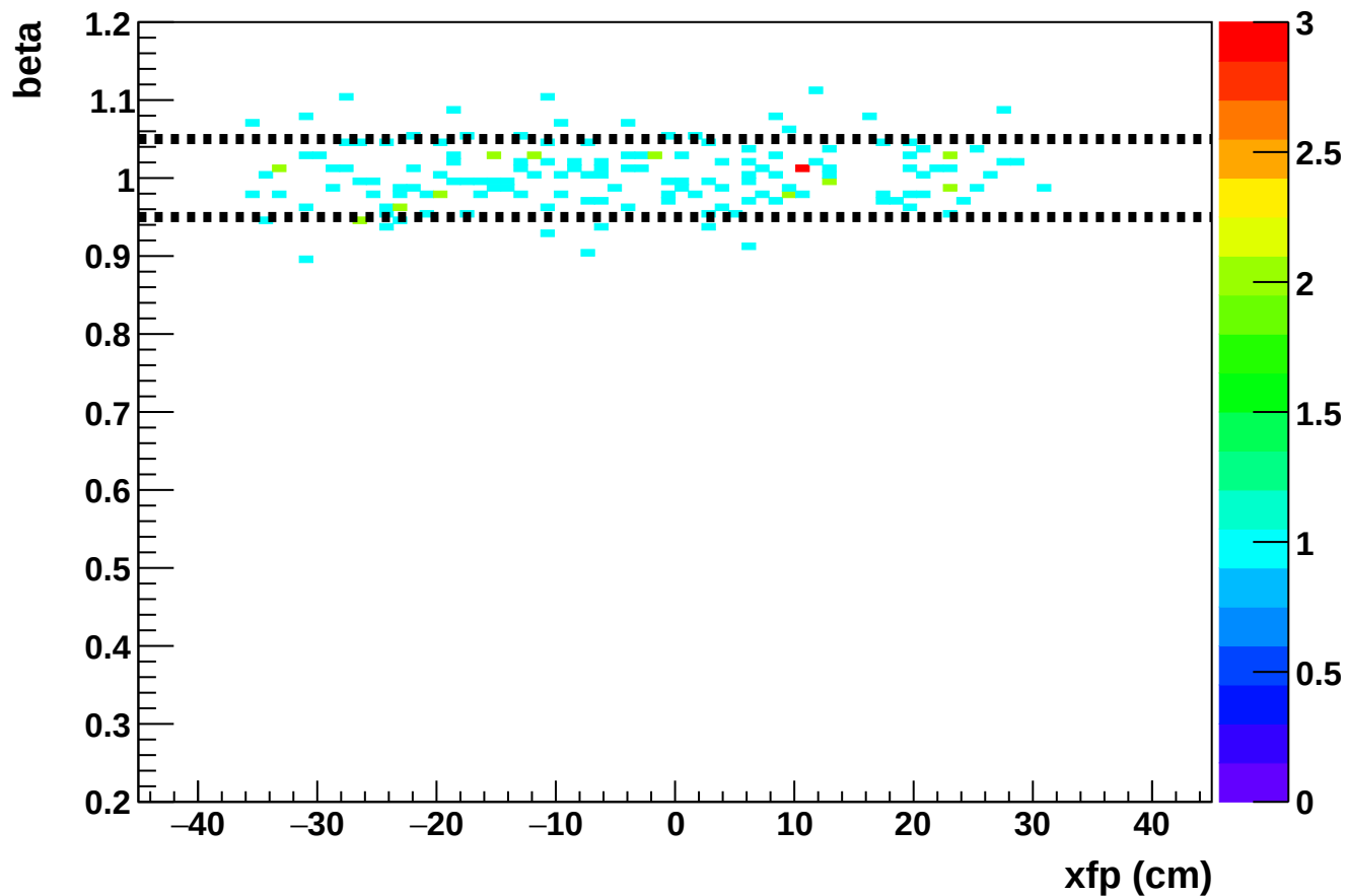
Phase 2 run 27322: beta vs xfp (HMS)
