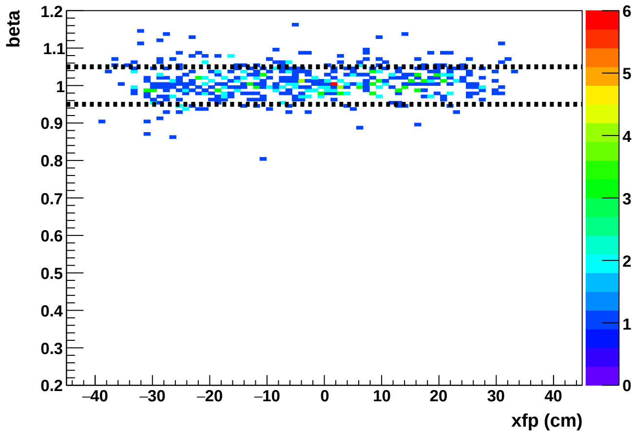
Phase 2 run 27199: beta vs xfp (HMS)
