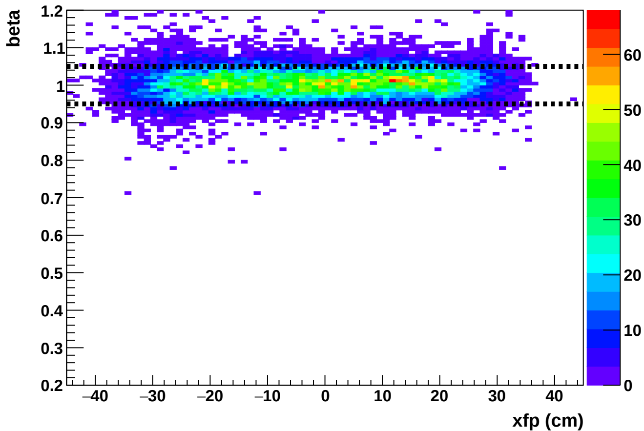
Phase 2 run 27167: beta vs xfp (HMS)
