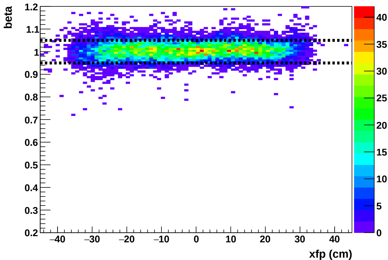
Phase 2 run 27130: beta vs xfp (HMS)
