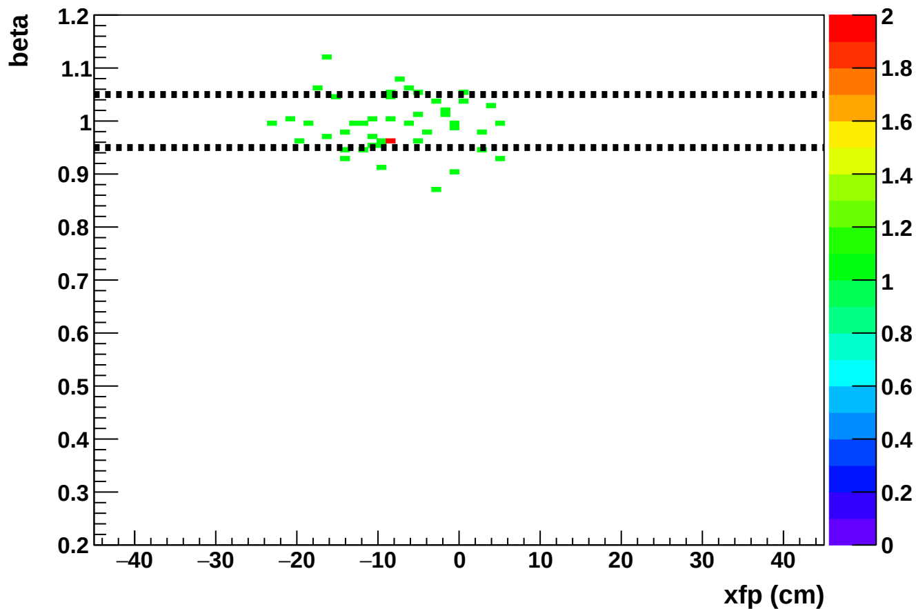
Phase 2 run 27200: beta vs xfp (SHMS)
