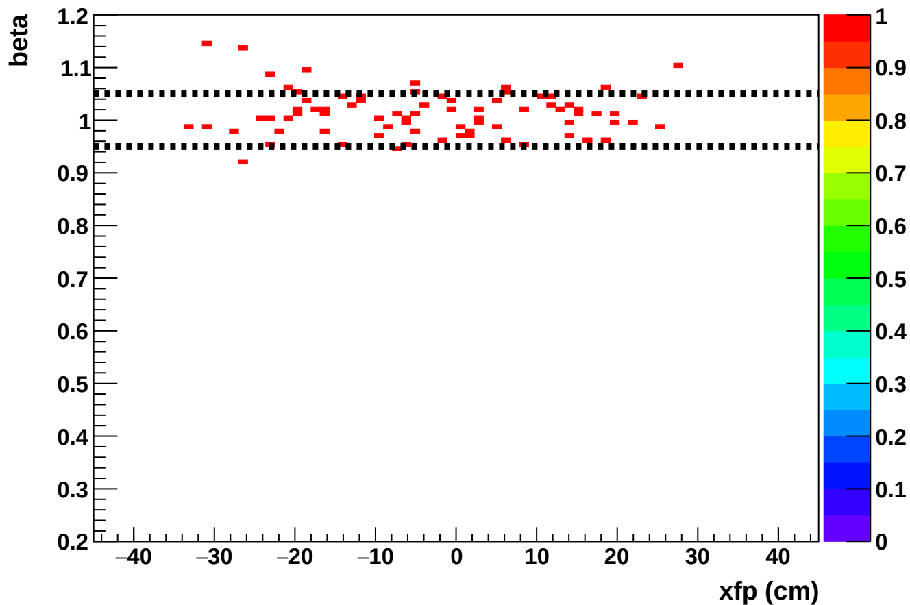
Phase 2 run 27396: beta vs xfp (HMS)
