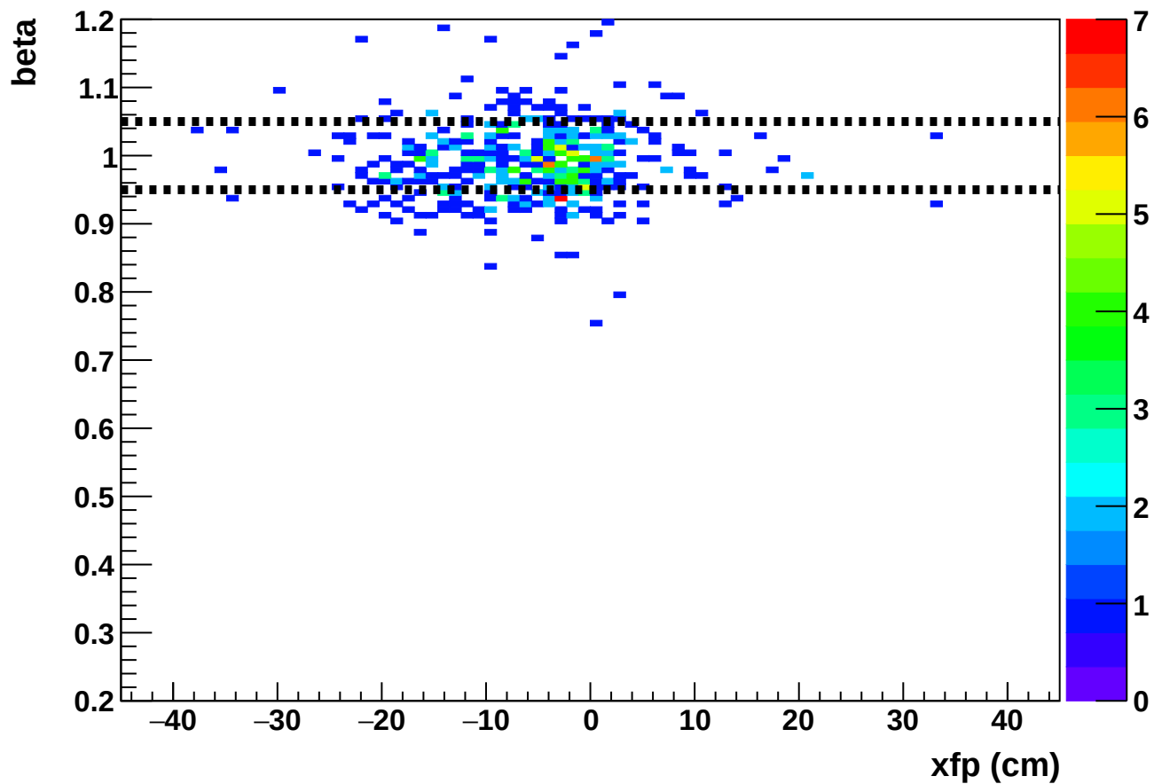
Phase 2 run 27199: beta vs xfp (SHMS)
