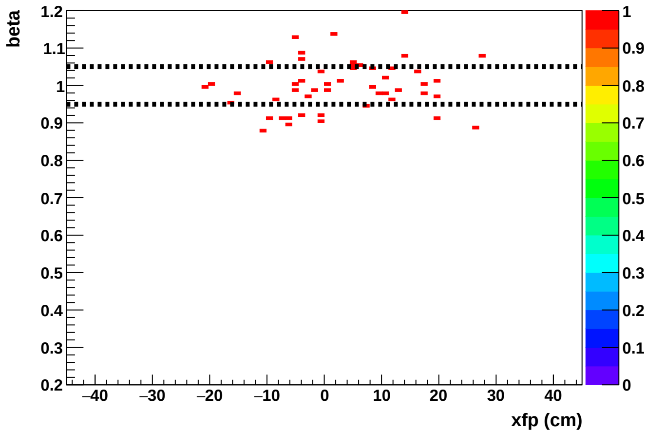
Phase 2 run 27376: beta vs xfp (SHMS)
