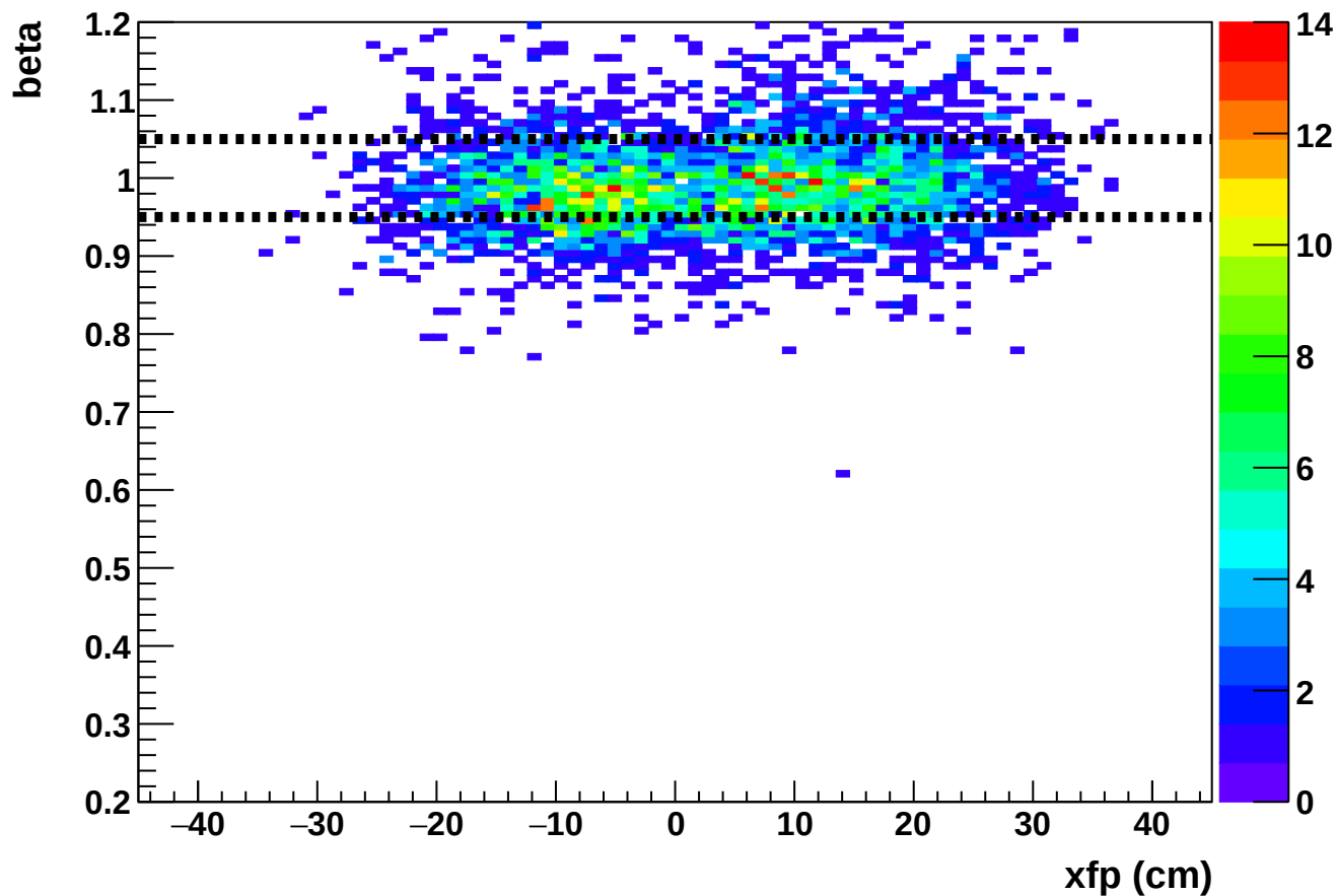
Phase 2 run 27250: beta vs xfp (SHMS)
