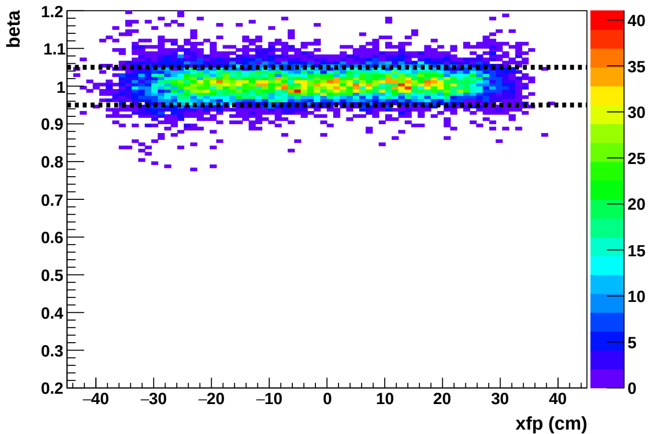
Phase 2 run 27141: beta vs xfp (HMS)
