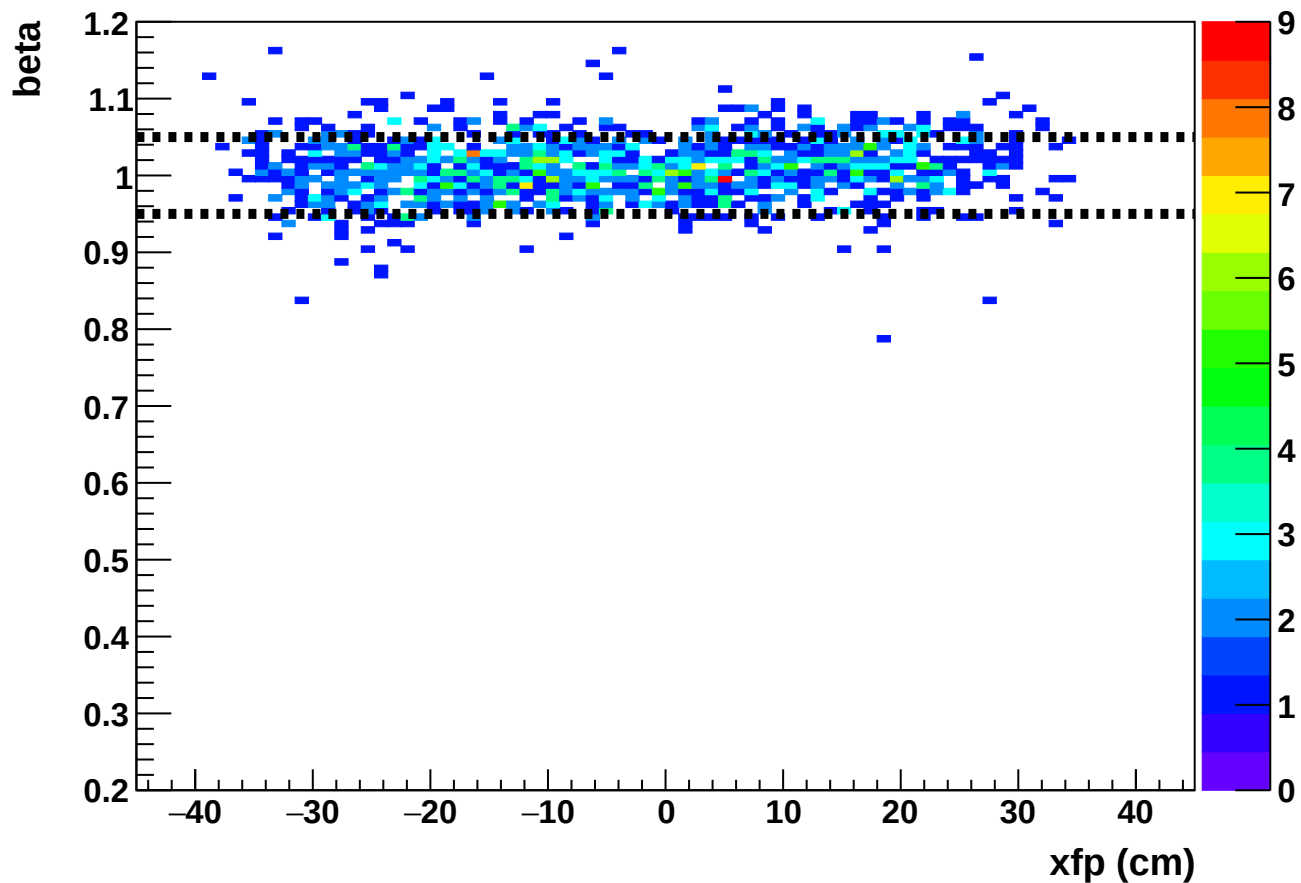
Phase 2 run 27365: beta vs xfp (HMS)
