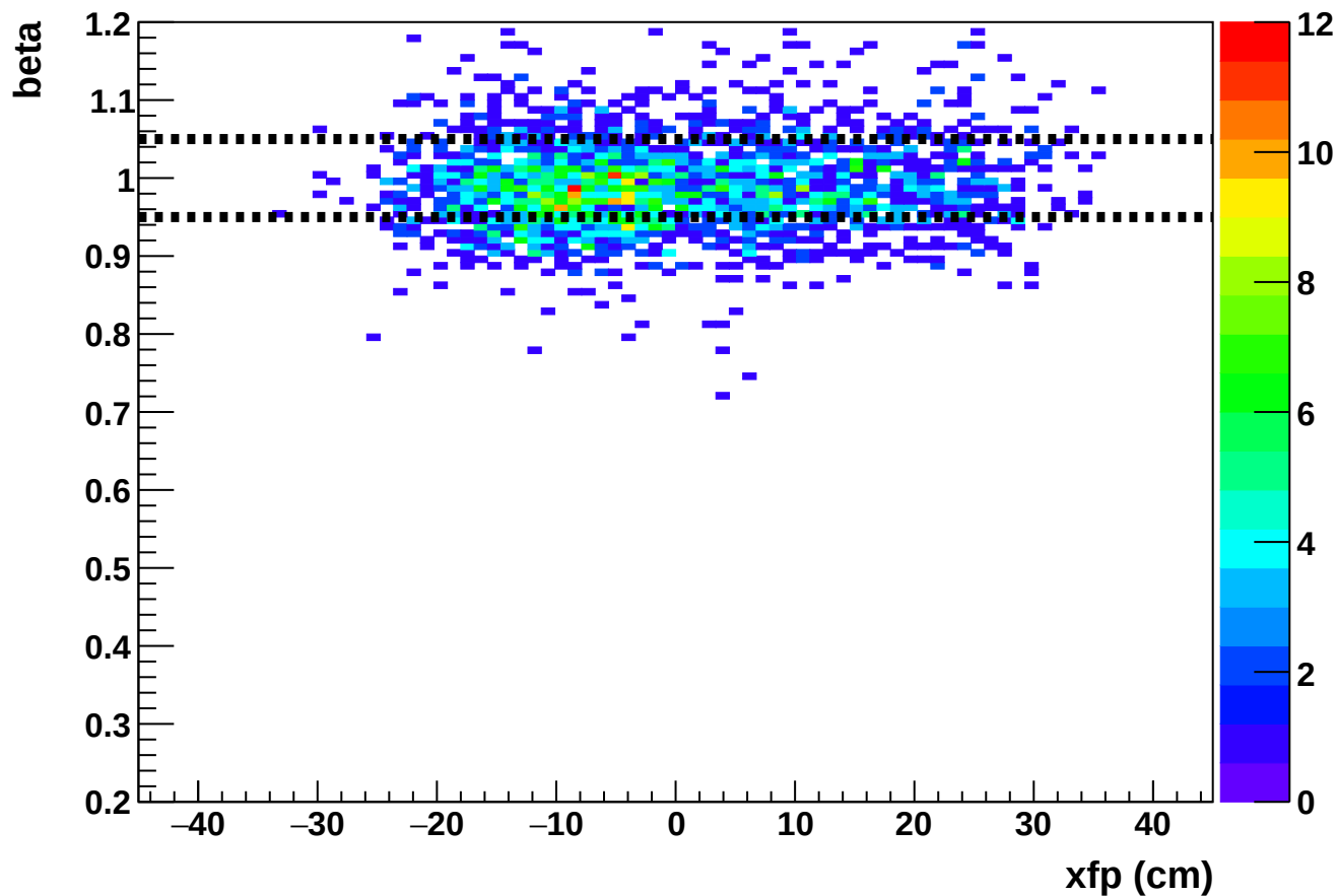
Phase 2 run 27211: beta vs xfp (SHMS)
