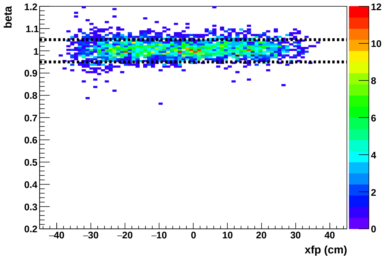
Phase 2 run 27206: beta vs xfp (HMS)
