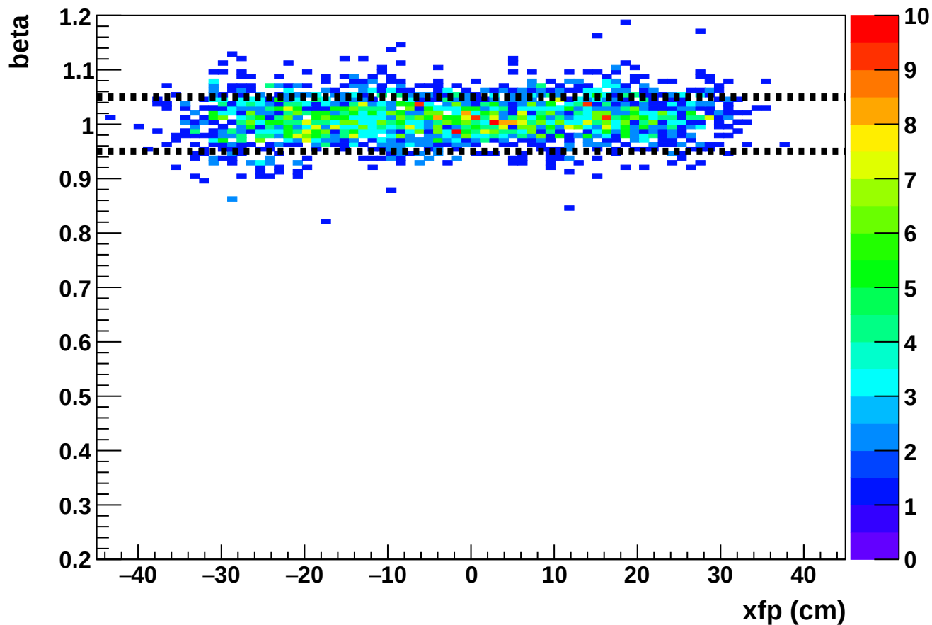
Phase 2 run 27202: beta vs xfp (HMS)
