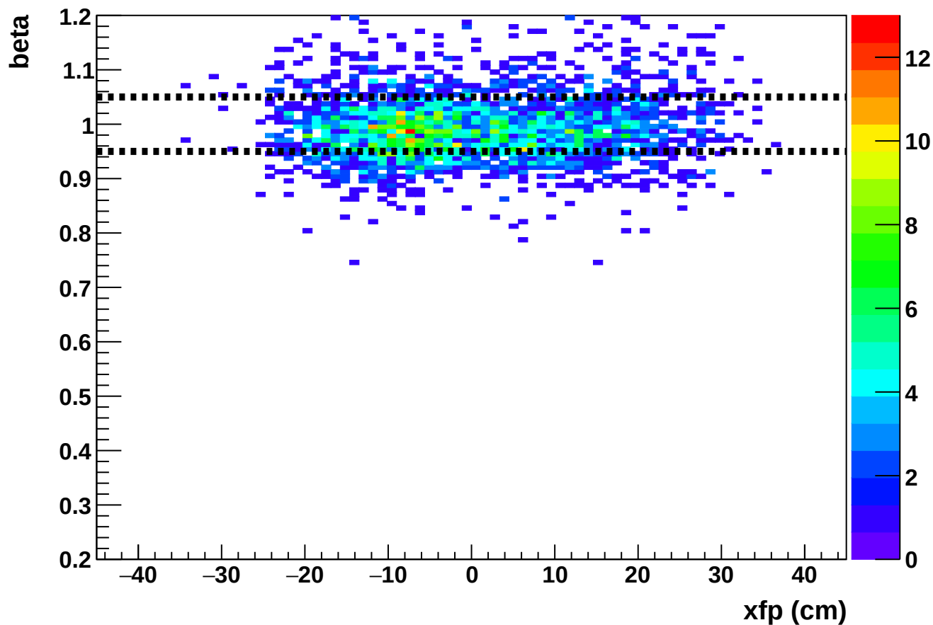
Phase 2 run 27230: beta vs xfp (SHMS)
