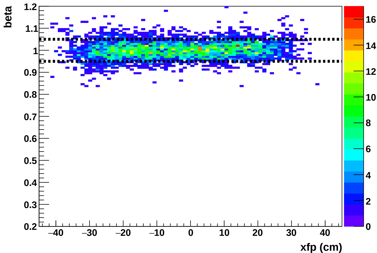
Phase 2 run 27251: beta vs xfp (HMS)
