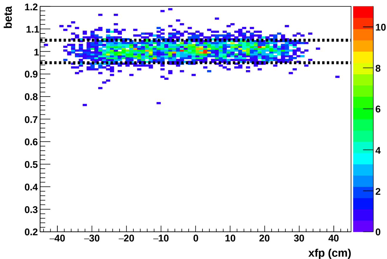
Phase 2 run 27208: beta vs xfp (HMS)
