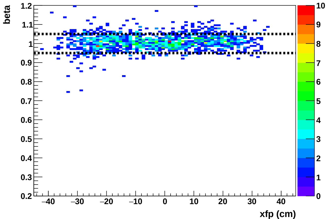
Phase 2 run 27390: beta vs xfp (HMS)
