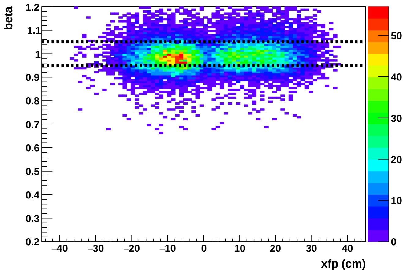
Phase 2 run 27164: beta vs xfp (SHMS)
