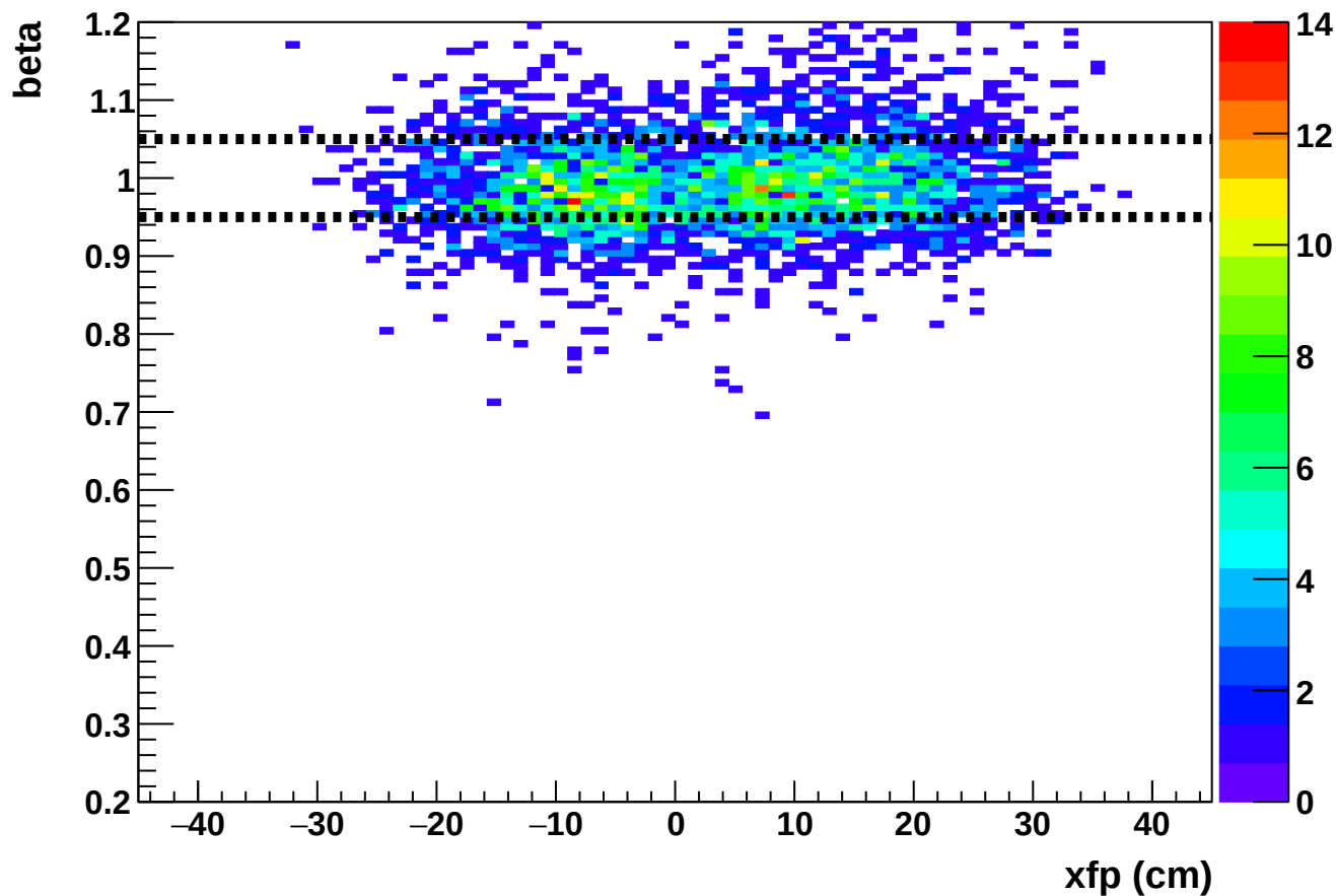
Phase 2 run 27319: beta vs xfp (SHMS)
