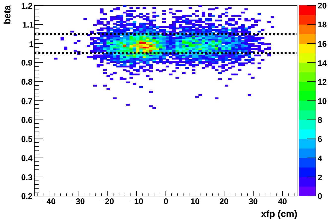
Phase 2 run 27186: beta vs xfp (SHMS)
