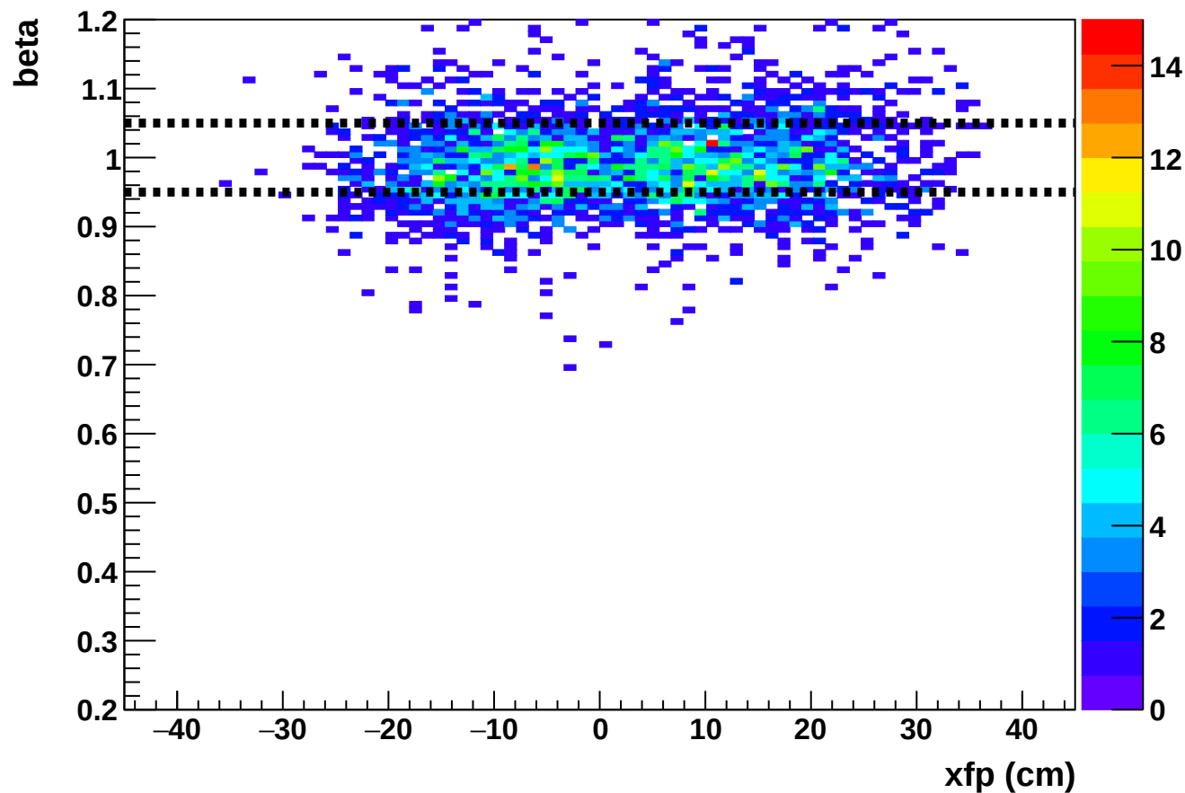
Phase 2 run 27276: beta vs xfp (SHMS)
