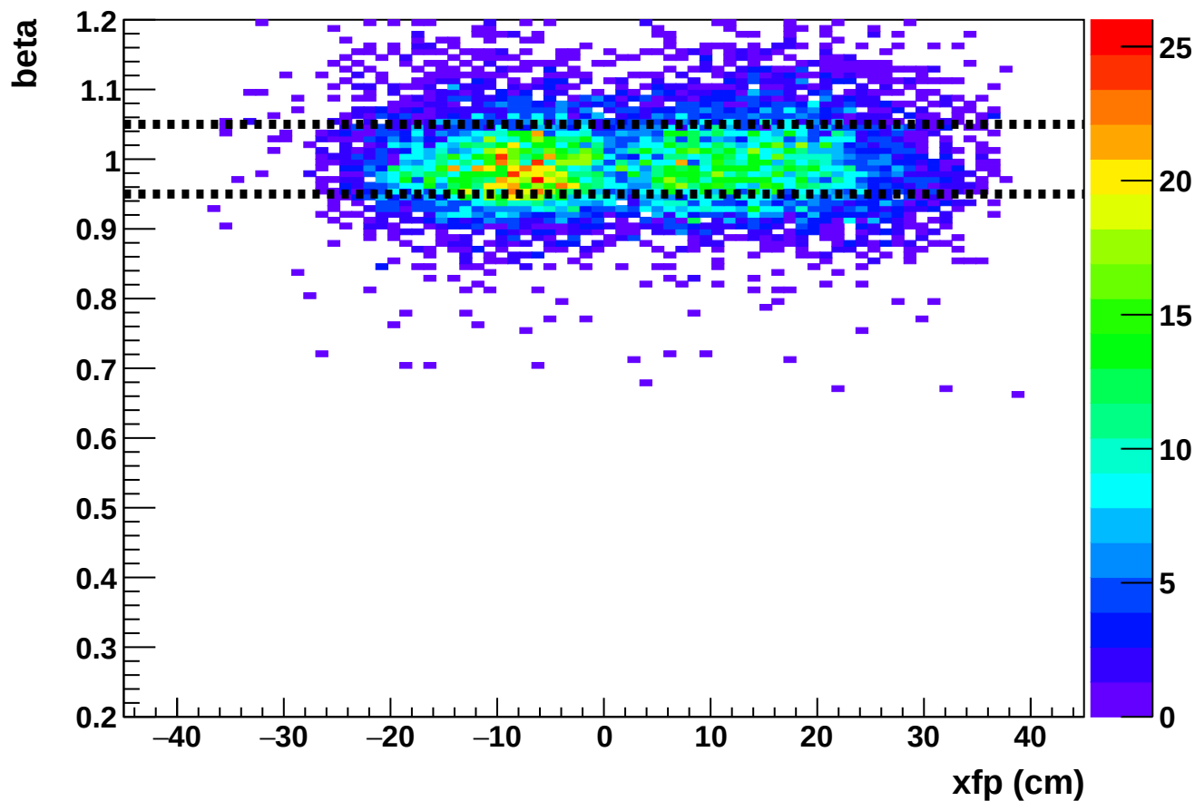
Phase 2 run 27149: beta vs xfp (SHMS)
