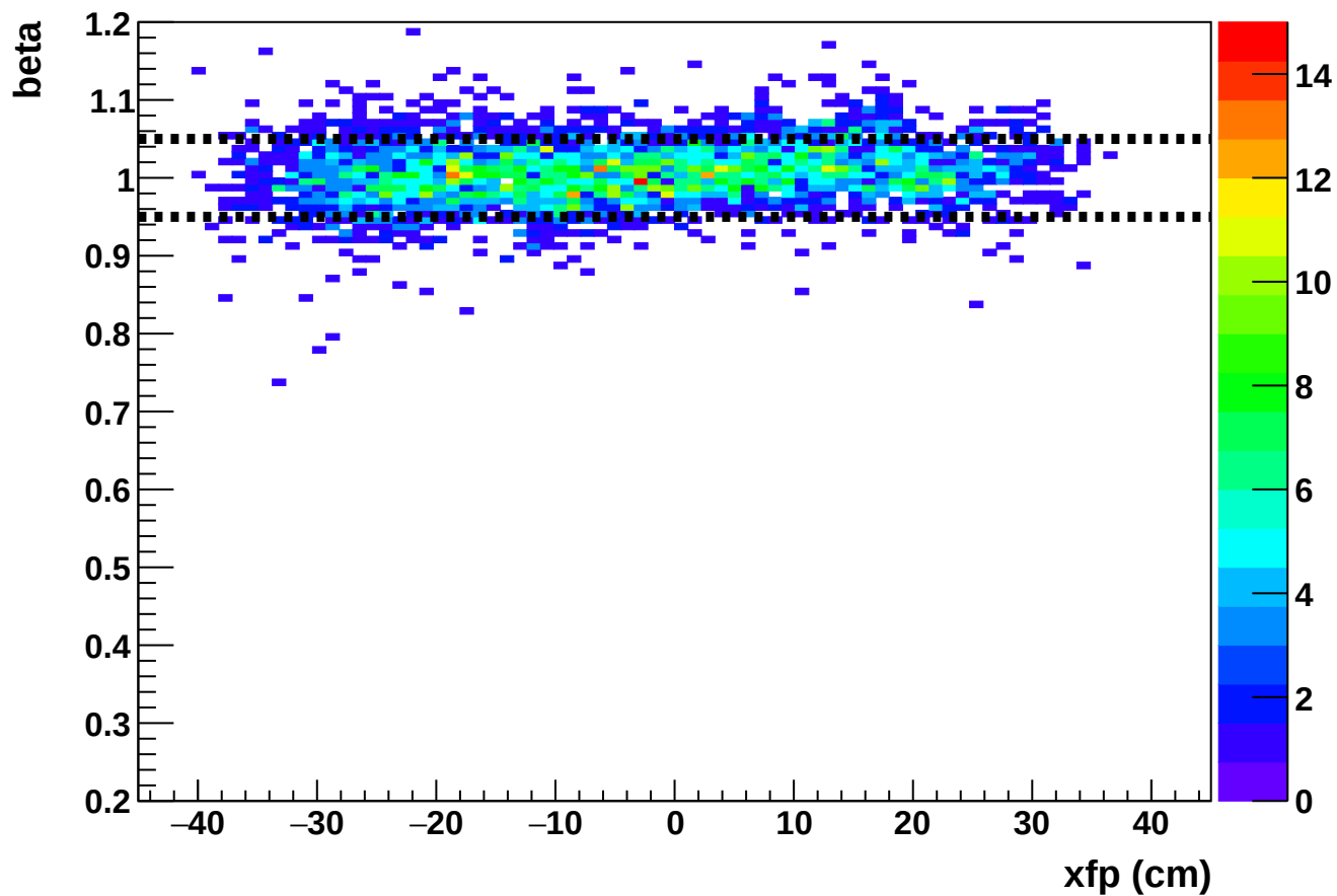
Phase 2 run 27334: beta vs xfp (HMS)
