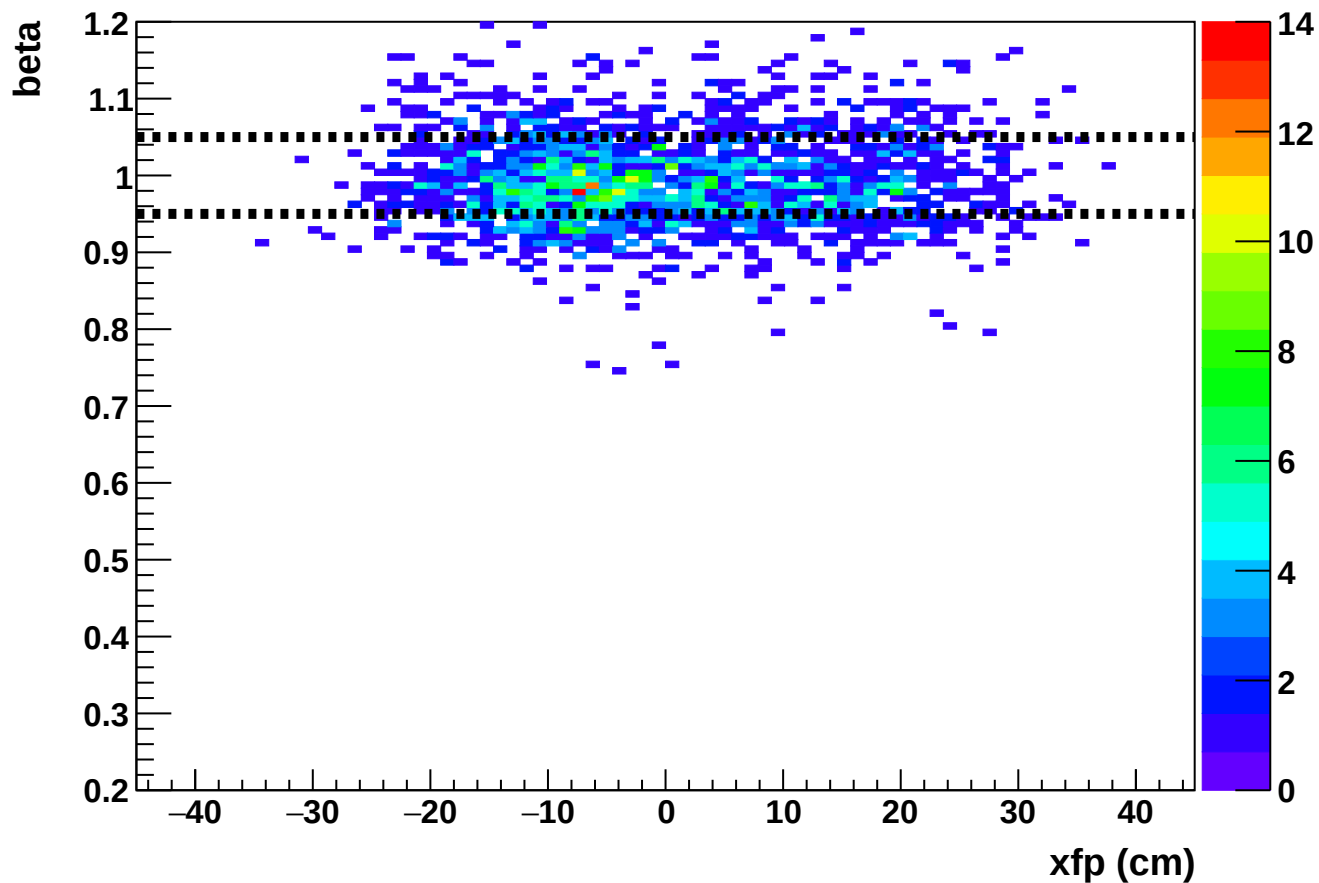
Phase 2 run 27201: beta vs xfp (SHMS)
