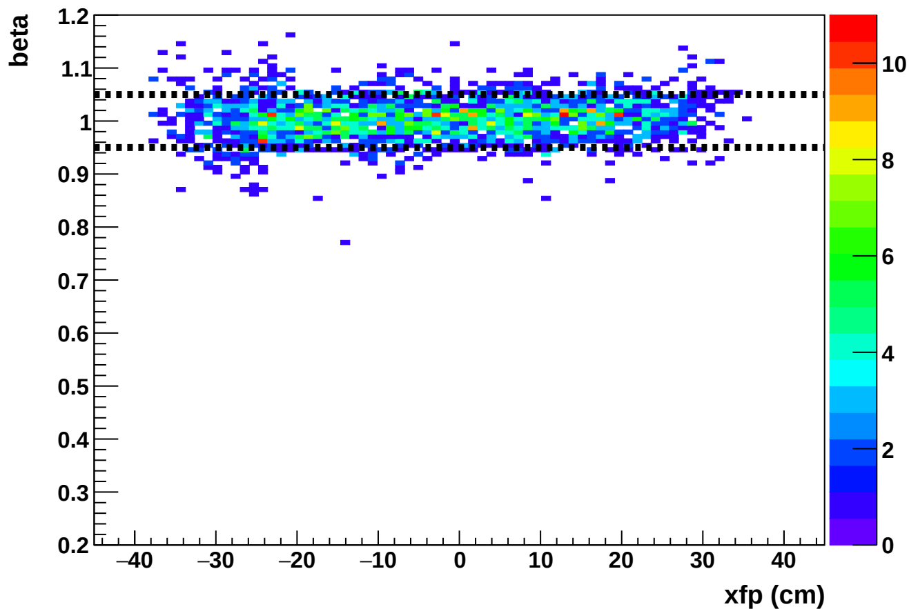
Phase 2 run 27211: beta vs xfp (HMS)
