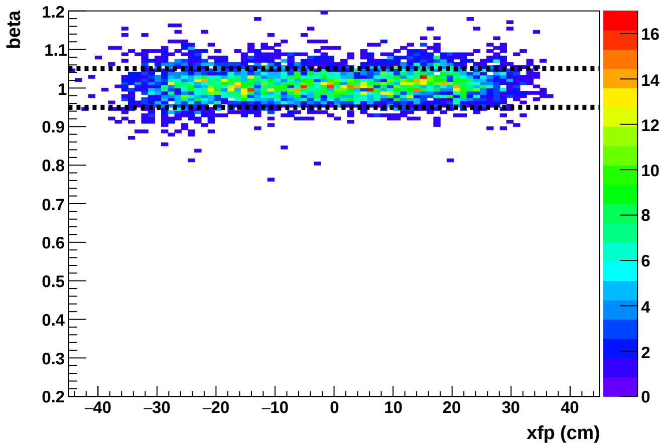
Phase 2 run 27178: beta vs xfp (HMS)
