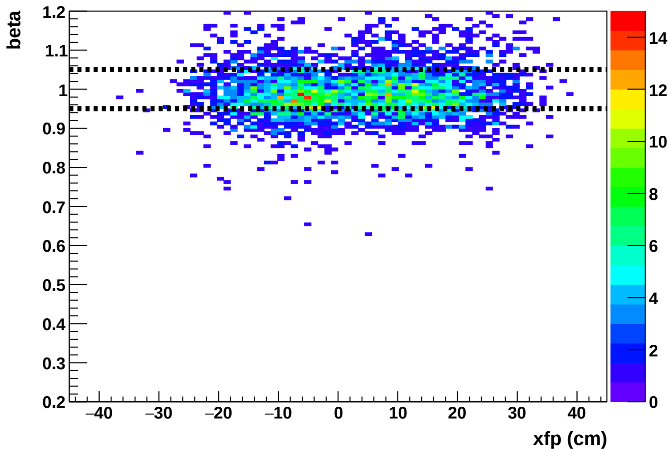
Phase 2 run 27310: beta vs xfp (SHMS)
