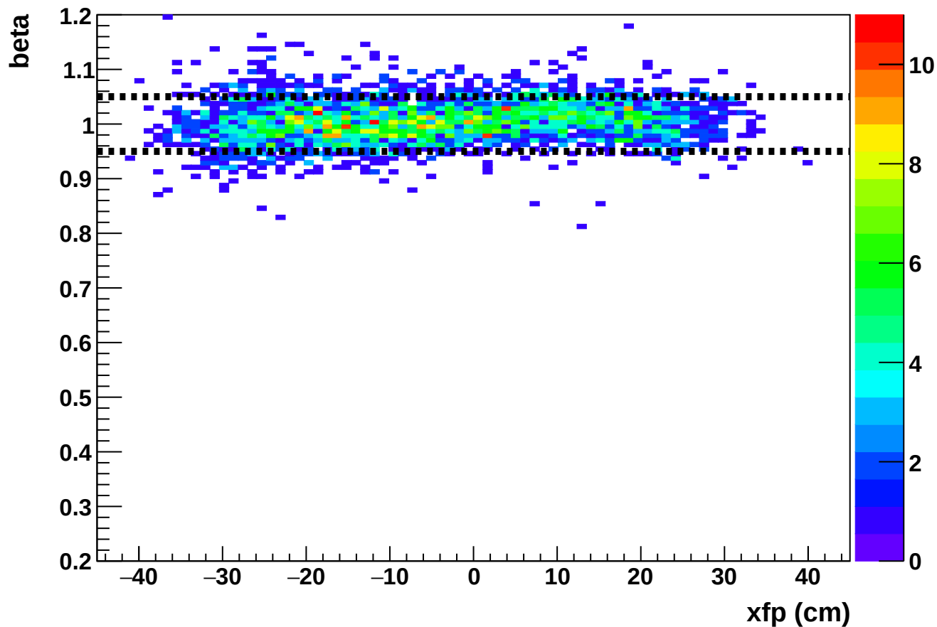
Phase 2 run 27290: beta vs xfp (HMS)
