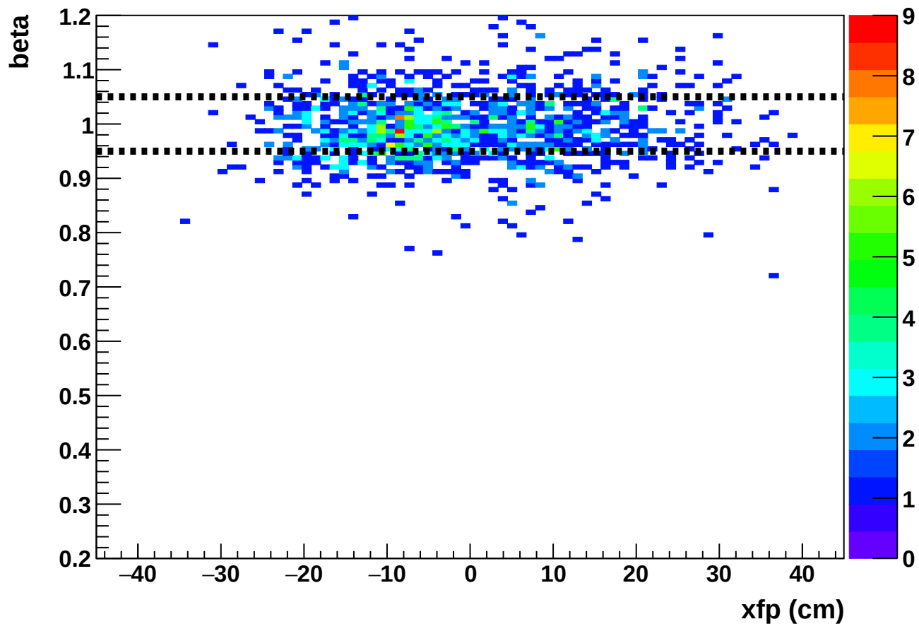
Phase 2 run 27389: beta vs xfp (SHMS)
