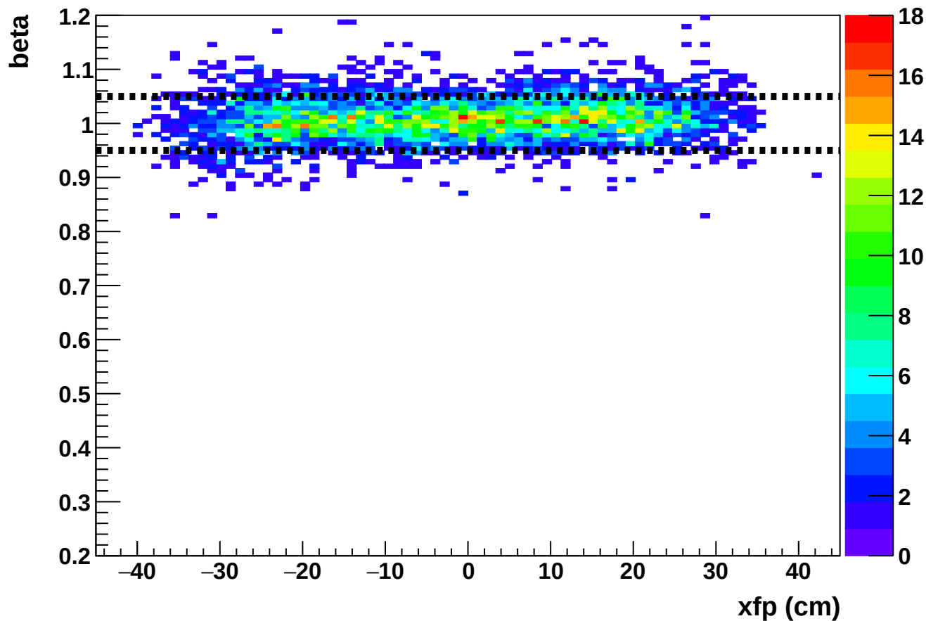
Phase 2 run 27158: beta vs xfp (HMS)
