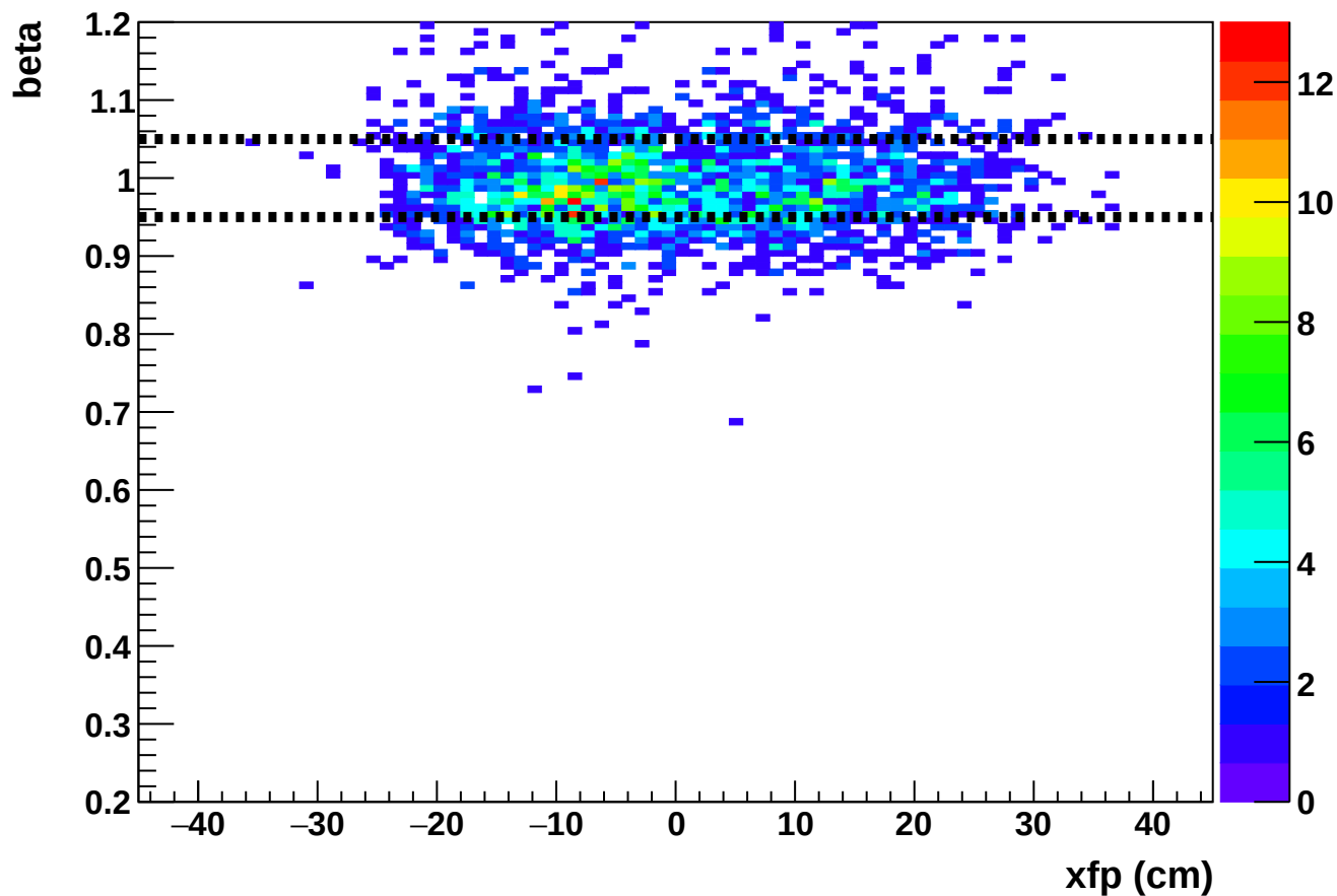
Phase 2 run 27224: beta vs xfp (SHMS)
