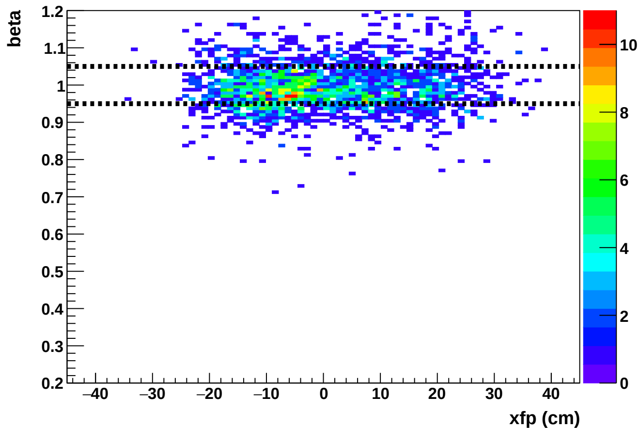
Phase 2 run 27202: beta vs xfp (SHMS)
