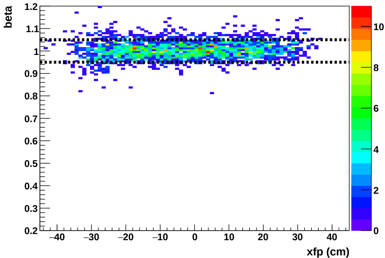
Phase 2 run 27212: beta vs xfp (HMS)
