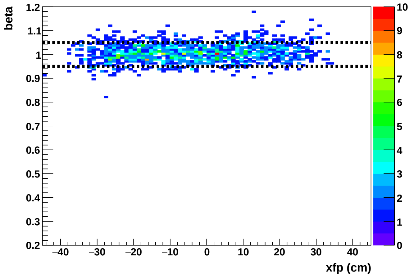
Phase 2 run 27386: beta vs xfp (HMS)
