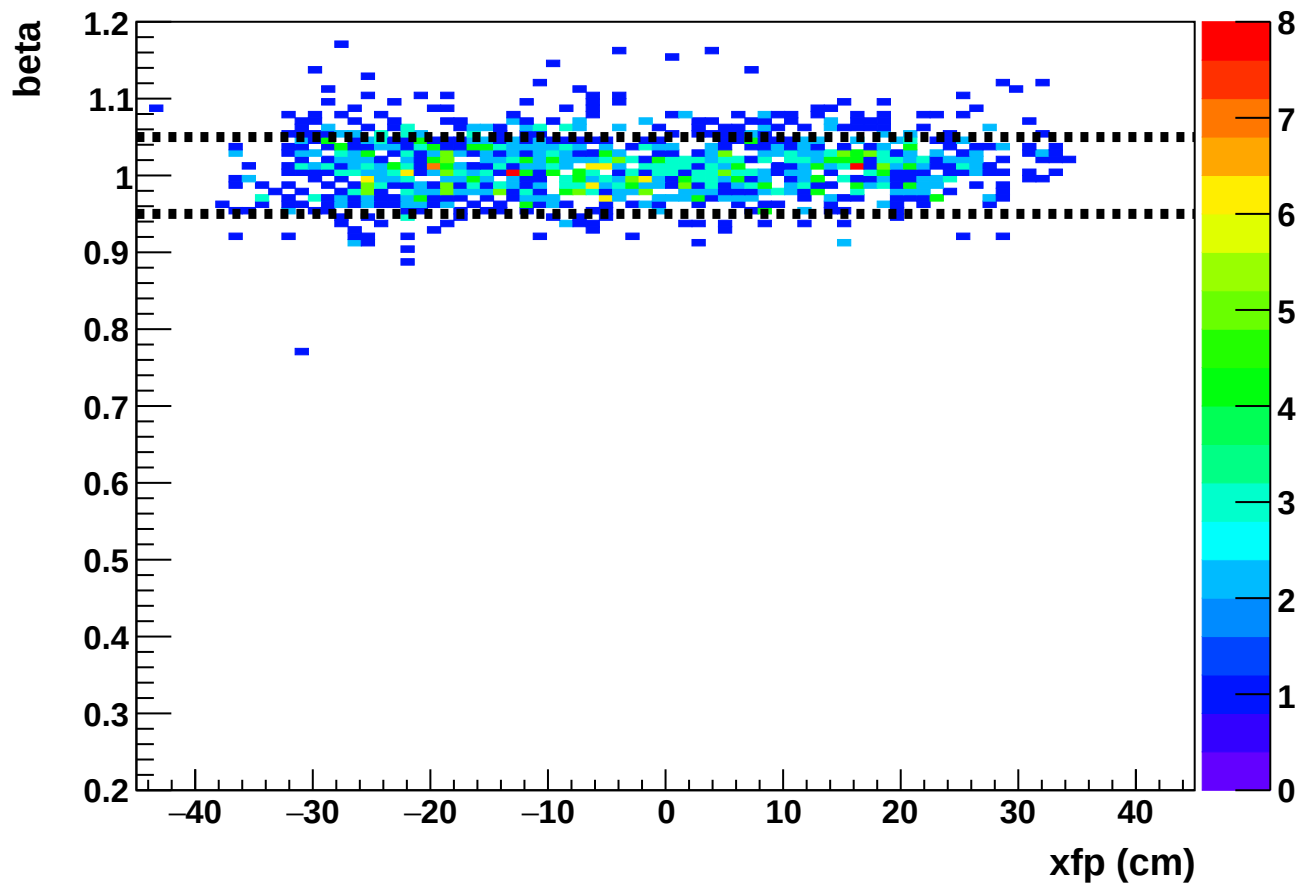
Phase 2 run 27384: beta vs xfp (HMS)
