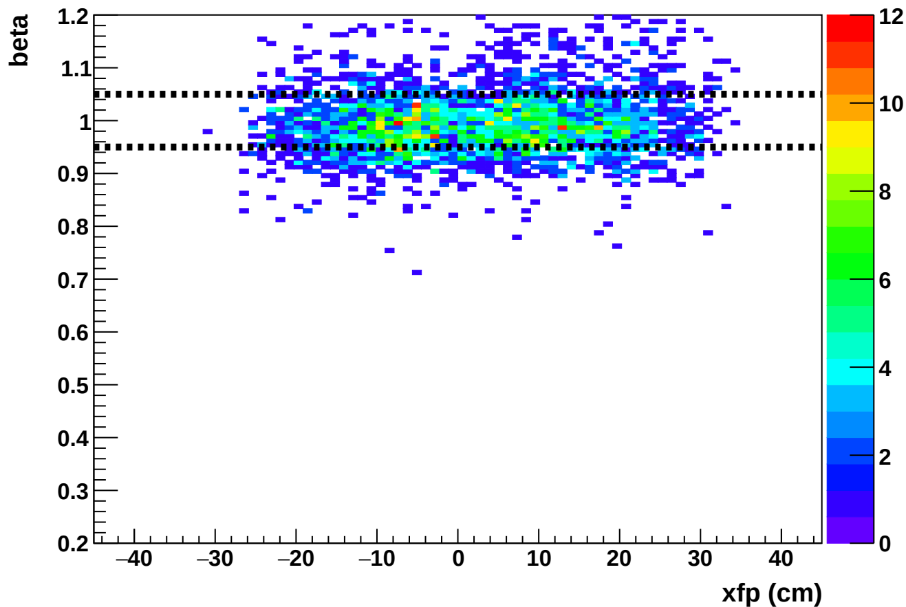
Phase 2 run 27304: beta vs xfp (SHMS)
