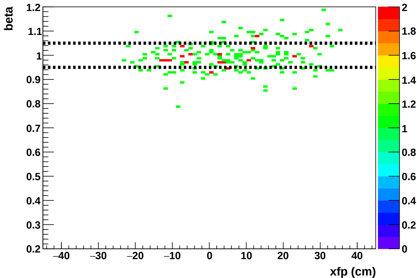
Phase 2 run 27266: beta vs xfp (SHMS)
