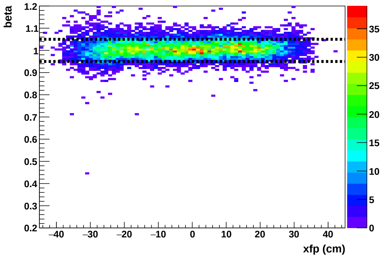
Phase 2 run 27144: beta vs xfp (HMS)
