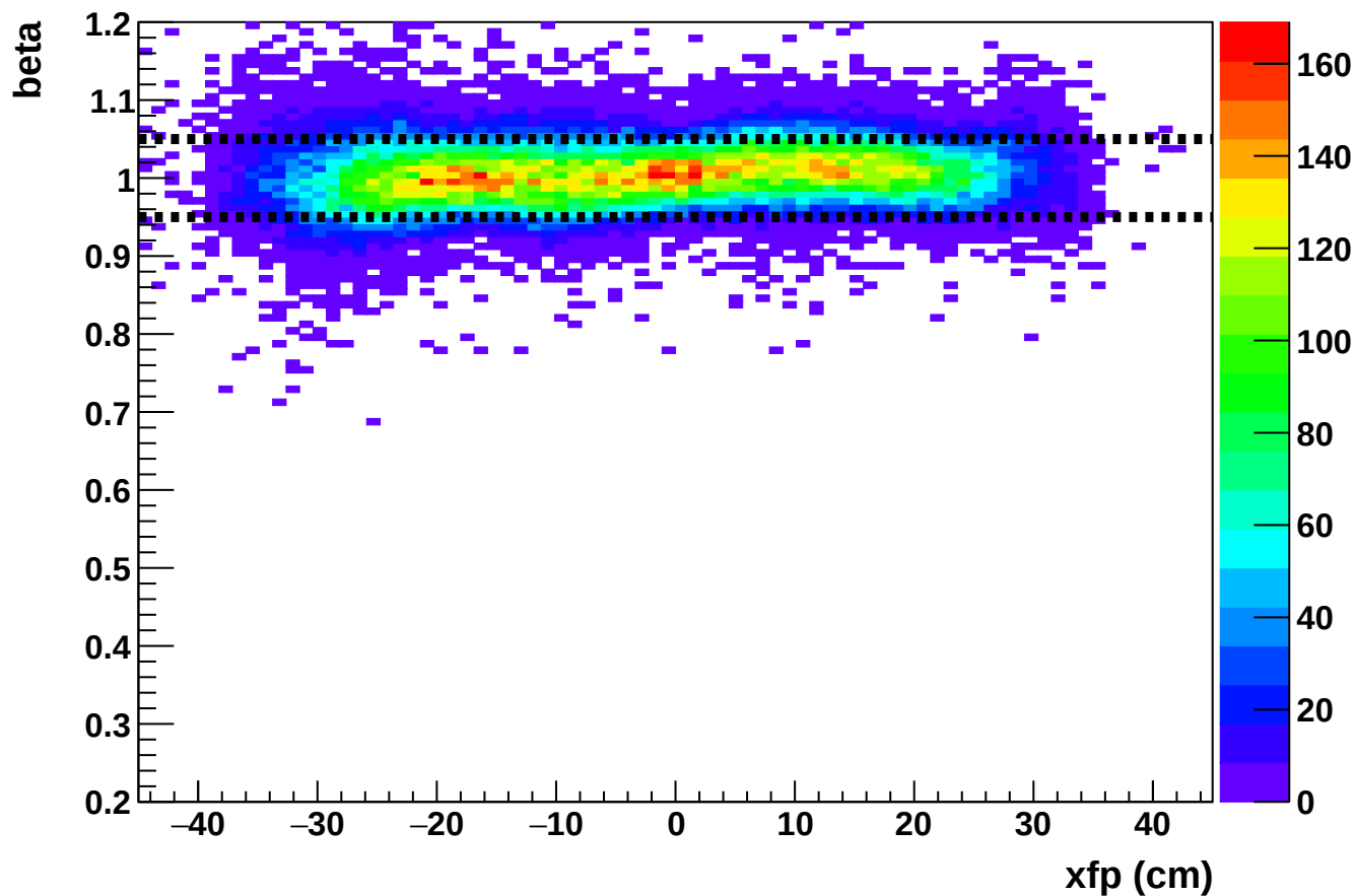
Phase 2 run 27298: beta vs xfp (HMS)
