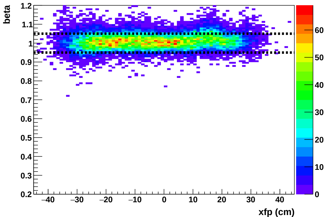
Phase 2 run 27197: beta vs xfp (HMS)
