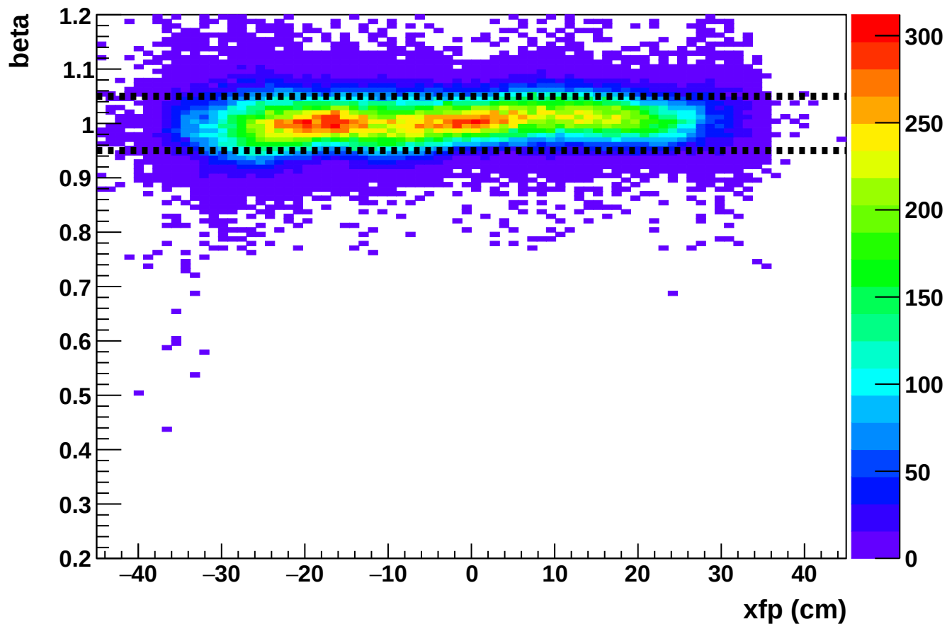
Phase 2 run 27295: beta vs xfp (HMS)
