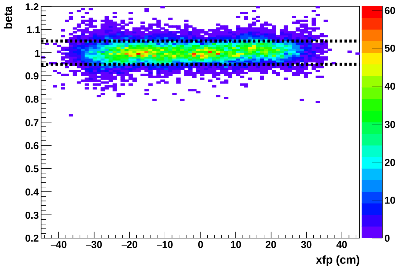
Phase 2 run 27264: beta vs xfp (HMS)
