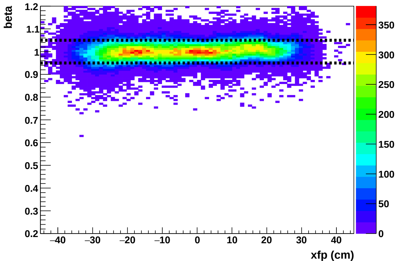
Phase 2 run 27262: beta vs xfp (HMS)
