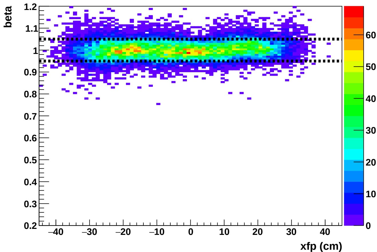
Phase 2 run 27270: beta vs xfp (HMS)
