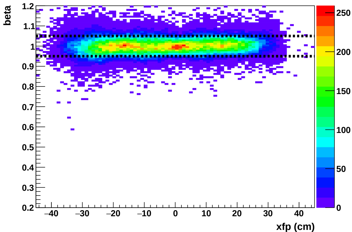
Phase 2 run 27247: beta vs xfp (HMS)
