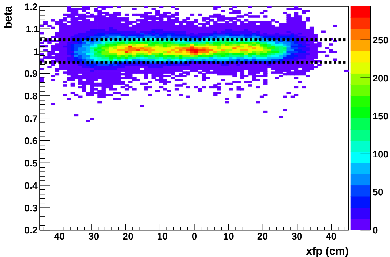
Phase 2 run 27192: beta vs xfp (HMS)
