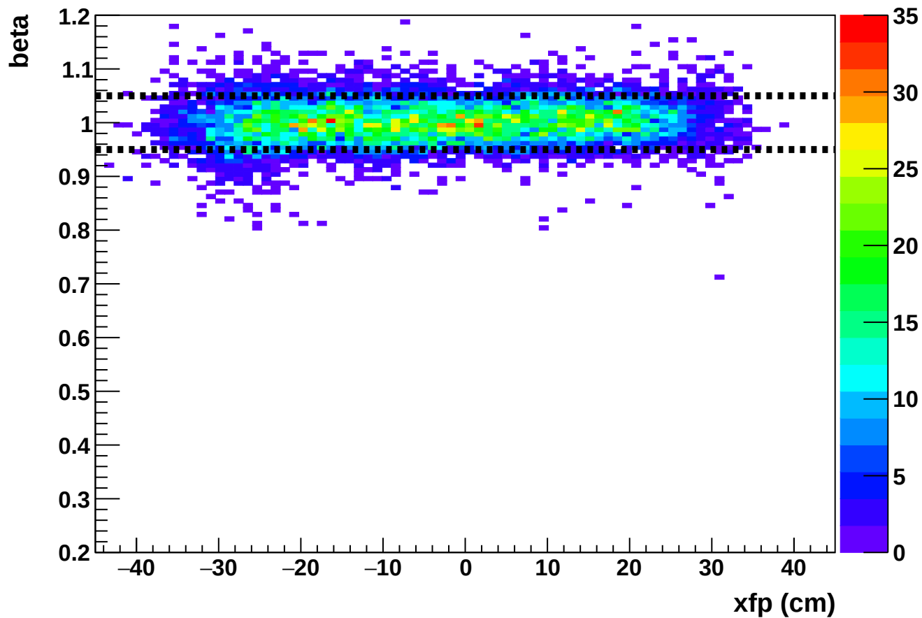
Phase 2 run 27248: beta vs xfp (HMS)
