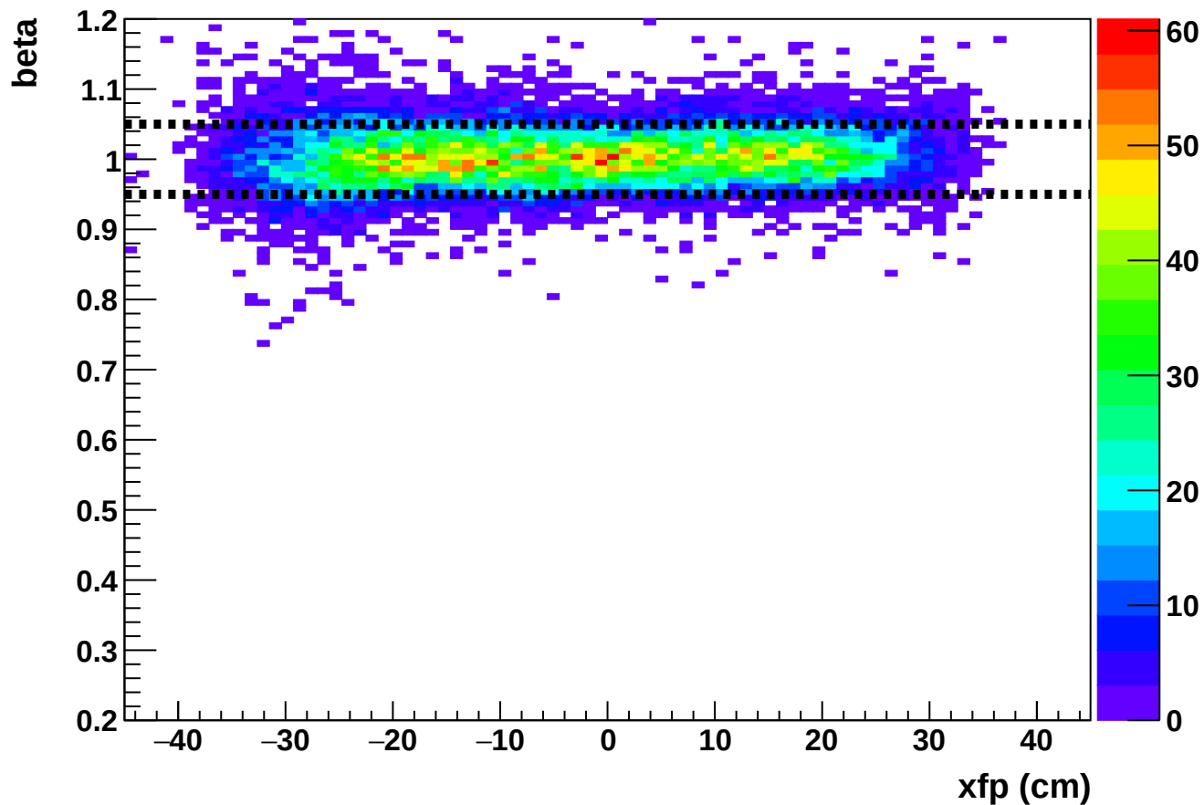
Phase 2 run 27215: beta vs xfp (HMS)
