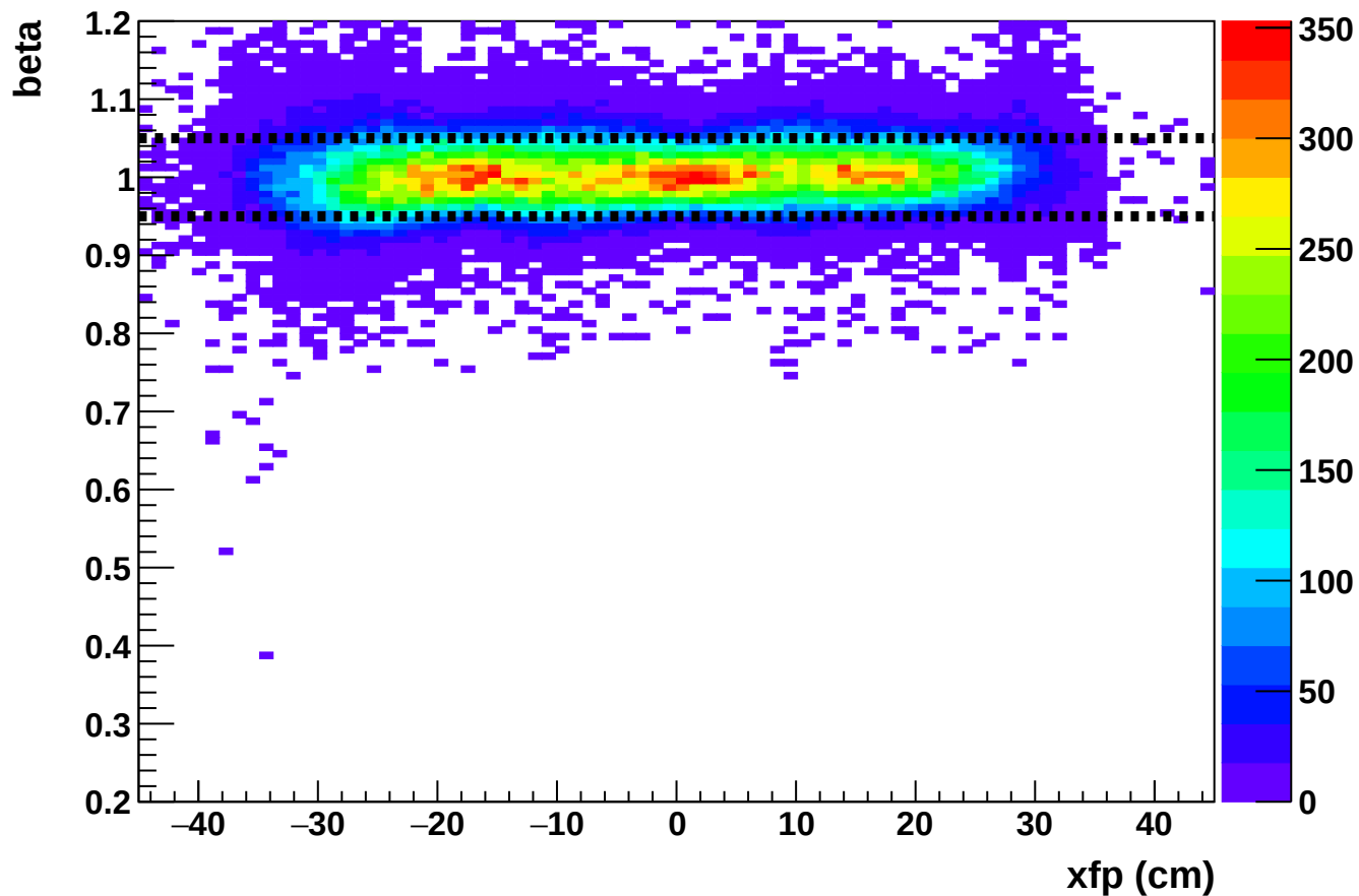
Phase 2 run 27214: beta vs xfp (HMS)
