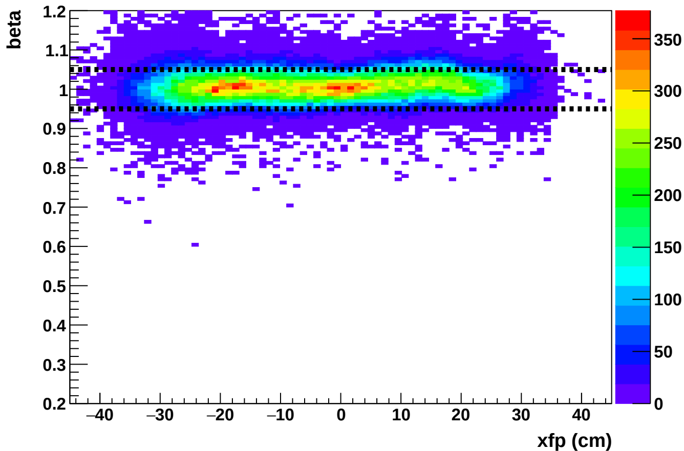
Phase 2 run 27372: beta vs xfp (HMS)
