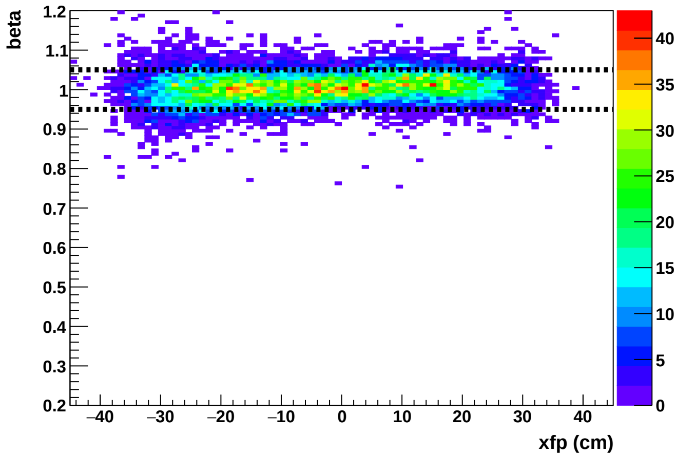
Phase 2 run 27299: beta vs xfp (HMS)
