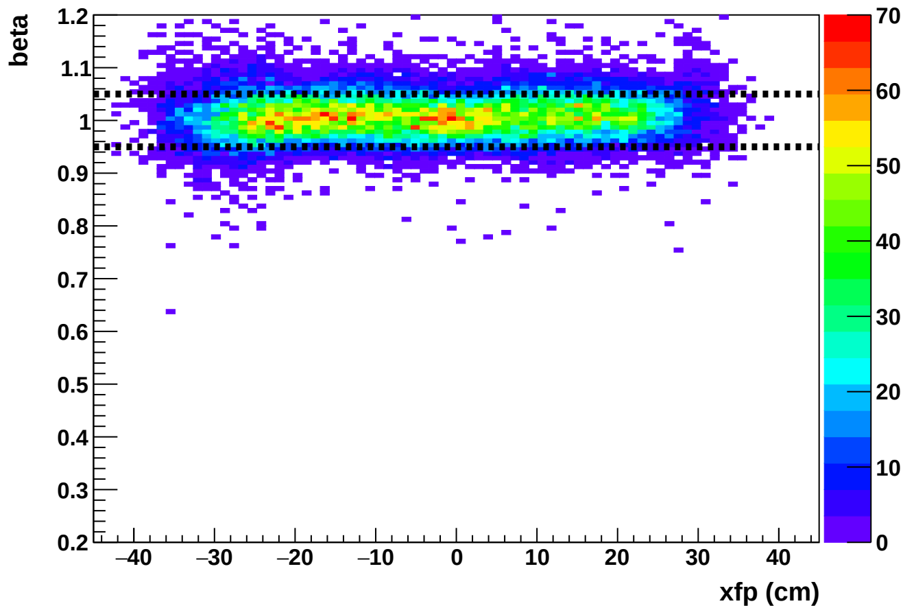
Phase 2 run 27379: beta vs xfp (HMS)
