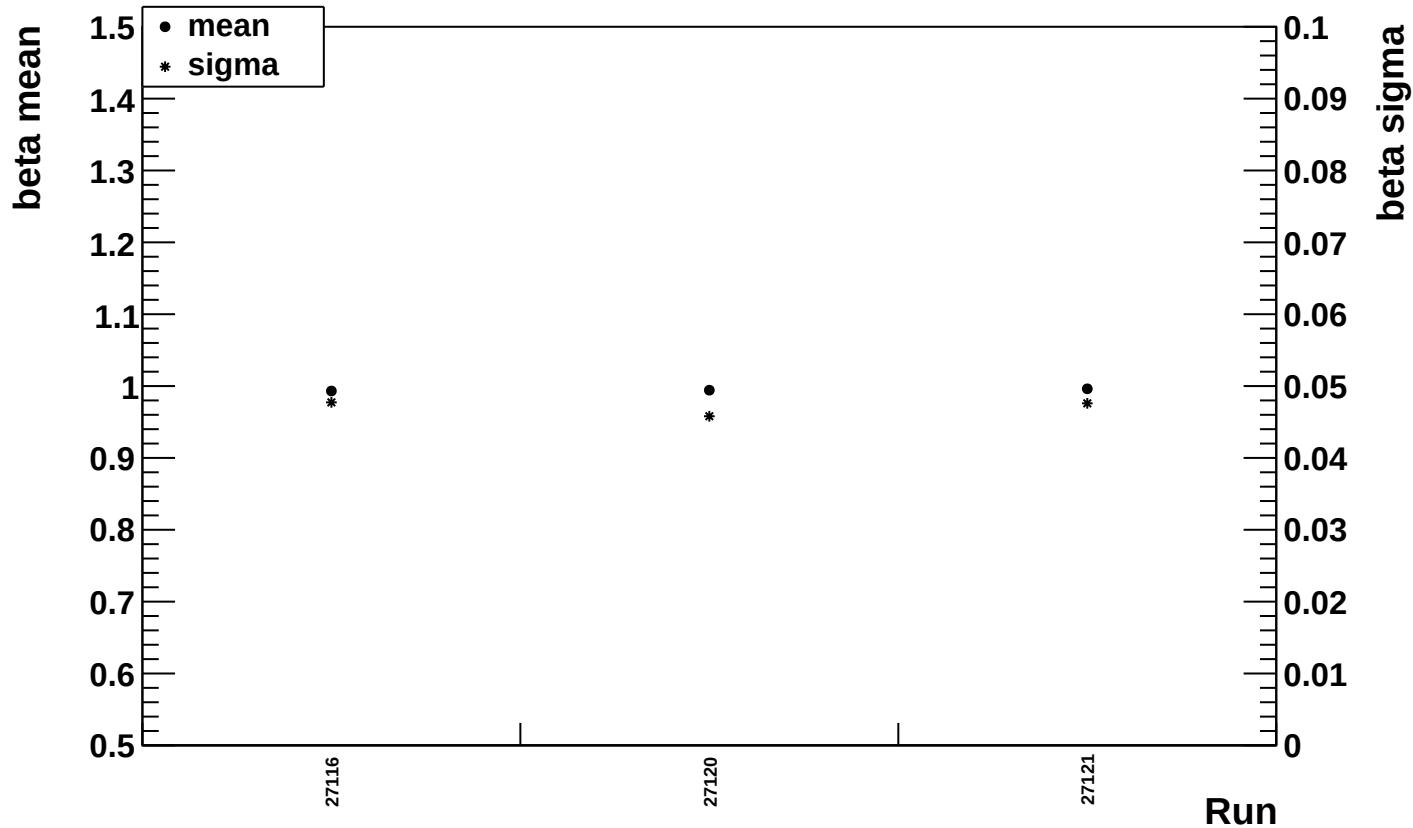
Phase 2 shms_electron: beta mean / sigma vs run
