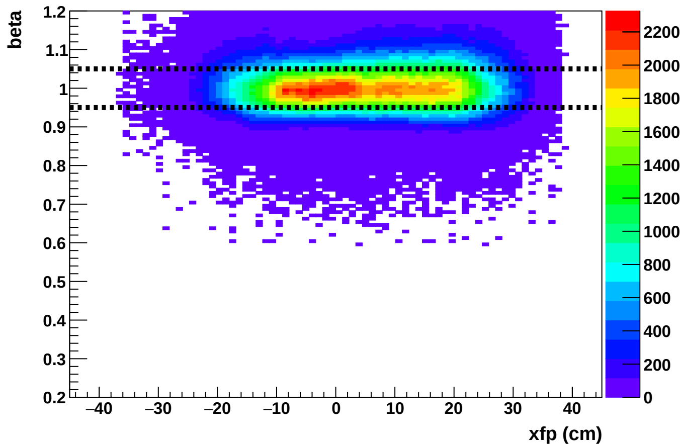
Phase 2 run 27121: beta vs xfp (SHMS)
