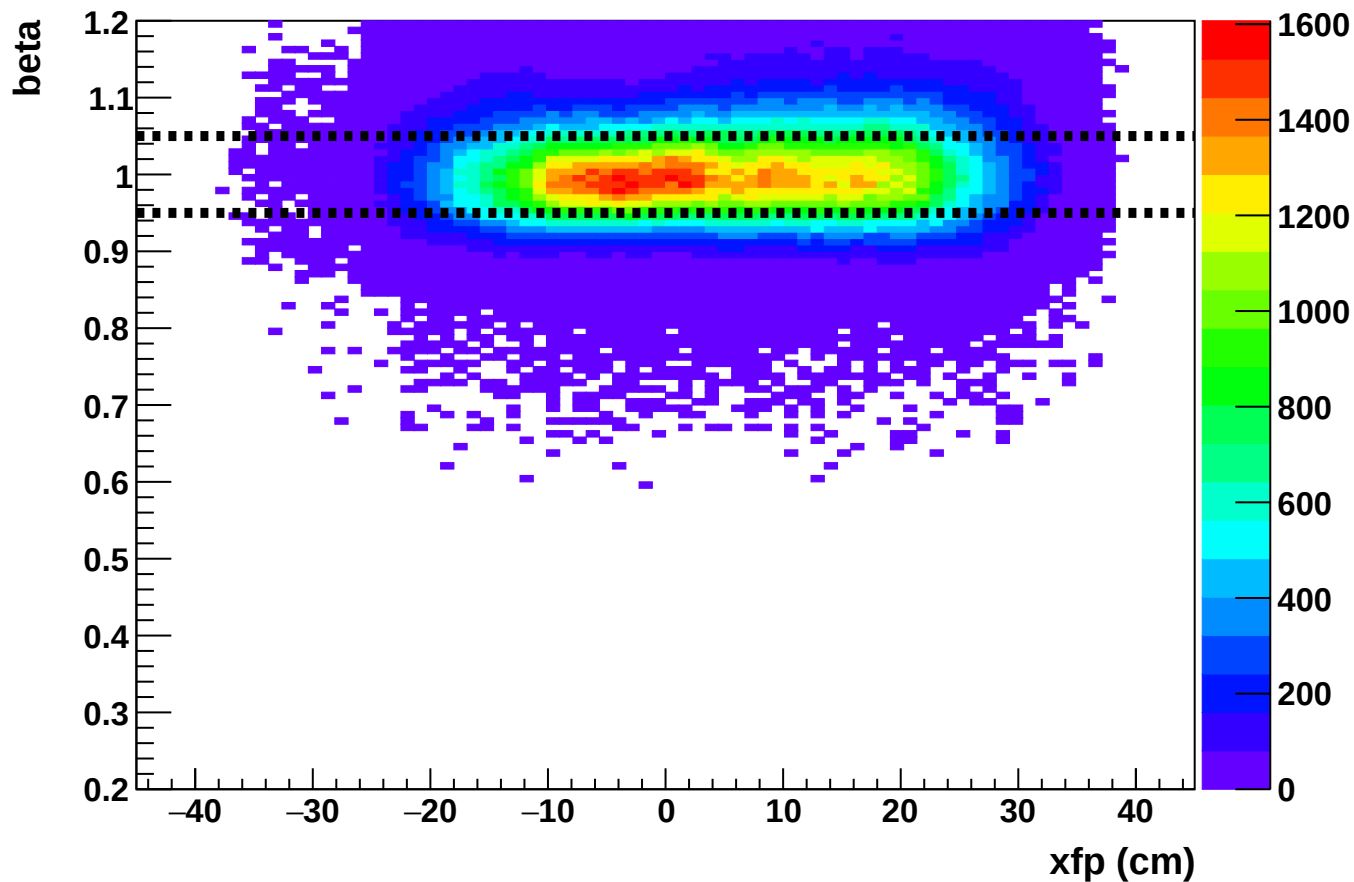
Phase 2 run 27120: beta vs xfp (SHMS)
