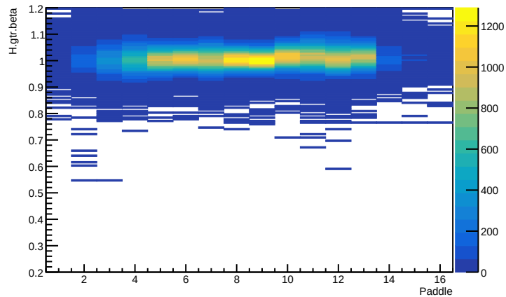
HMS beta vs 2x accepted paddle
