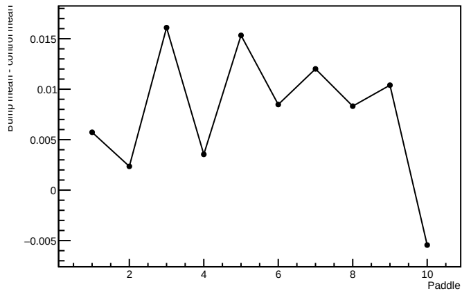
HMS 2y beta displacement
