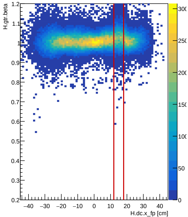
Phase 2 run 28425: HMS beta vs HMS xfp
