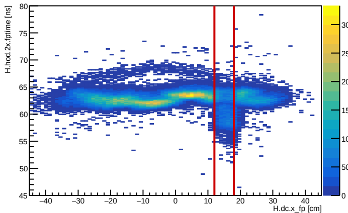
HMS 2x fptime vs xfp
