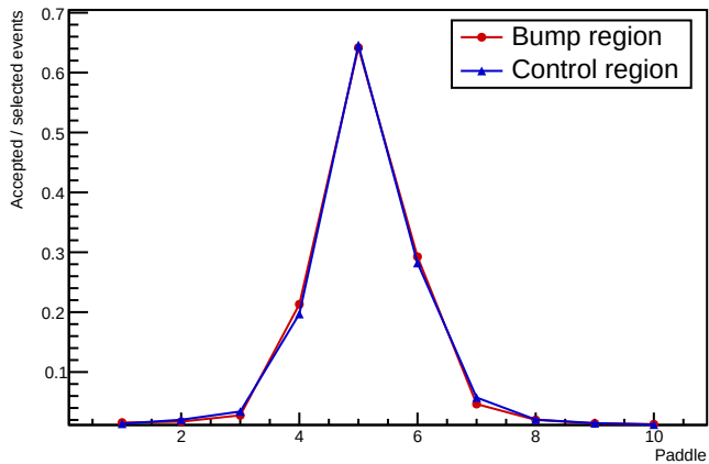
HMS 2y candidate ranking
