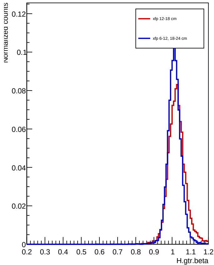
Bump and control beta spectra
