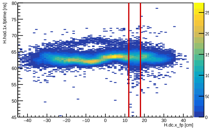
HMS 1x fptime vs xfp
