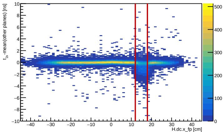
HMS 2x time residual vs xfp
