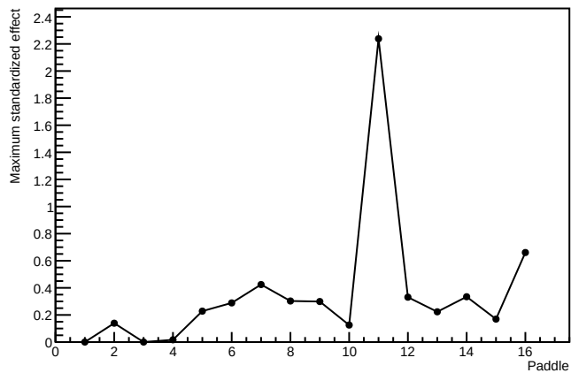
HMS 1x candidate ranking
