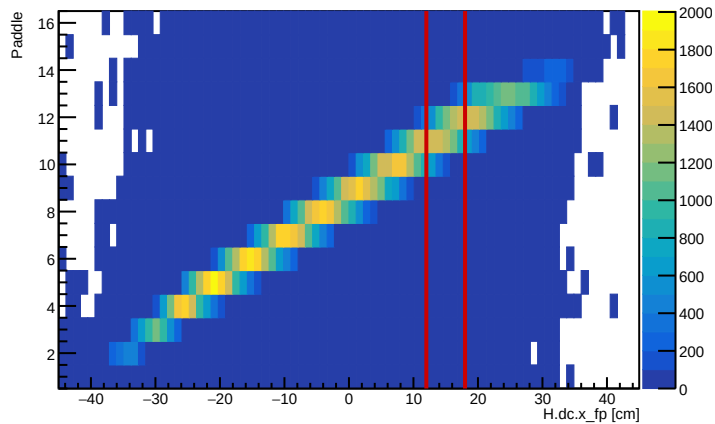
HMS 2x accepted paddle vs xfp
