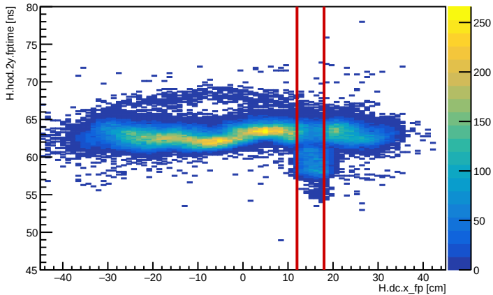
HMS 2y fptime vs xfp
