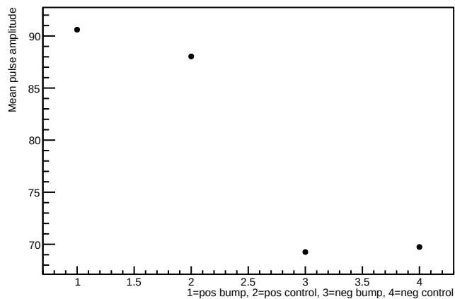
ADC amplitude means
