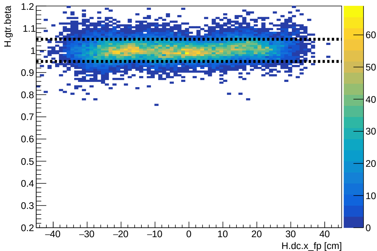
Phase 2 run 27270: HMS beta vs HMS xfp
