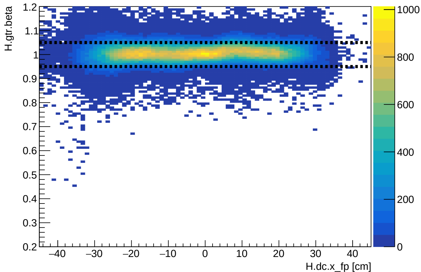
Phase 2 run 28239: HMS beta vs HMS xfp
