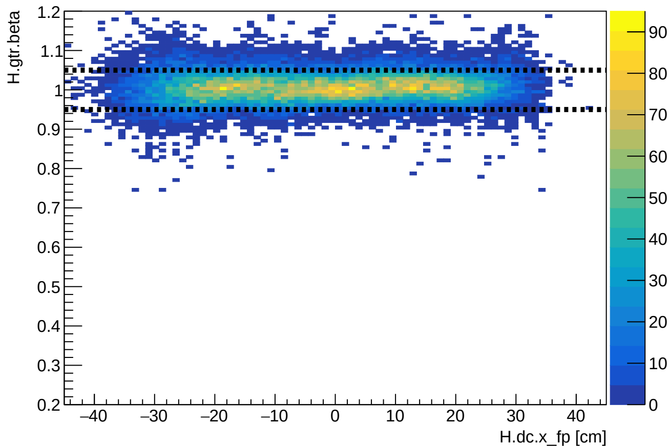
Phase 2 run 27175: HMS beta vs HMS xfp
