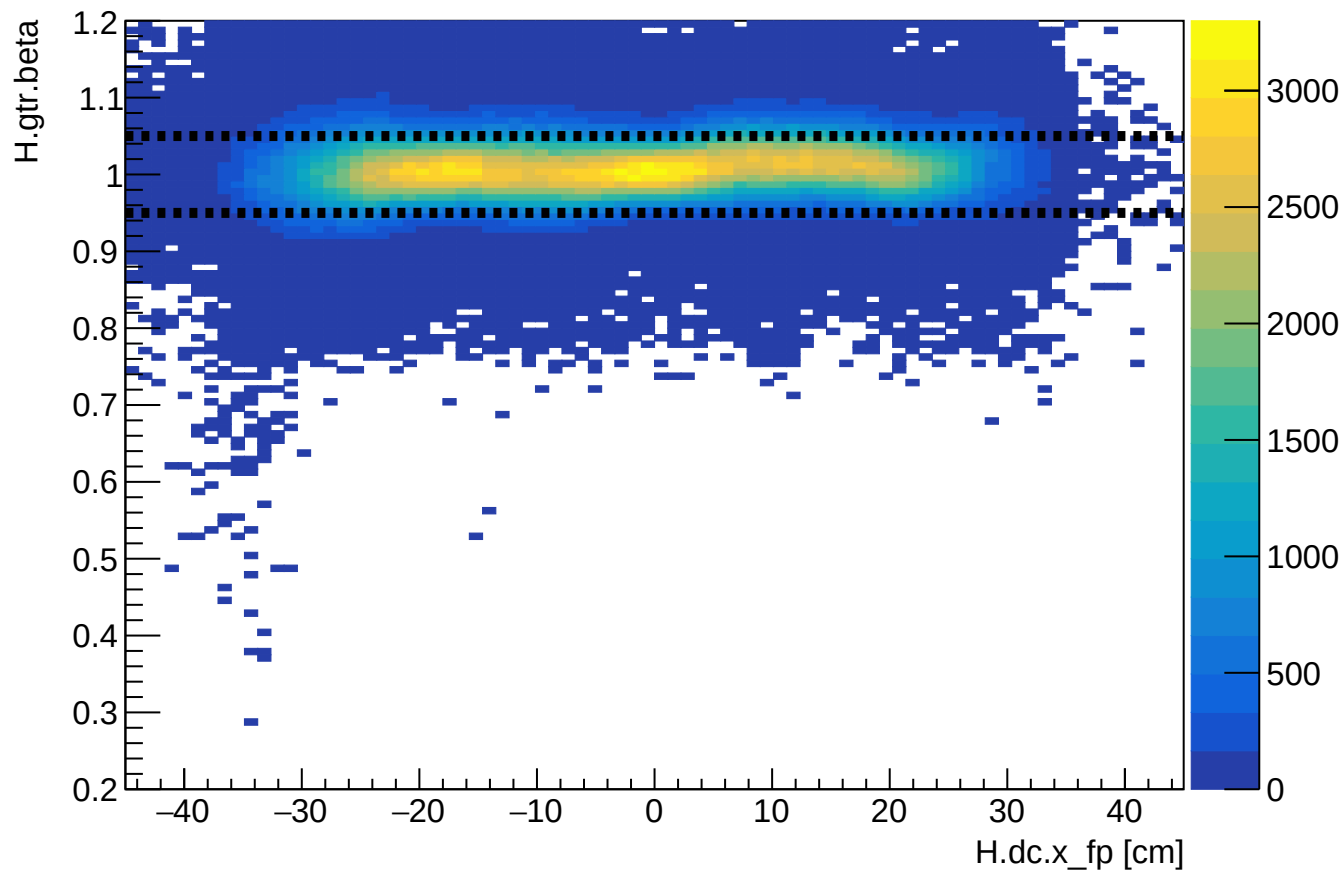
Phase 2 run 28255: HMS beta vs HMS xfp
