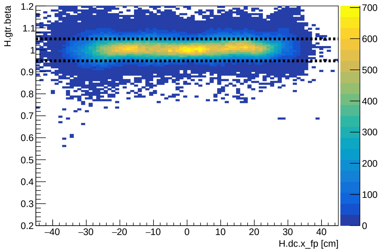
Phase 2 run 27179: HMS beta vs HMS xfp
