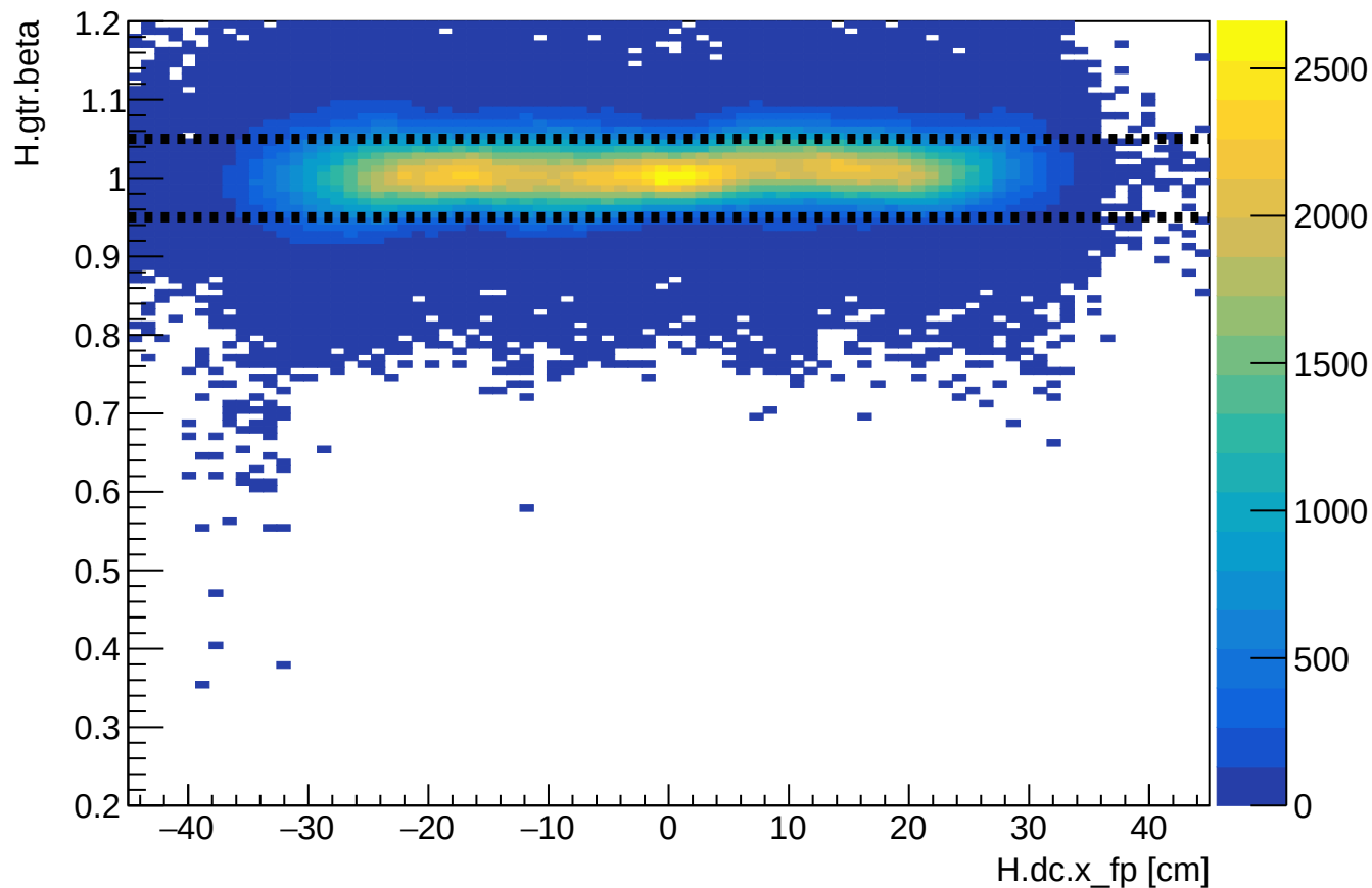
Phase 2 run 28266: HMS beta vs HMS xfp
