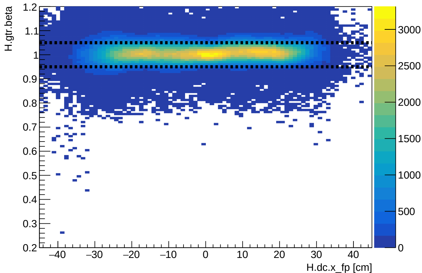
Phase 2 run 27798: HMS beta vs HMS xfp
