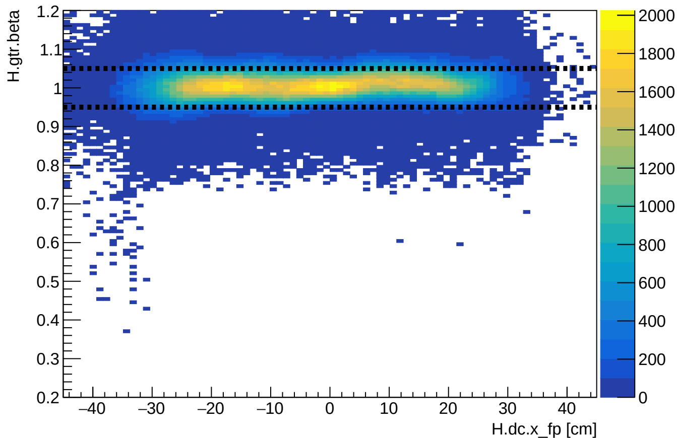
Phase 2 run 28236: HMS beta vs HMS xfp
