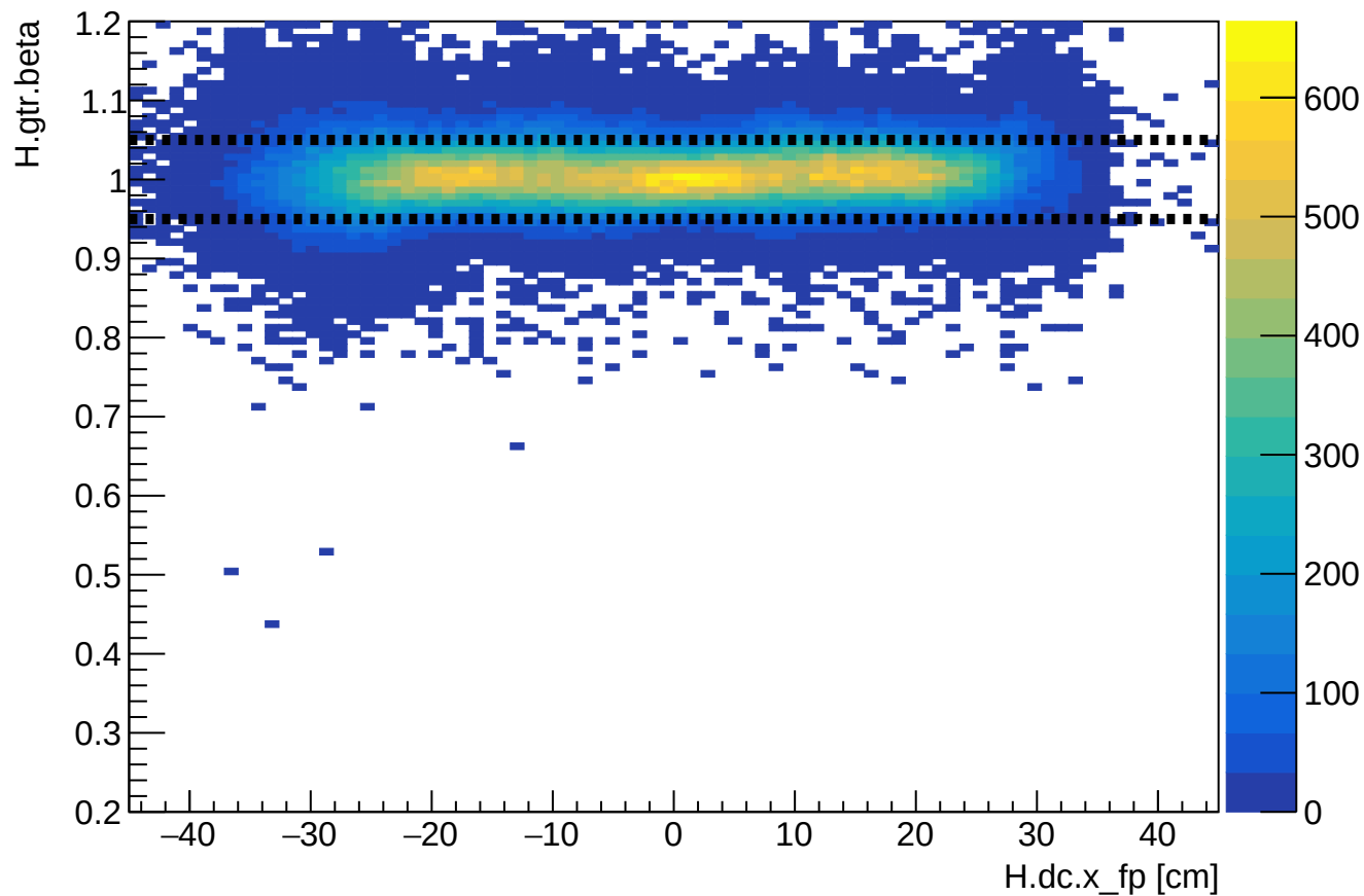
Phase 2 run 27138: HMS beta vs HMS xfp
