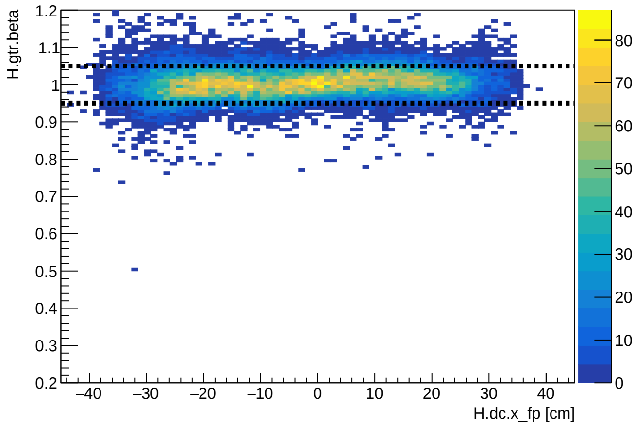
Phase 2 run 27282: HMS beta vs HMS xfp
