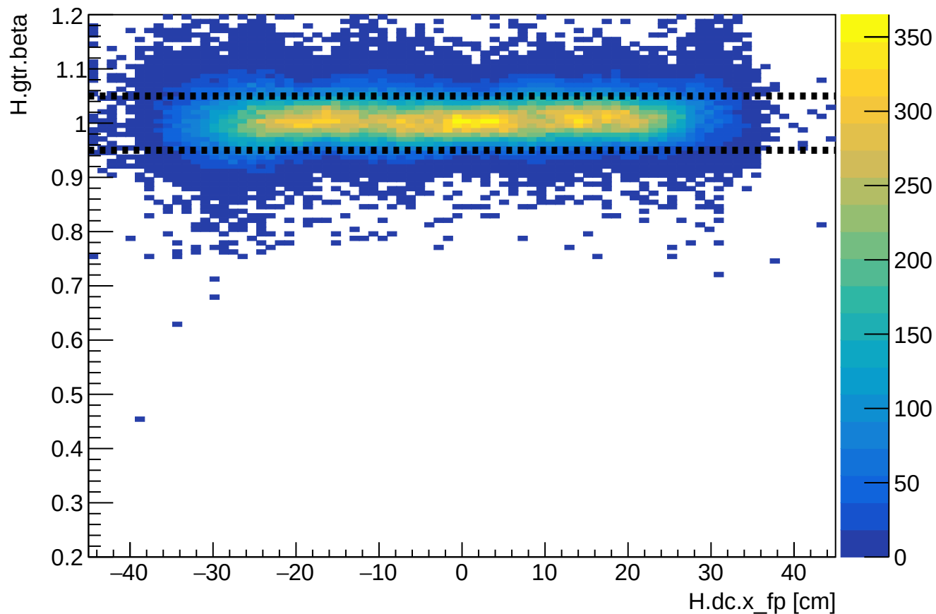
Phase 2 run 27161: HMS beta vs HMS xfp
