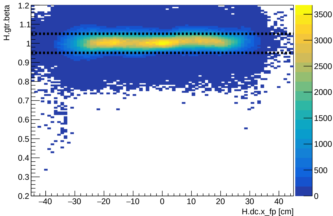
Phase 2 run 28247: HMS beta vs HMS xfp
