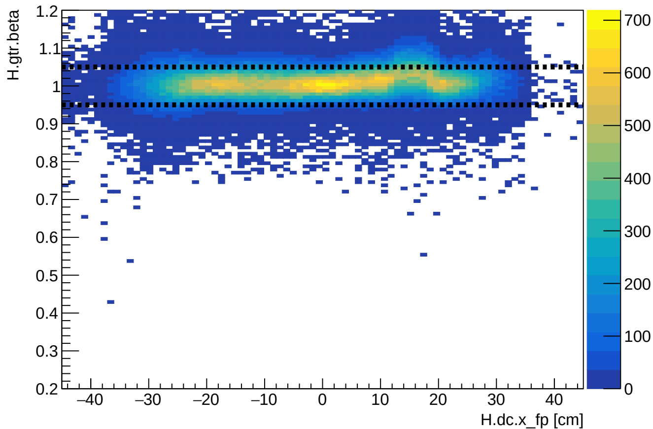
Phase 2 run 28428: HMS beta vs HMS xfp
