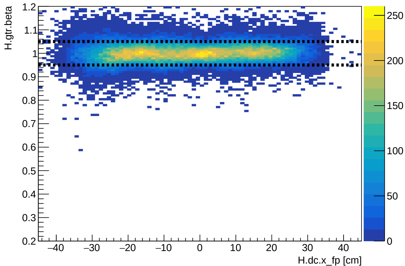
Phase 2 run 27247: HMS beta vs HMS xfp
