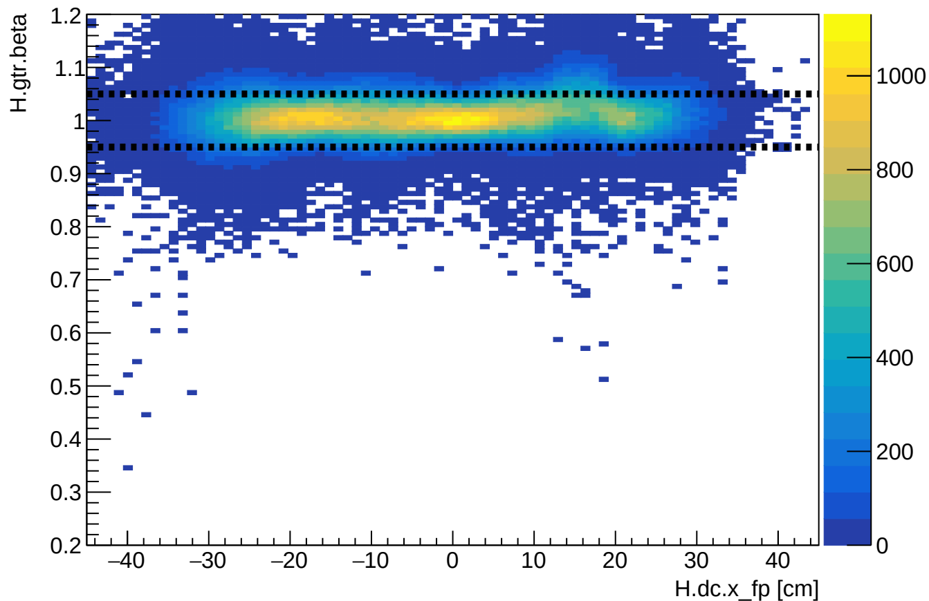
Phase 2 run 28284: HMS beta vs HMS xfp
