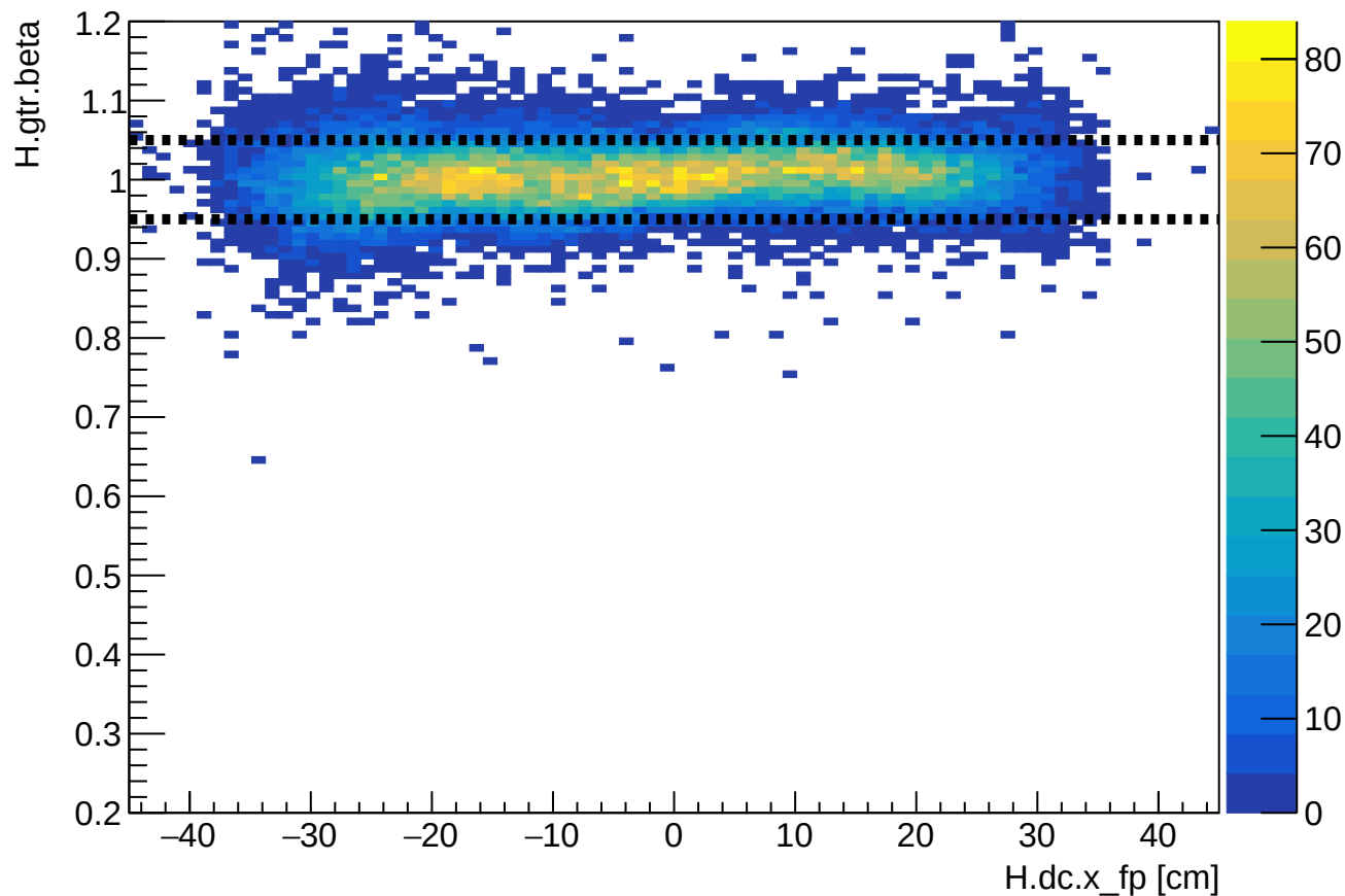
Phase 2 run 27299: HMS beta vs HMS xfp
