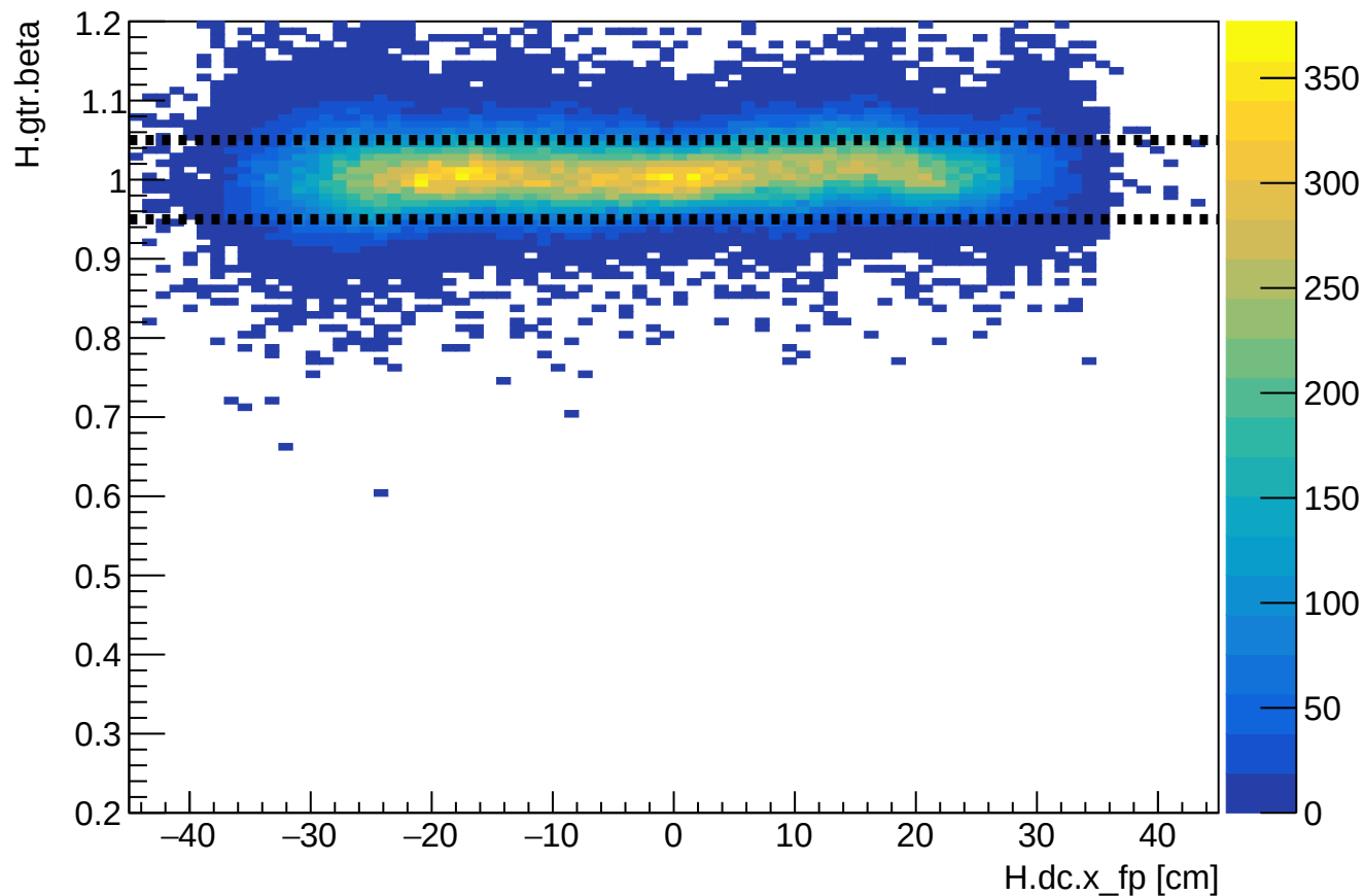
Phase 2 run 27372: HMS beta vs HMS xfp
