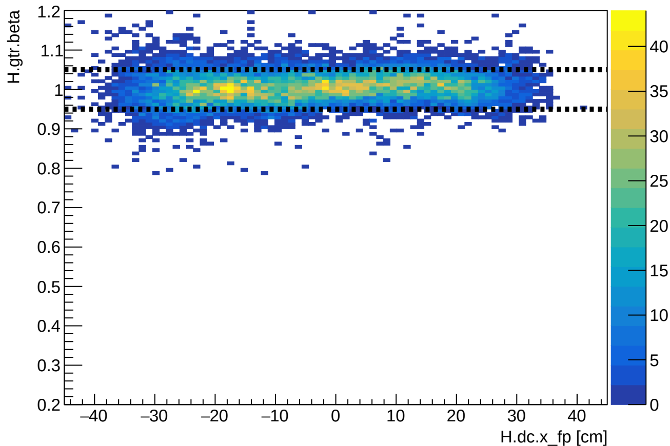
Phase 2 run 27284: HMS beta vs HMS xfp
