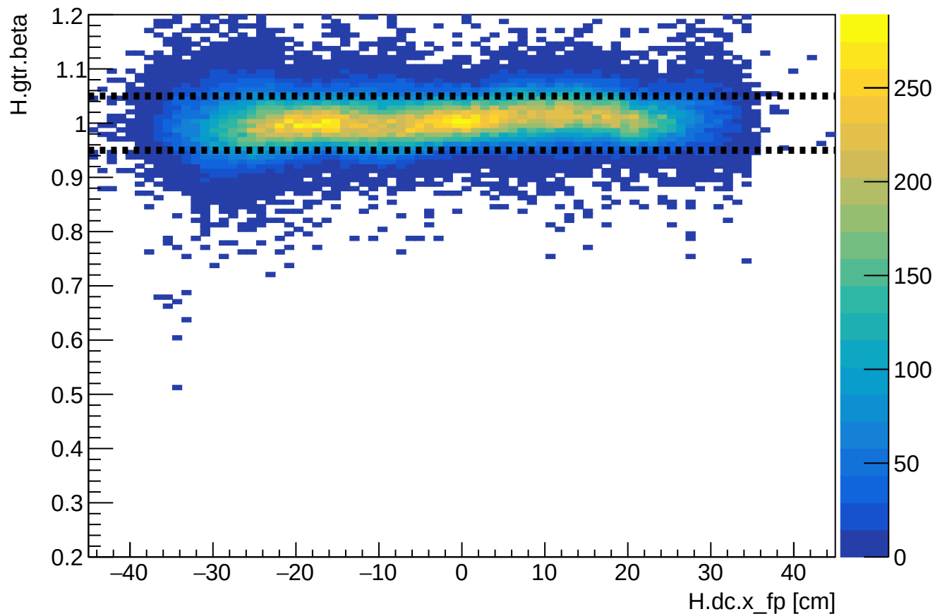
Phase 2 run 27283: HMS beta vs HMS xfp
