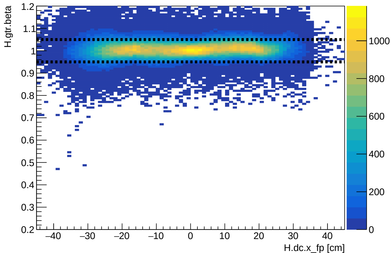
Phase 2 run 27159: HMS beta vs HMS xfp
