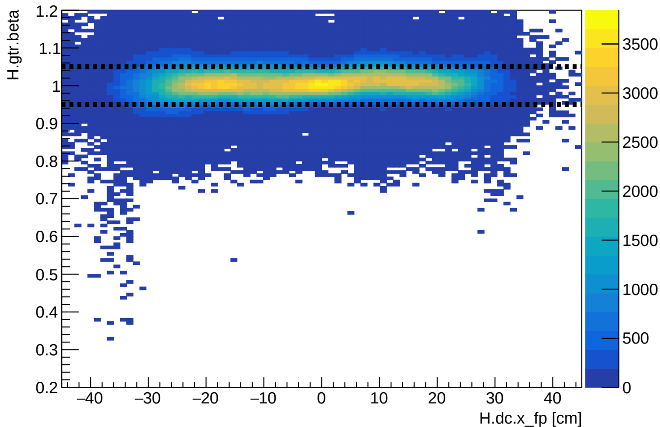
Phase 2 run 28244: HMS beta vs HMS xfp
