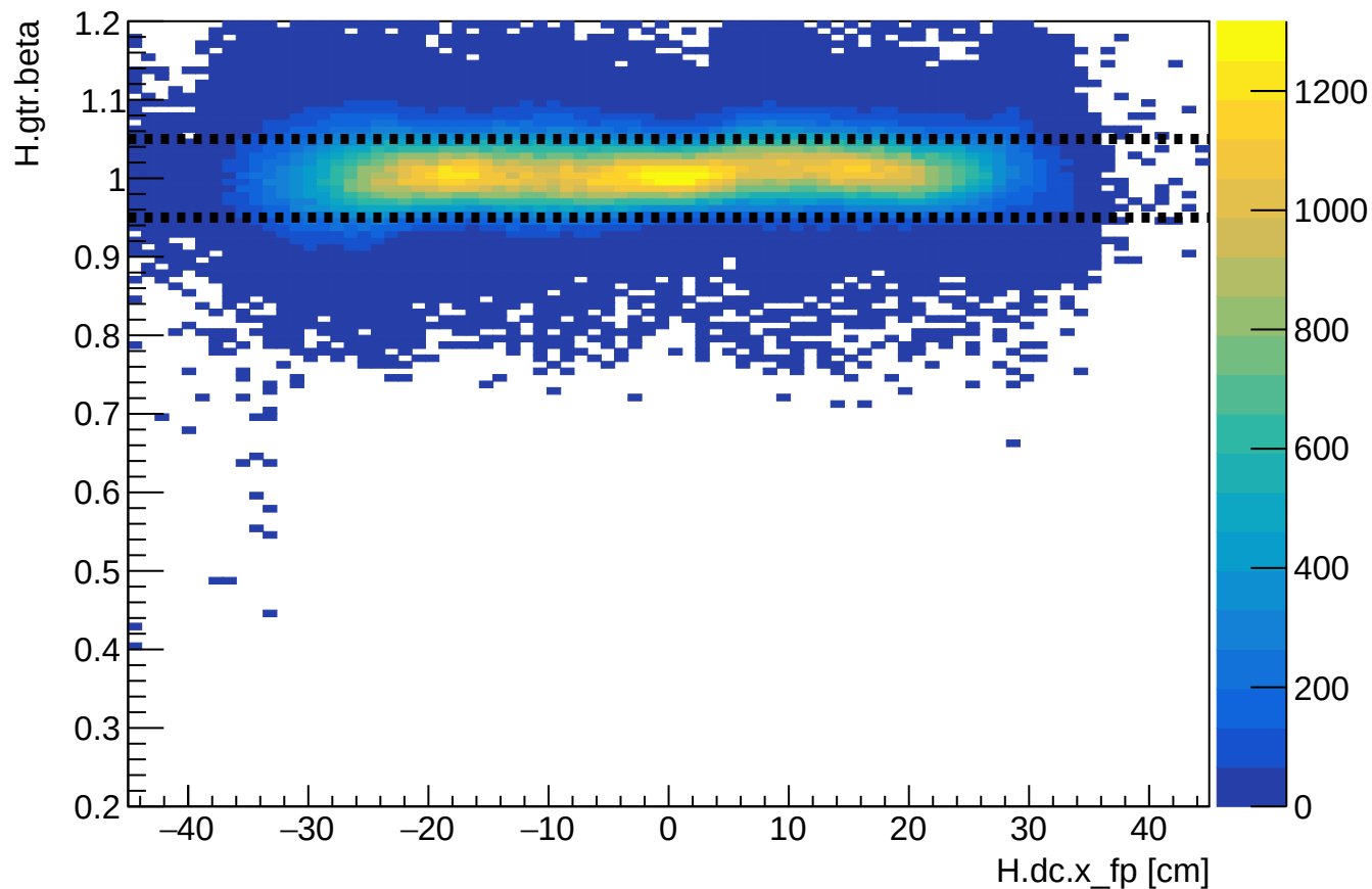
Phase 2 run 28225: HMS beta vs HMS xfp
