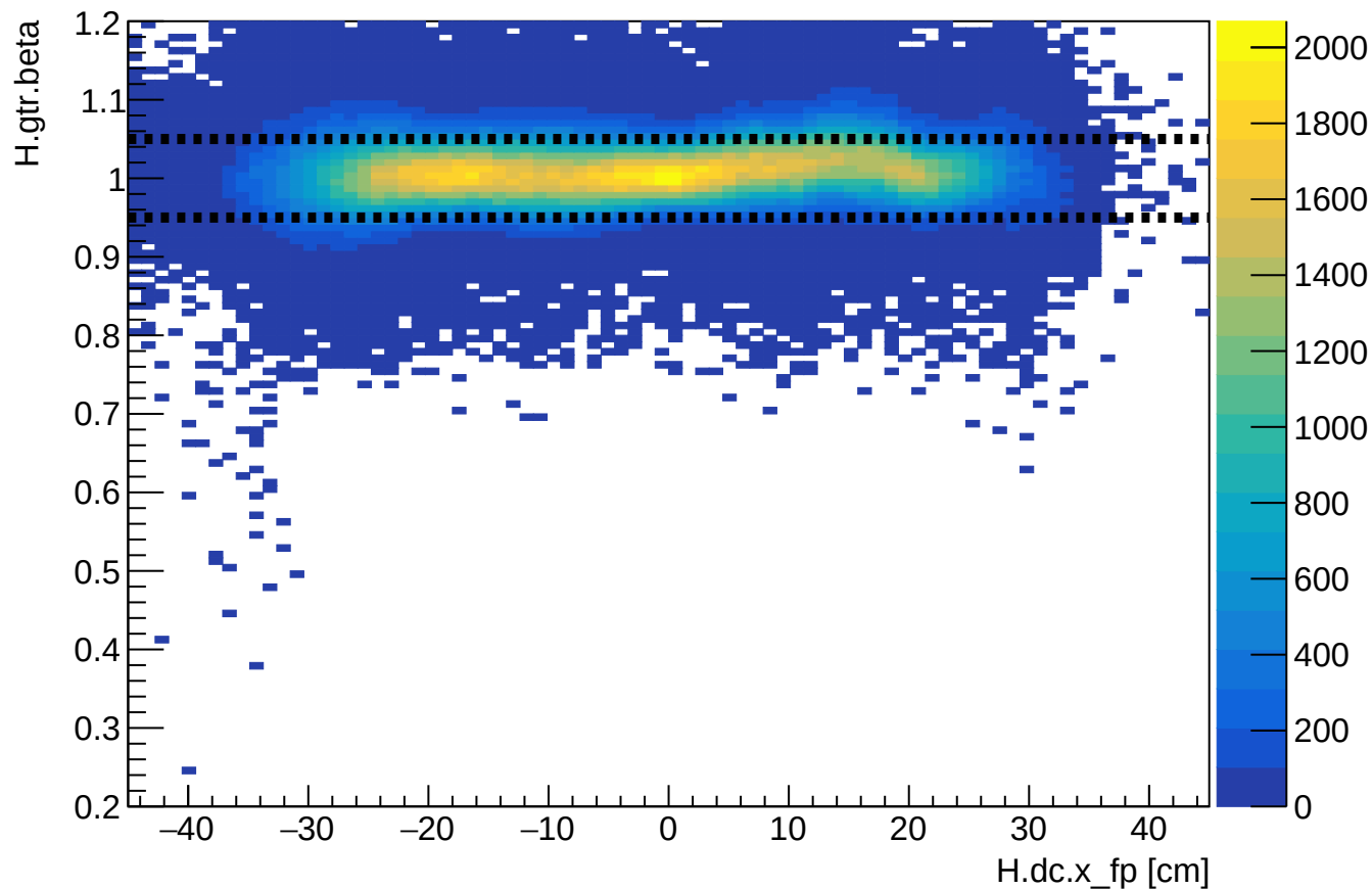
Phase 2 run 28232: HMS beta vs HMS xfp
