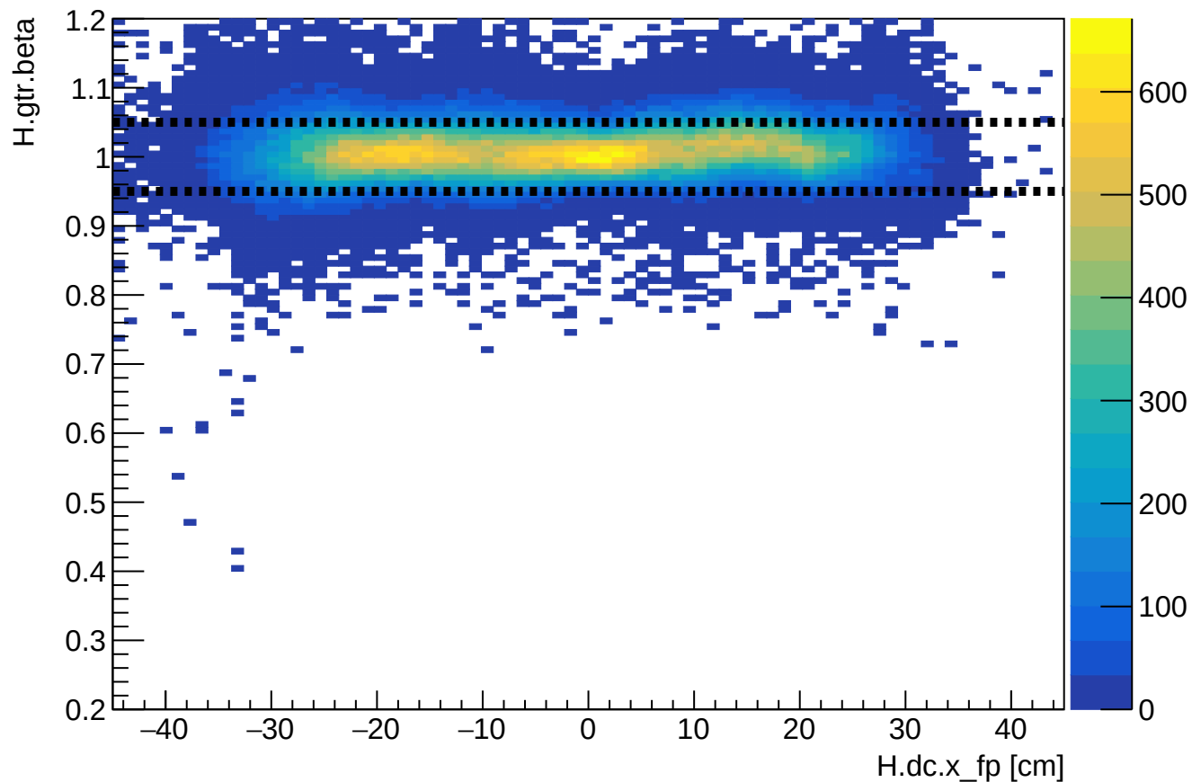
Phase 2 run 28229: HMS beta vs HMS xfp
