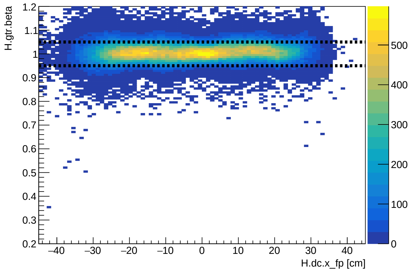
Phase 2 run 28349: HMS beta vs HMS xfp
