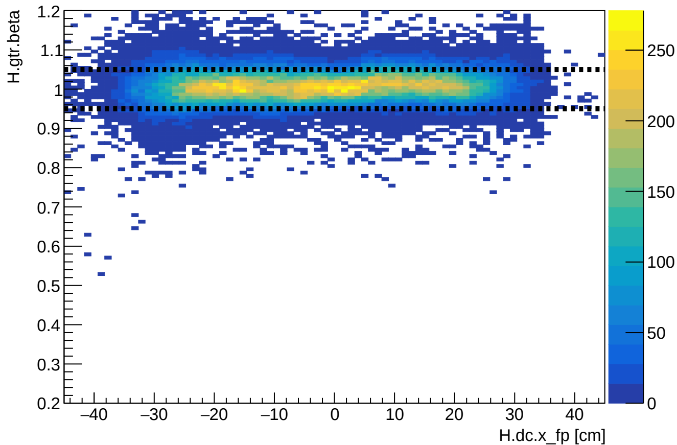
Phase 2 run 28201: HMS beta vs HMS xfp
