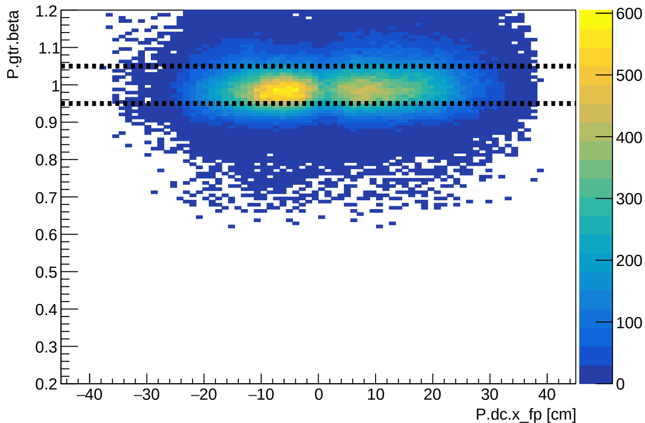
Phase 2 run 28328: SHMS beta vs SHMS xfp
