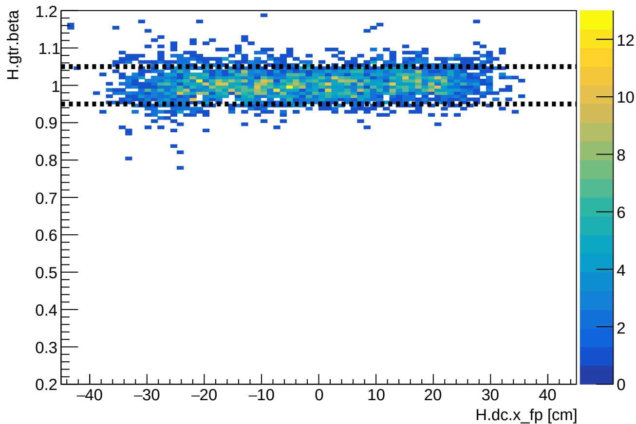
Phase 2 run 27230: HMS beta vs HMS xfp
