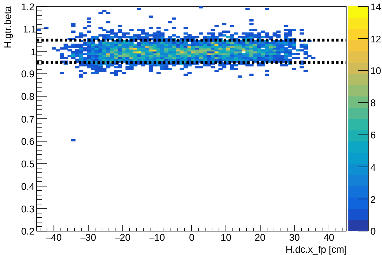
Phase 2 run 27307: HMS beta vs HMS xfp
