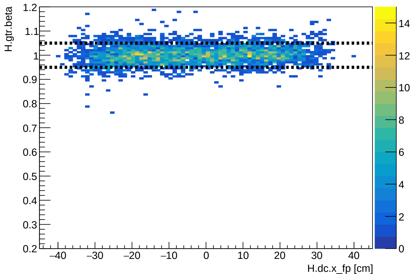
Phase 2 run 27242: HMS beta vs HMS xfp
