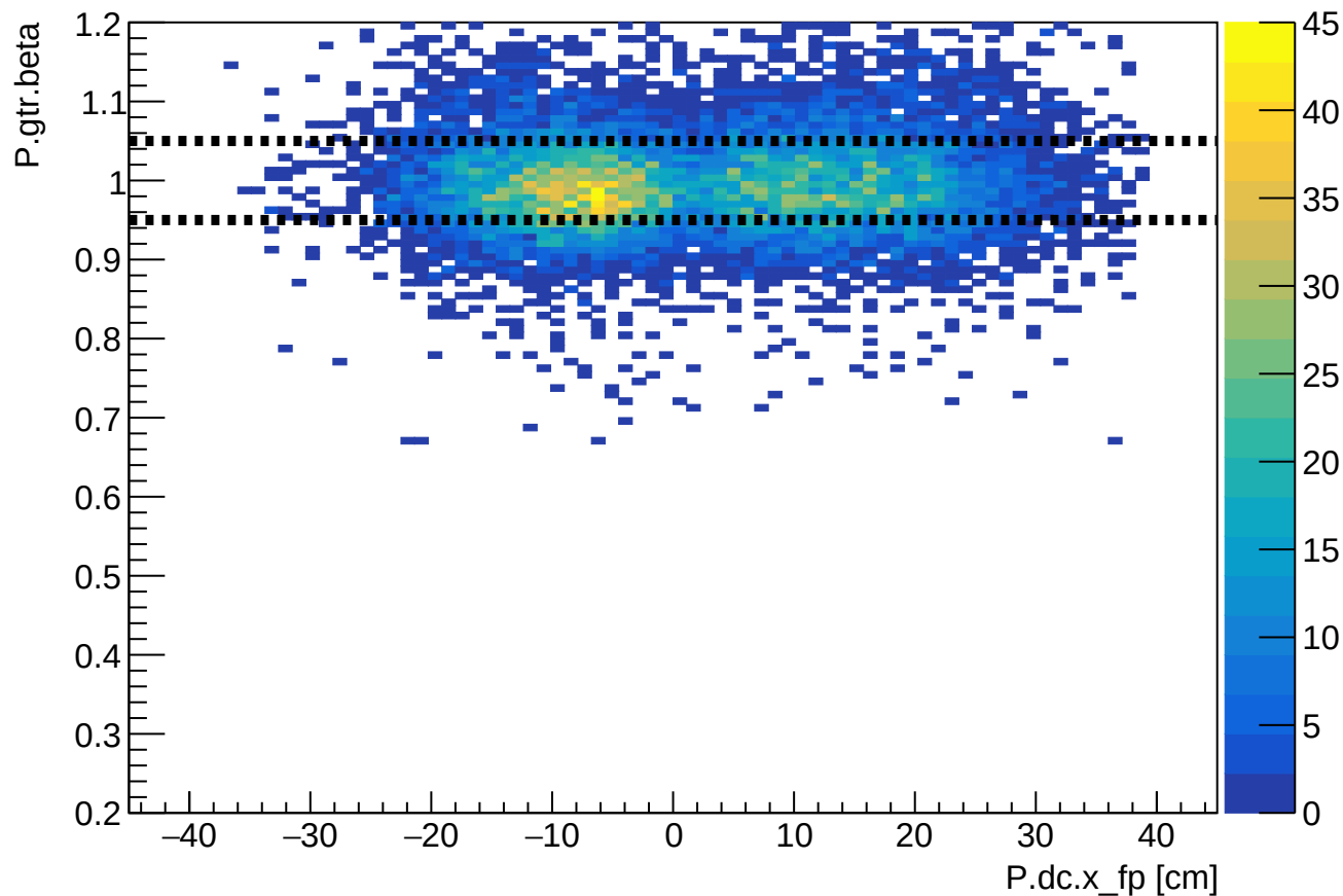
Phase 2 run 27131: SHMS beta vs SHMS xfp
