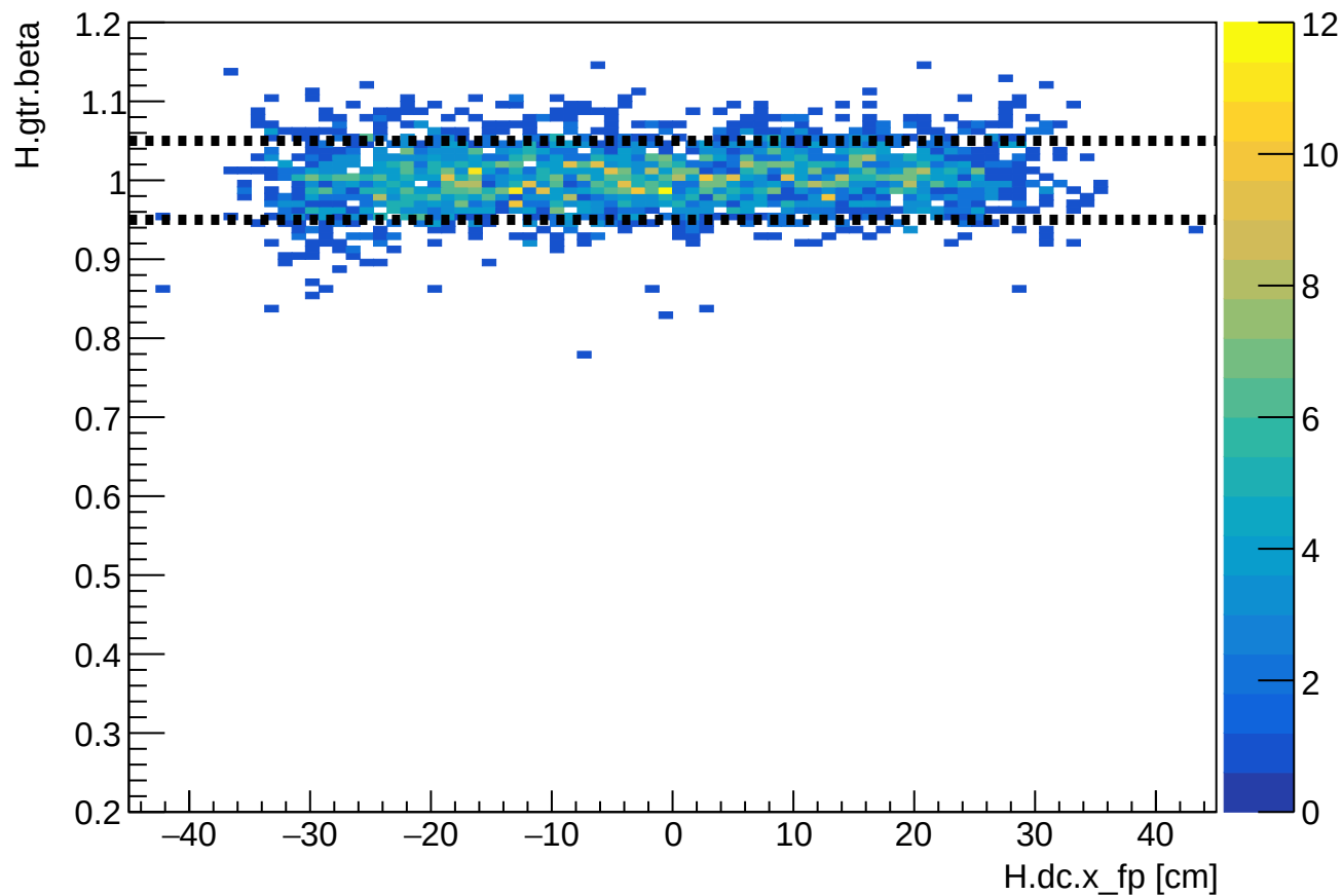
Phase 2 run 27228: HMS beta vs HMS xfp
