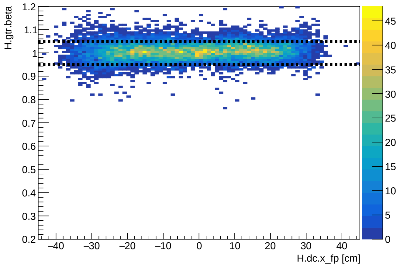
Phase 2 run 27142: HMS beta vs HMS xfp
