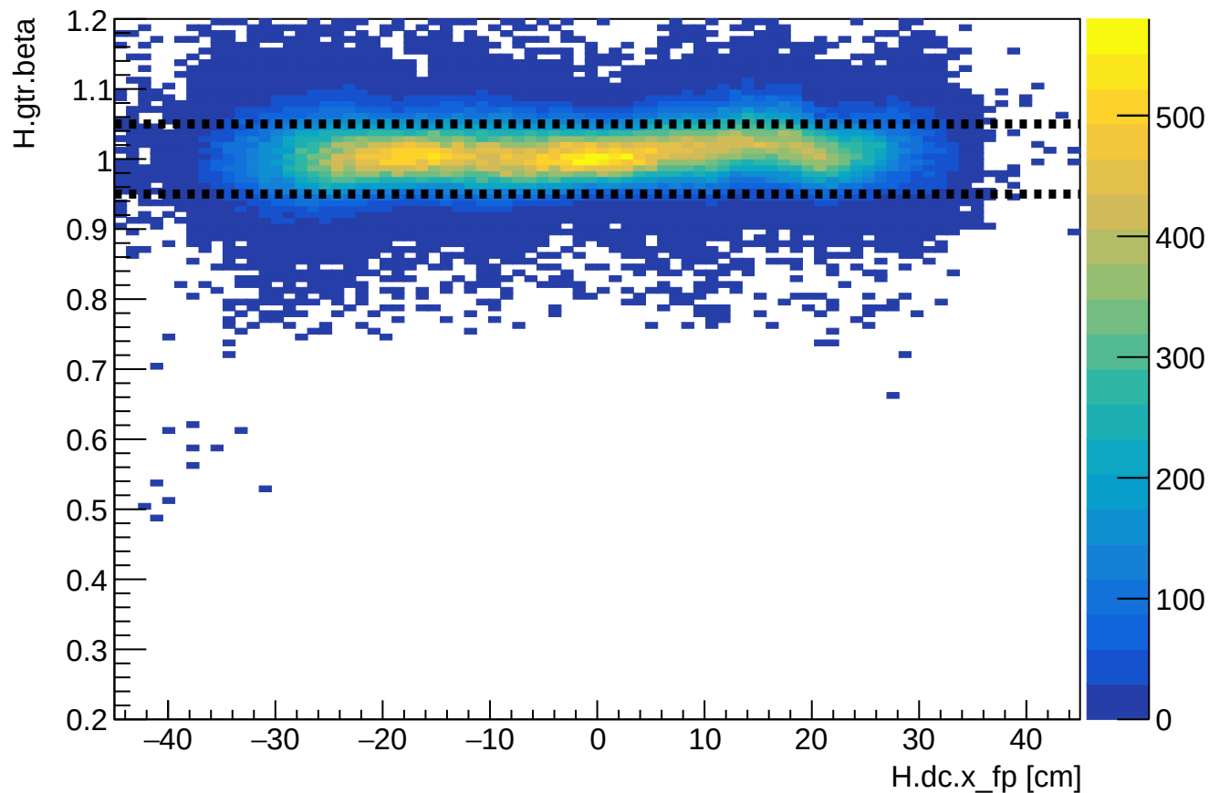
Phase 2 run 28331: HMS beta vs HMS xfp
