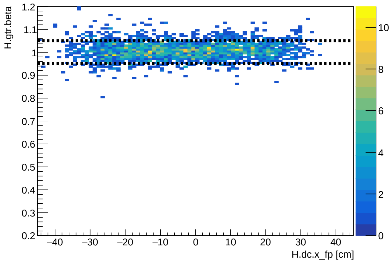
Phase 2 run 27418: HMS beta vs HMS xfp
