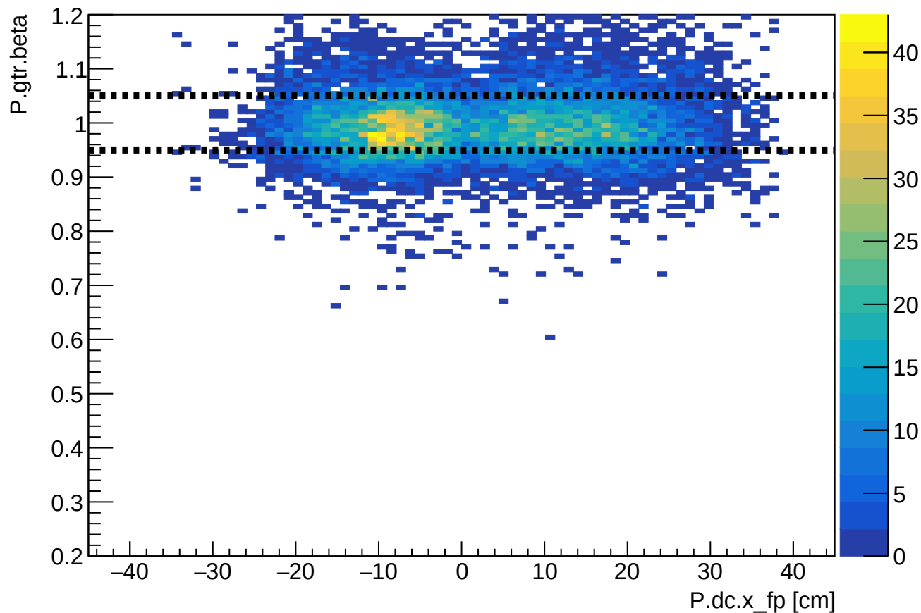
Phase 2 run 27130: SHMS beta vs SHMS xfp
