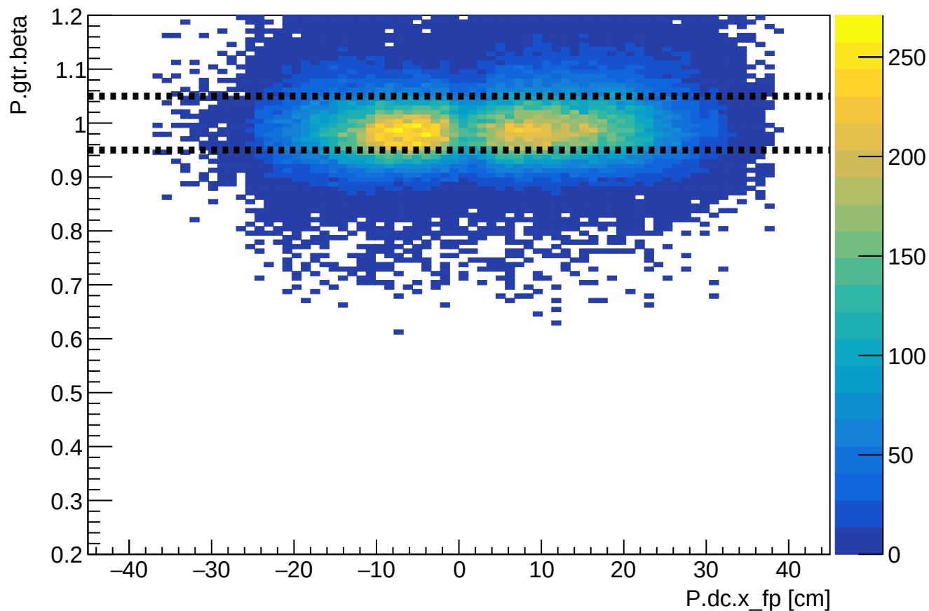
Phase 2 run 28189: SHMS beta vs SHMS xfp
