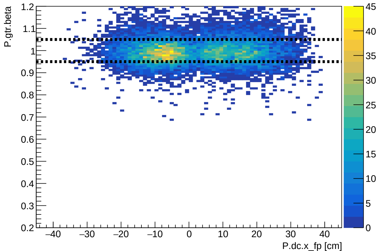
Phase 2 run 27124: SHMS beta vs SHMS xfp
