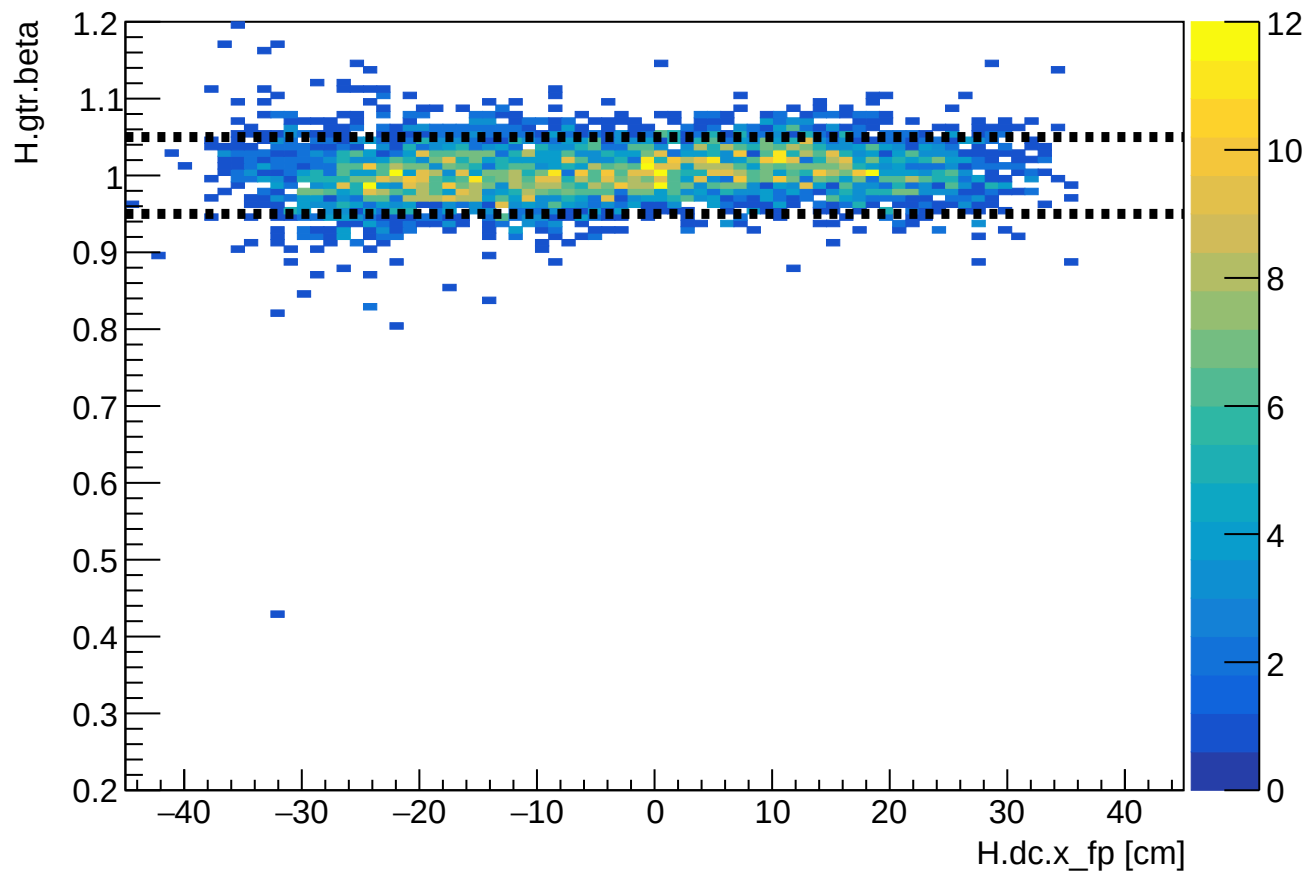
Phase 2 run 27279: HMS beta vs HMS xfp
