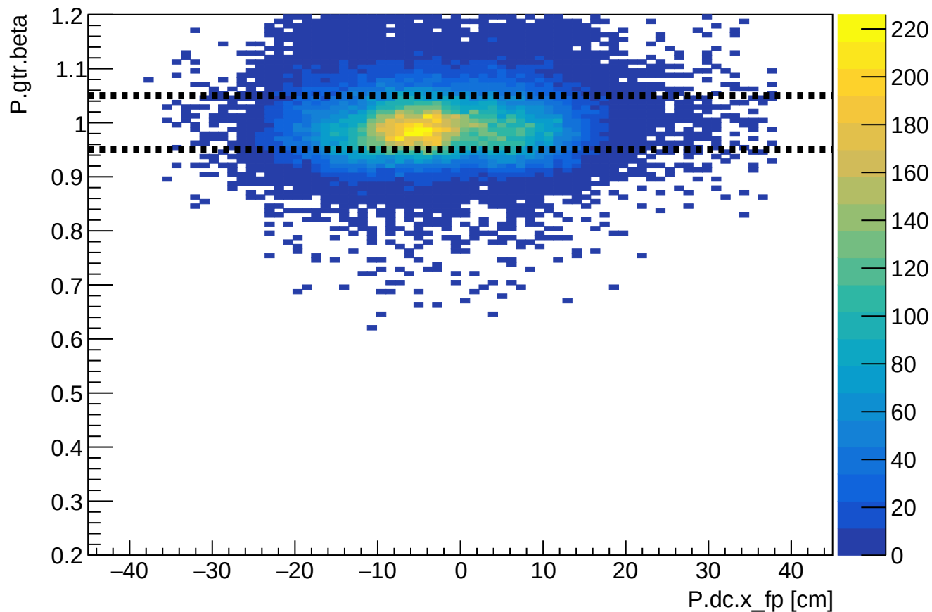
Phase 2 run 28108: SHMS beta vs SHMS xfp
