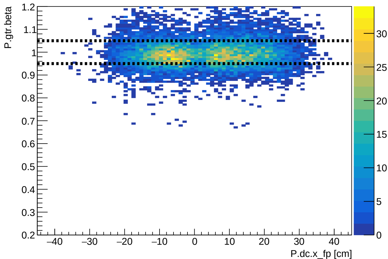
Phase 2 run 27888: SHMS beta vs SHMS xfp
