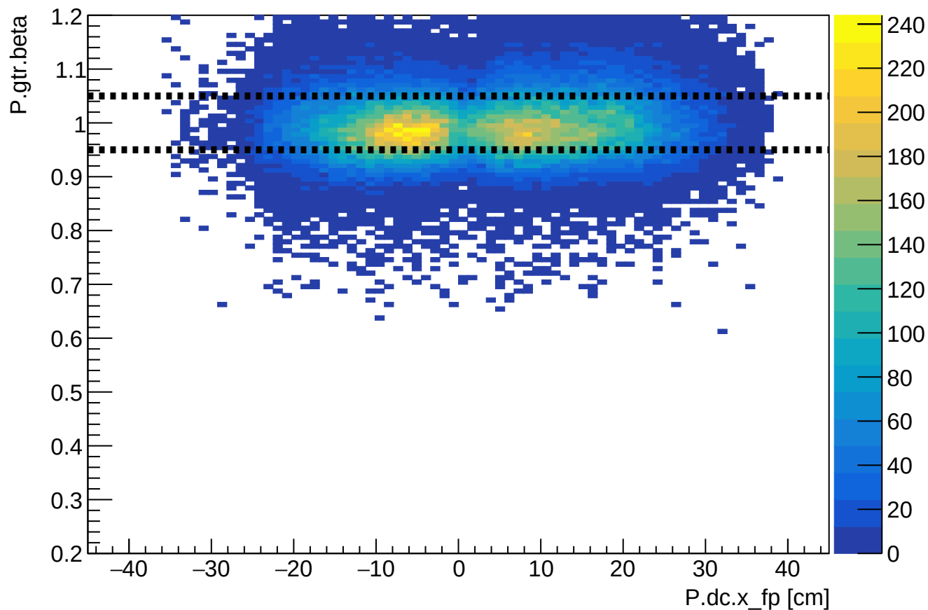
Phase 2 run 28203: SHMS beta vs SHMS xfp
