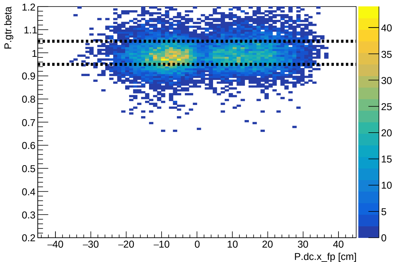
Phase 2 run 27172: SHMS beta vs SHMS xfp
