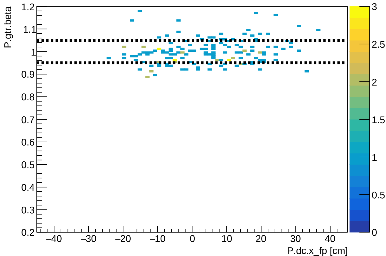
Phase 2 run 27320: SHMS beta vs SHMS xfp
