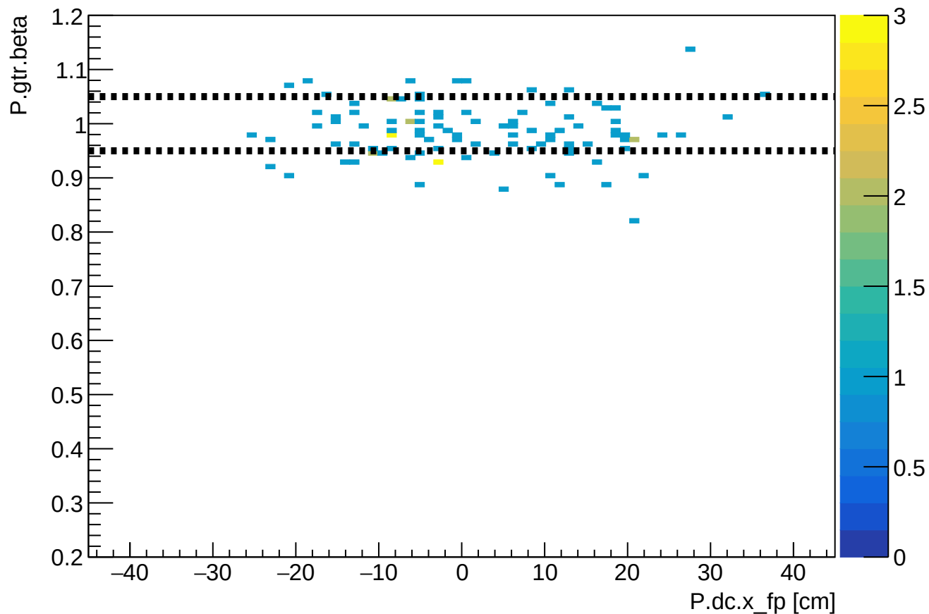
Phase 2 run 27234: SHMS beta vs SHMS xfp
