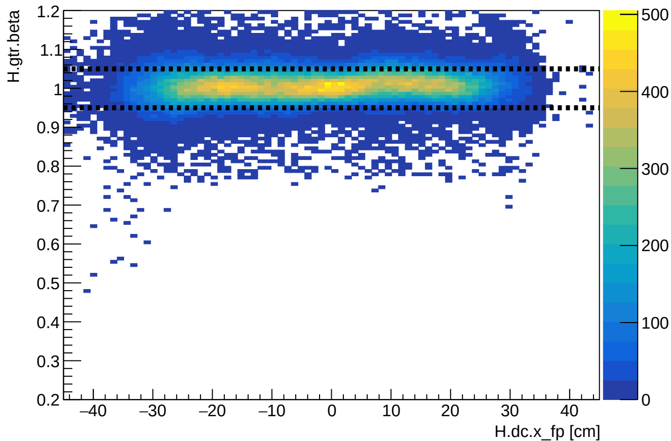
Phase 2 run 28267: HMS beta vs HMS xfp
