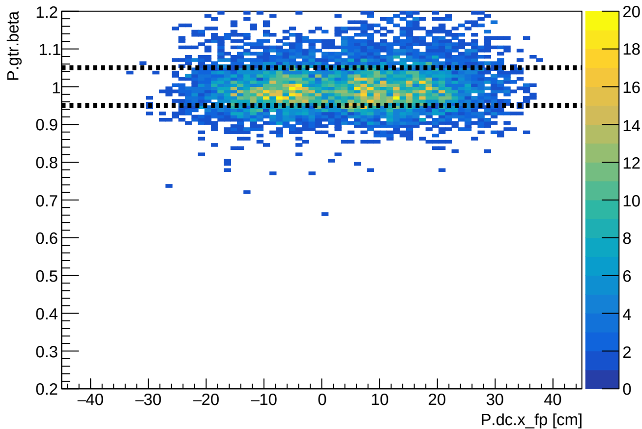
Phase 2 run 28348: SHMS beta vs SHMS xfp
