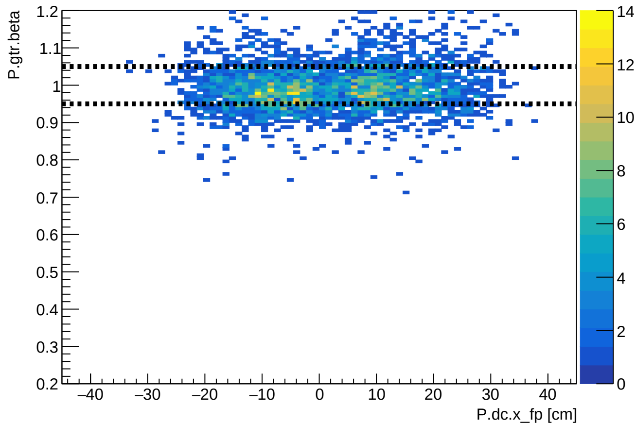
Phase 2 run 27279: SHMS beta vs SHMS xfp
