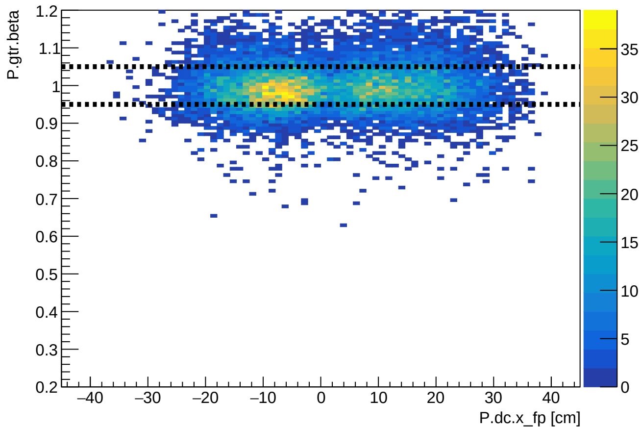
Phase 2 run 27144: SHMS beta vs SHMS xfp
