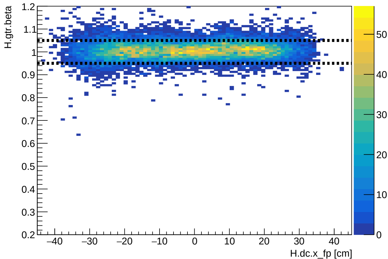
Phase 2 run 27165: HMS beta vs HMS xfp
