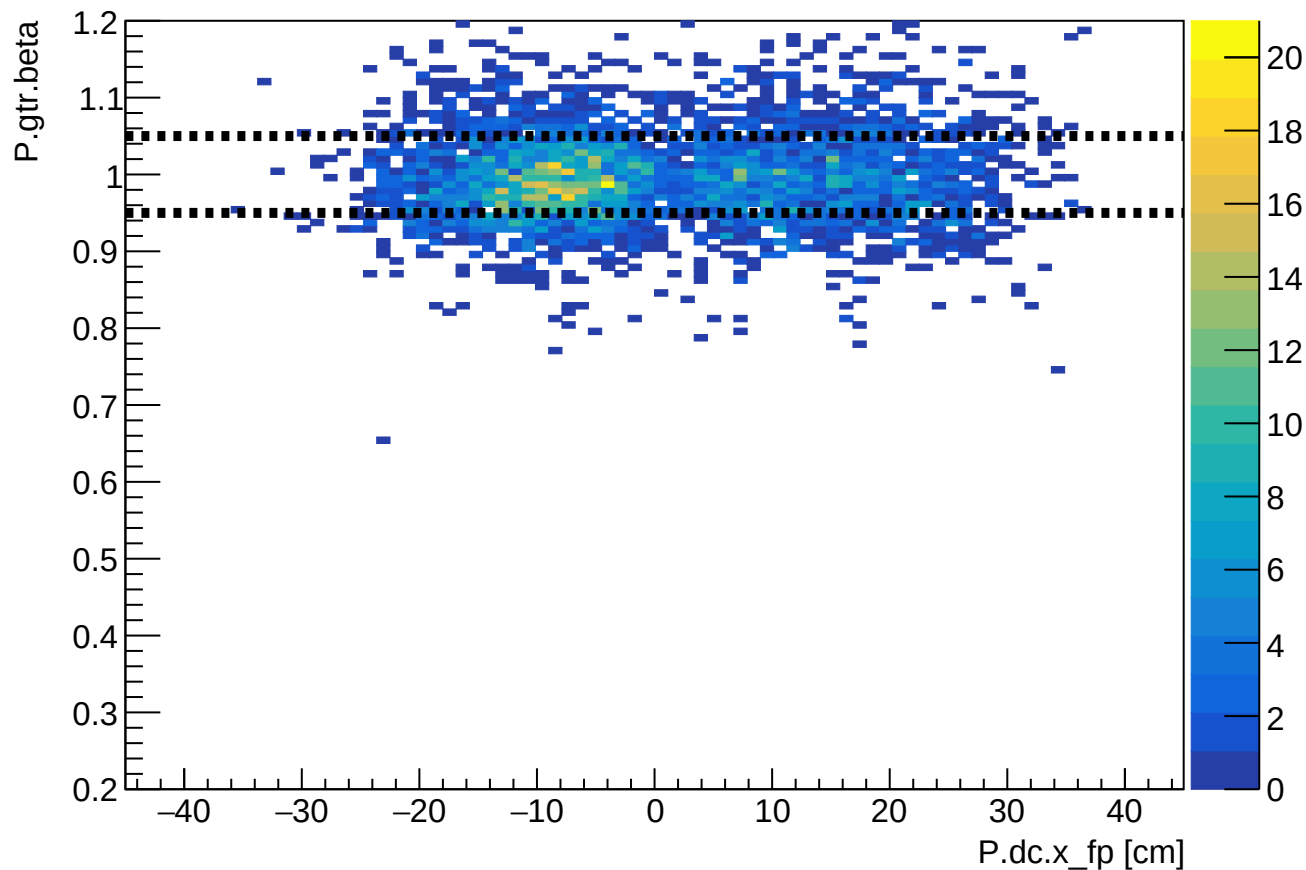
Phase 2 run 27150: SHMS beta vs SHMS xfp
