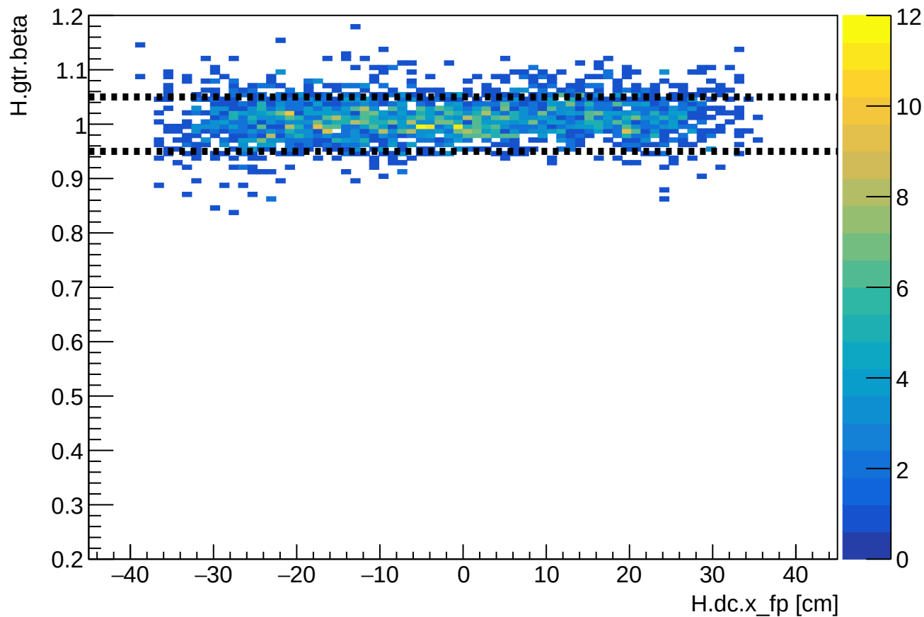
Phase 2 run 28365: HMS beta vs HMS xfp
