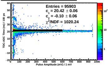
TDC-ADC Time vs. Pulse Amp Plane 1y Side neg Paddle 5
