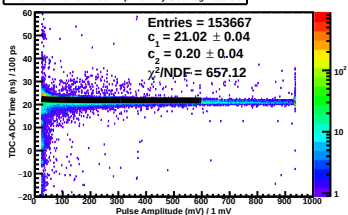
TDC-ADC Time vs. Pulse Amp Plane 1y Side neg Paddle 9
