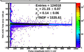
TDC-ADC Time vs. Pulse Amp Plane 1y Side neg Paddle 10
