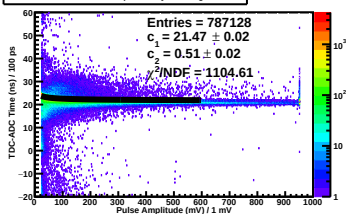
TDC-ADC Time vs. Pulse Amp Plane 1y Side neg Paddle 6
