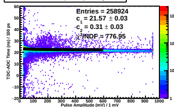
TDC-ADC Time vs. Pulse Amp Plane 1y Side neg Paddle 8
