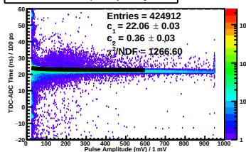
TDC-ADC Time vs. Pulse Amp Plane 1y Side neg Paddle 7
