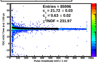
TDC-ADC Time vs. Pulse Amp Plane 1y Side pos Paddle 10
