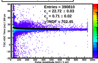
TDC-ADC Time vs. Pulse Amp Plane 1y Side pos Paddle 7
