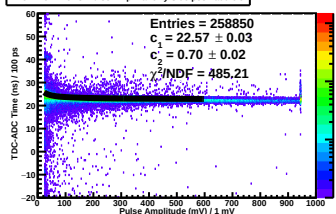
TDC-ADC Time vs. Pulse Amp Plane 1y Side pos Paddle 8
