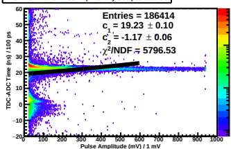
TDC-ADC Time vs. Pulse Amp Plane 1y Side pos Paddle 9
