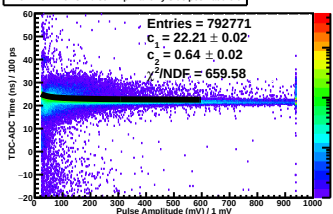
TDC-ADC Time vs. Pulse Amp Plane 1y Side pos Paddle 6
