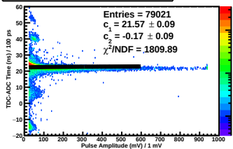
TDC-ADC Time vs. Pulse Amp Plane 1y Side pos Paddle 5
