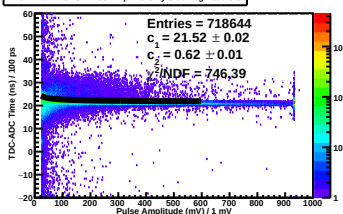
TDC-ADC Time vs. Pulse Amp Plane 2y Side neg Paddle 6
