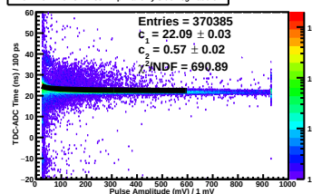
TDC-ADC Time vs. Pulse Amp Plane 2y Side neg Paddle 7
