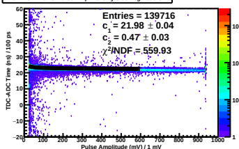
TDC-ADC Time vs. Pulse Amp Plane 2y Side neg Paddle 10
