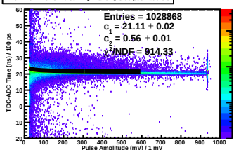
TDC-ADC Time vs. Pulse Amp Plane 2y Side pos Paddle 5
