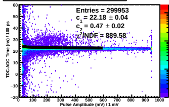
TDC-ADC Time vs. Pulse Amp Plane 2y Side pos Paddle 7
