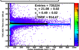
TDC-ADC Time vs. Pulse Amp Plane 2y Side pos Paddle 6
