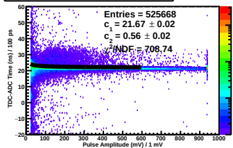
TDC-ADC Time vs. Pulse Amp Plane 2y Side pos Paddle 8
