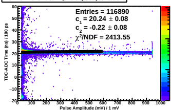
TDC-ADC Time vs. Pulse Amp Plane 2y Side pos Paddle 10
