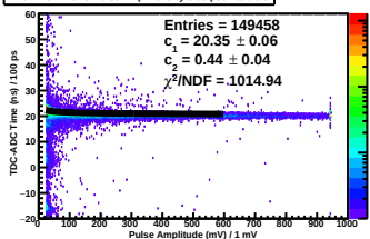
TDC-ADC Time vs. Pulse Amp Plane 2y Side pos Paddle 9
