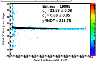
TDC-ADC Time vs. Pulse Amp Plane 1y Side neg Paddle 10
