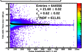
TDC-ADC Time vs. Pulse Amp Plane 1y Side neg Paddle 6
