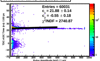
TDC-ADC Time vs. Pulse Amp Plane 1y Side pos Paddle 9
