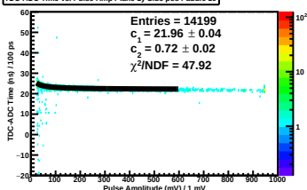
TDC-ADC Time vs. Pulse Amp Plane 1y Side pos Paddle 10
