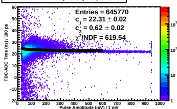
TDC-ADC Time vs. Pulse Amp Plane 1y Side pos Paddle 6
