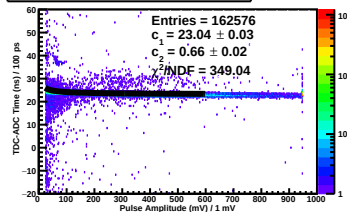
TDC-ADC Time vs. Pulse Amp Plane 1y Side pos Paddle 7
