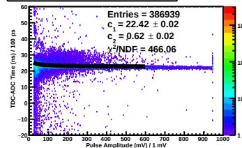
TDC-ADC Time vs. Pulse Amp Plane 1y Side pos Paddle 8
