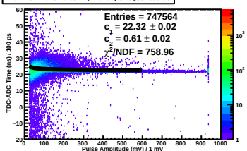
TDC-ADC Time vs. Pulse Amp Plane 1y Side pos Paddle 5
