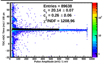
TDC-ADC Time vs. Pulse Amp Plane 2y Side neg Paddle 5
