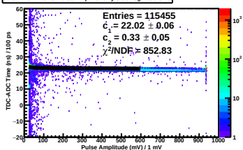
TDC-ADC Time vs. Pulse Amp Plane 2y Side neg Paddle 10
