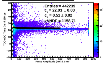
TDC-ADC Time vs. Pulse Amp Plane 2y Side neg Paddle 8
