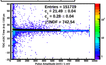
TDC-ADC Time vs. Pulse Amp Plane 2y Side neg Paddle 9
