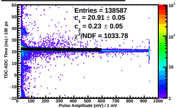
TDC-ADC Time vs. Pulse Amp Plane 2y Side neg Paddle 6
