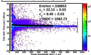
TDC-ADC Time vs. Pulse Amp Plane 2y Side neg Paddle 7
