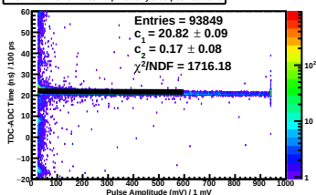
TDC-ADC Time vs. Pulse Amp Plane 2y Side pos Paddle 10
