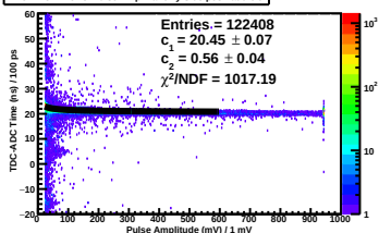
TDC-ADC Time vs. Pulse Amp Plane 2y Side pos Paddle 9
