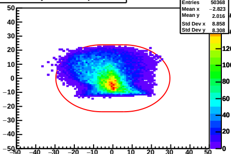
Tracks Projected to Dipole Exit
