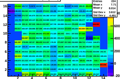
Calib. Gains: Shower (Layer2)
