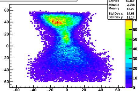
Tracks Projected to Calorimeter
