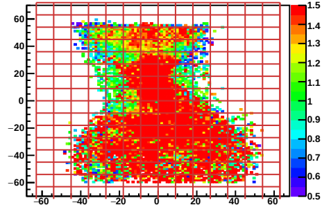
Calibrated E/p at calorimeter
