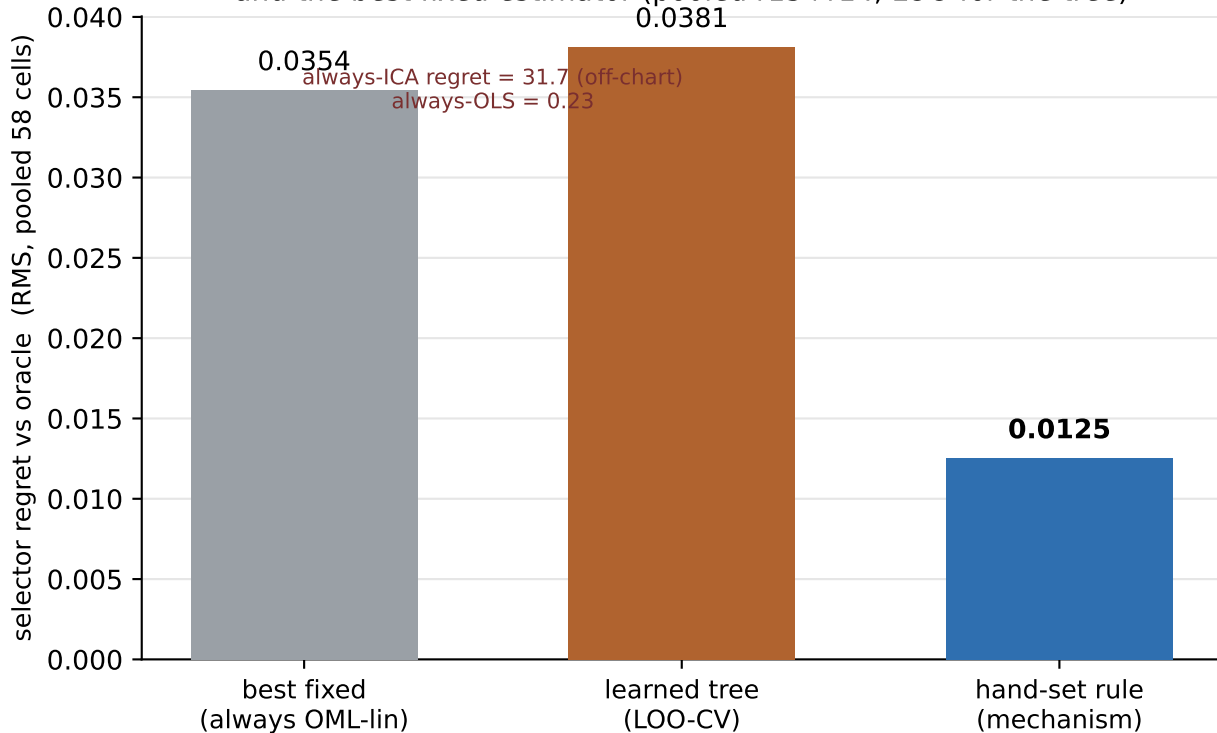
WS4 closure: the interpretable rule beats a learned tree and the best fixed estimator (pooled r13+r14, LOO for the tree)
